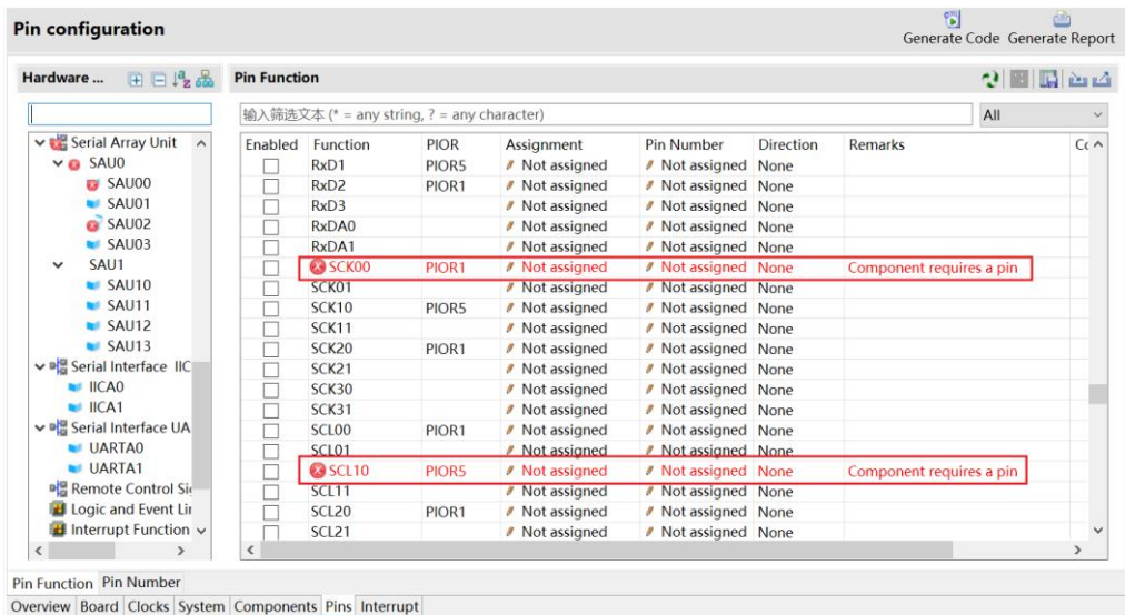
Figure 5-8 Incorrect pin assignment in [Pins] page
