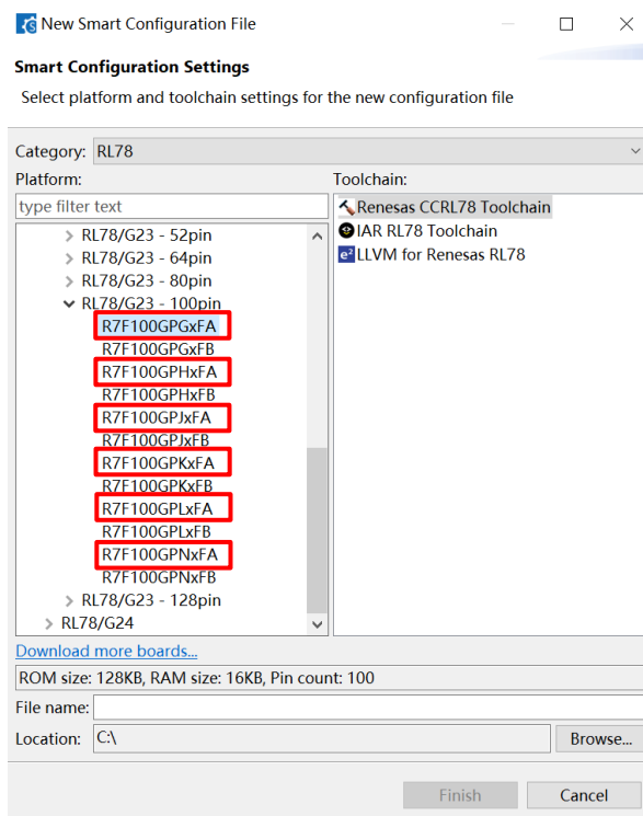
Figure 5-10 The chips which are 100-pin plastic LQFP
