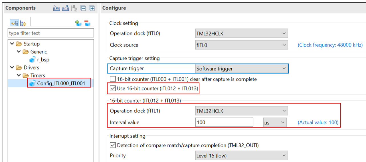
Figure 3-2 Use 16-bit count mode with channel 2 and 3 in 16 bit capture mode
