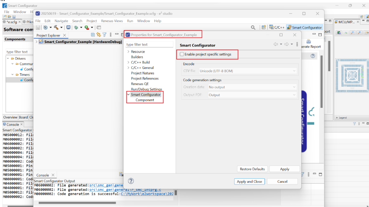
Figure 2-4 Smart Configurator preferences setting at project level
