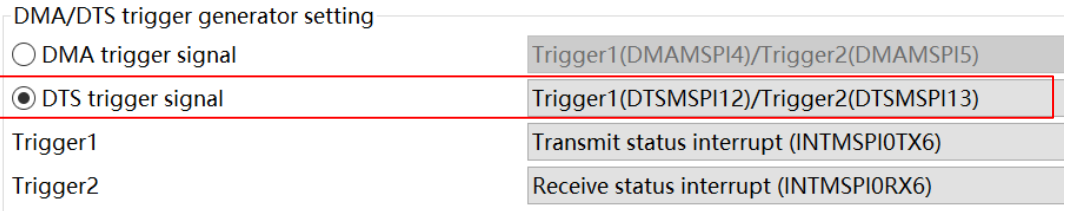
Figure 6-4. "Trigger1(DTSMSPi12)/Trigger2(DTSMSPi13)" selected after reloading in Smart Configurator for RH850 V1.6.0
