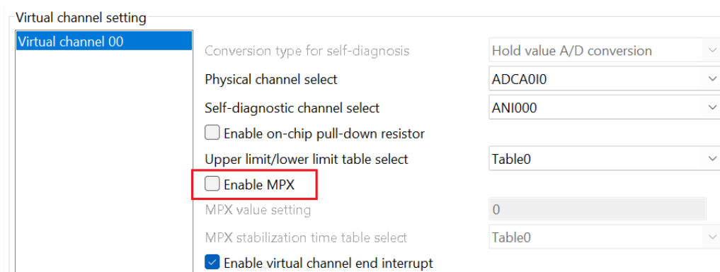
Figure 3-1 Enable MPX checkbox in A/D Converter
