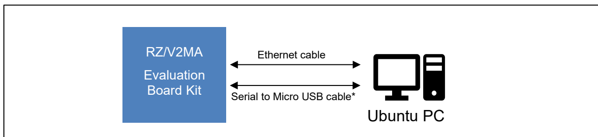
Figure 3-1 Hardware Configuration
