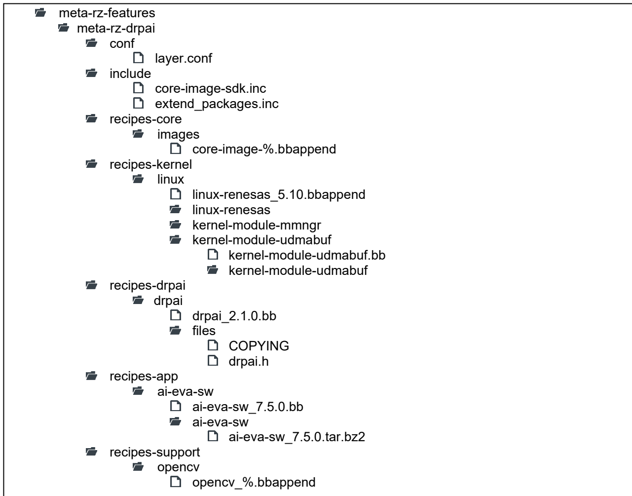
Figure 3-1 Directory Structure of Recipe
