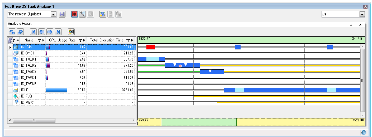
Figure 7-2 Image of Realtime OS Task Analyzer
