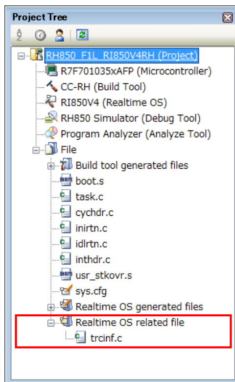
figure 7-3 Project Tree
