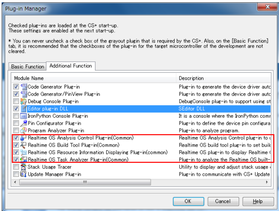
figure 8-8 Plug-in Manager
