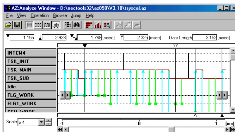
figure 7-1 Image of AZ850V4
