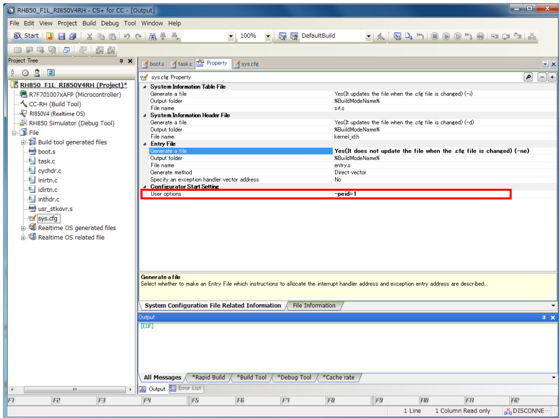
figure 8-14 Set the option about entry file
