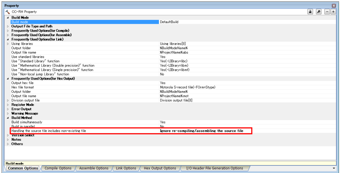
figure 7-4 Property of CC-RH
