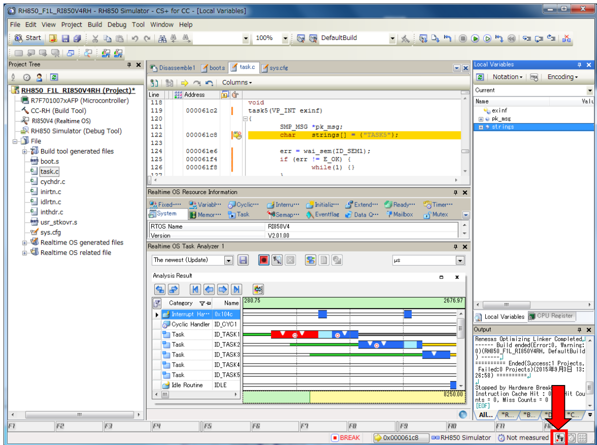
figure 8-13 Enable The Trace Function of The Debugger
