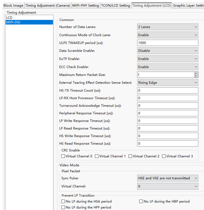
Figure 1-2 MIPI-DSI Setting
