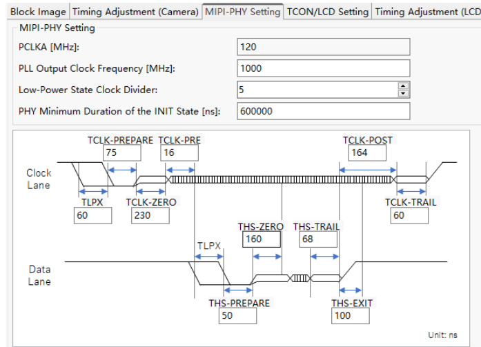
Figure 1-1 MIPI-PHY Setting
