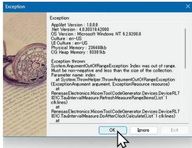
Figure 3-3 The error message
