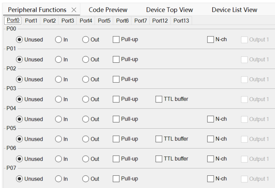
Figure 3-2 Code Generator view (after)
