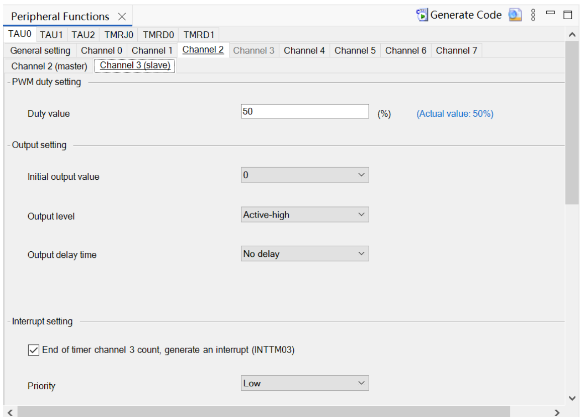
Figure 6-13 The scroll bar exists
