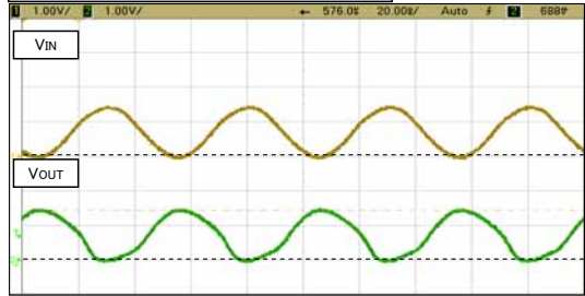
Typical sample at V cc =5V,25deg.C Vertical: 1V/div., Horizontal: 20ns/div. Broken line: GND
