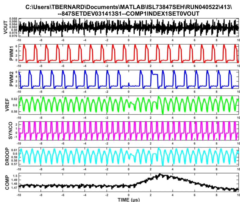
Figure 4. SET, LET86, f_{SW} = 1\text{MHz} , trigger V_{OUT} \pm 20\text{mV}
