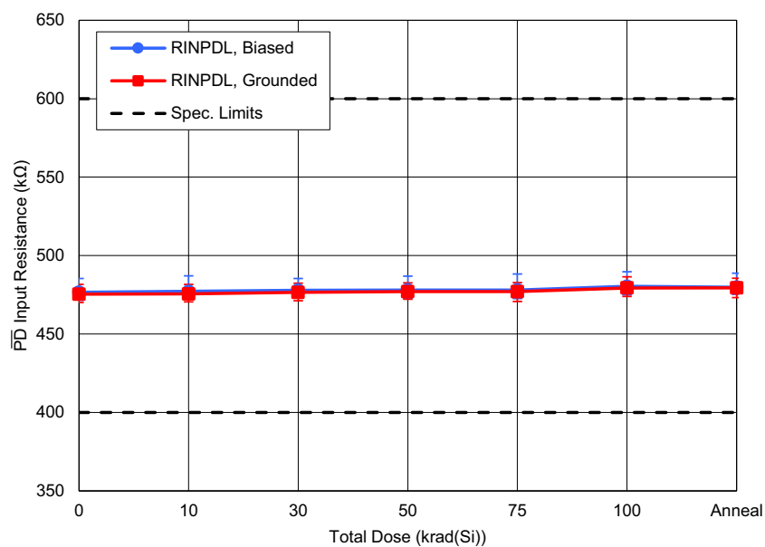
Figure 52. ISL73148SEH \overline{PD} input resistance ( R_{INPDL} ) as a function of LDR irradiation and anneal for biased and grounded configurations. The error bars (if visible) represent the minimum and maximum measured values. The datasheet limits are a minimum of 400k\Omega and a maximum of 600k\Omega .
