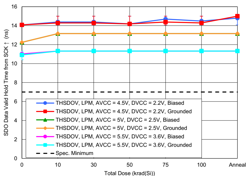
Figure 70. ISL73148SEH SDO Data Valid Hold Time from SCK ↑ ( t_{HSDOV} ) in low power mode with C_L = 10\text{pF} and with AV_{CC} = 4.5\text{V} and DV_{CC} = 2.2\text{V} or AV_{CC} = 5\text{V} and DV_{CC} = 2.5\text{V} or AV_{CC} = 5.5\text{V} and DV_{CC} = 3.6\text{V} as a function of LDR irradiation and anneal for biased and grounded configurations. The error bars (if visible) represent the minimum and maximum measured values. The datasheet limit is a minimum of 7ns.
