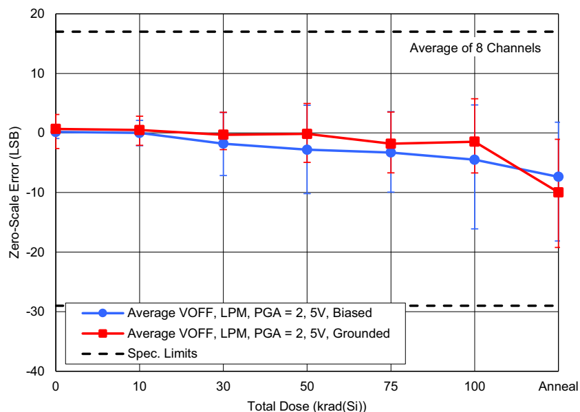
Figure 9. ISL73148SEH average zero-scale error (V OFF ) in low power mode with AV CC = 5V and PGA Gain = 2 as a function of LDR irradiation and anneal for biased and grounded configurations. The error bars (if visible) represent the minimum and maximum measured values across all channels. The datasheet limits are a minimum of -29LSB and a maximum of 17LSB.
