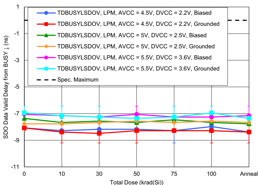
Figure 66. ISL73148SEH SDO Data Valid Delay from BUSY ↓ ( t_{\text{DBUSYLSDOV}} ) in low power mode with C_L = 10\text{pF} and with \text{AV}_{\text{CC}} = 4.5\text{V} and \text{DV}_{\text{CC}} = 2.2\text{V} or \text{AV}_{\text{CC}} = 5\text{V} and \text{DV}_{\text{CC}} = 2.5\text{V} or \text{AV}_{\text{CC}} = 5.5\text{V} and \text{DV}_{\text{CC}} = 3.6\text{V} as a function of LDR irradiation and anneal for biased and grounded configurations. The error bars (if visible) represent the minimum and maximum measured values. The datasheet limit is a maximum of 0ns.
