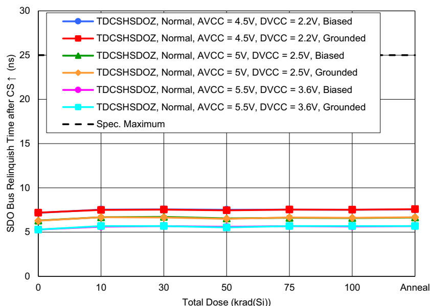
Figure 73. ISL73148SEH SDO Bus Relinquish Time after \overline{CS} \uparrow ( t_{DCSHSDOZ} ) in normal operating mode with C_L = 10\text{pF} and with AV_{CC} = 4.5\text{V} and DV_{CC} = 2.2\text{V} or AV_{CC} = 5\text{V} and DV_{CC} = 2.5\text{V} or AV_{CC} = 5.5\text{V} and DV_{CC} = 3.6\text{V} as a function of LDR irradiation and anneal for biased and grounded configurations. The error bars (if visible) represent the minimum and maximum measured values. The datasheet limit is a maximum of 25ns.
