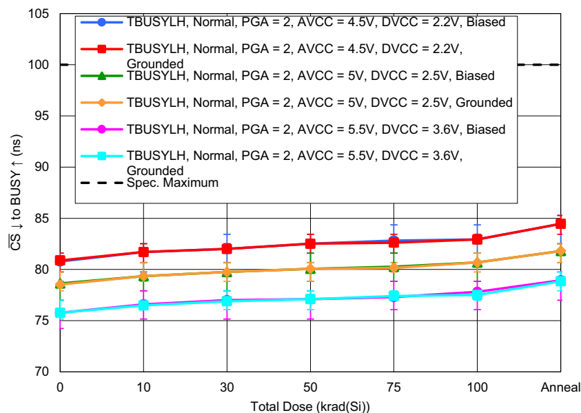
Figure 61. ISL73148SEH \overline{CS}_{\downarrow} to BUSY_{\uparrow} ( t_{BUSYLH} ) in normal operating mode with PGA Gain = 2, C_L = 10pF , and with AV_{CC} = 4.5V and DV_{CC} = 2.2V or AV_{CC} = 5V and DV_{CC} = 2.5V or AV_{CC} = 5.5V and DV_{CC} = 3.6V as a function of LDR irradiation and anneal for biased and grounded configurations. The error bars (if visible) represent the minimum and maximum measured values. The datasheet limit is a maximum of 100ns.
