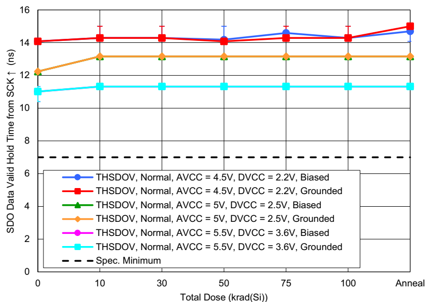
Figure 69. ISL73148SEH SDO Data Valid Hold Time from SCK ↑ ( t_{HSDOV} ) in normal operating mode with C_L = 10\text{pF} and with AV_{CC} = 4.5\text{V} and DV_{CC} = 2.2\text{V} or AV_{CC} = 5\text{V} and DV_{CC} = 2.5\text{V} or AV_{CC} = 5.5\text{V} and DV_{CC} = 3.6\text{V} as a function of LDR irradiation and anneal for biased and grounded configurations. The error bars (if visible) represent the minimum and maximum measured values. The datasheet limit is a minimum of 7ns.
