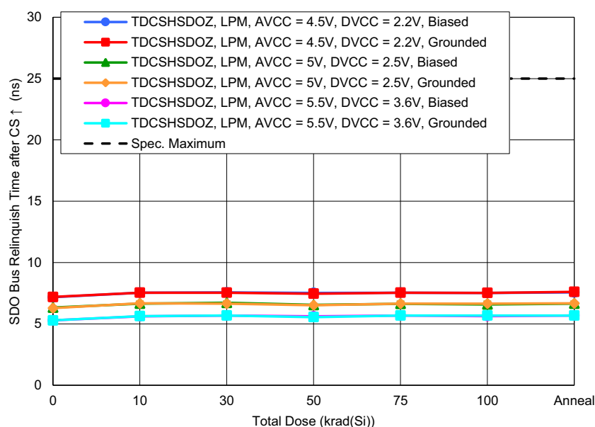
Figure 74. ISL73148SEH SDO Bus Relinquish Time after \overline{CS} \uparrow ( t_{DCSHSDOZ} ) in low power mode with C_L = 10\text{pF} and with AV_{CC} = 4.5\text{V} and DV_{CC} = 2.2\text{V} or AV_{CC} = 5\text{V} and DV_{CC} = 2.5\text{V} or AV_{CC} = 5.5\text{V} and DV_{CC} = 3.6\text{V} as a function of LDR irradiation and anneal for biased and grounded configurations. The error bars (if visible) represent the minimum and maximum measured values. The datasheet limit is a maximum of 25ns.
