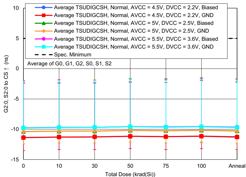
Figure 75. ISL73148SEH average G2:0, S2:0 to CS↑ ( t_{SUDIGCSH} ) in normal operating mode with AV_{CC} = 4.5V and DV_{CC} = 2.2V or AV_{CC} = 5V and DV_{CC} = 2.5V or AV_{CC} = 5.5V and DV_{CC} = 3.6V as a function of LDR irradiation and anneal for biased and grounded configurations. The error bars (if visible) represent the minimum and maximum measured values across all pins. The datasheet limit is a minimum of 5ns.
