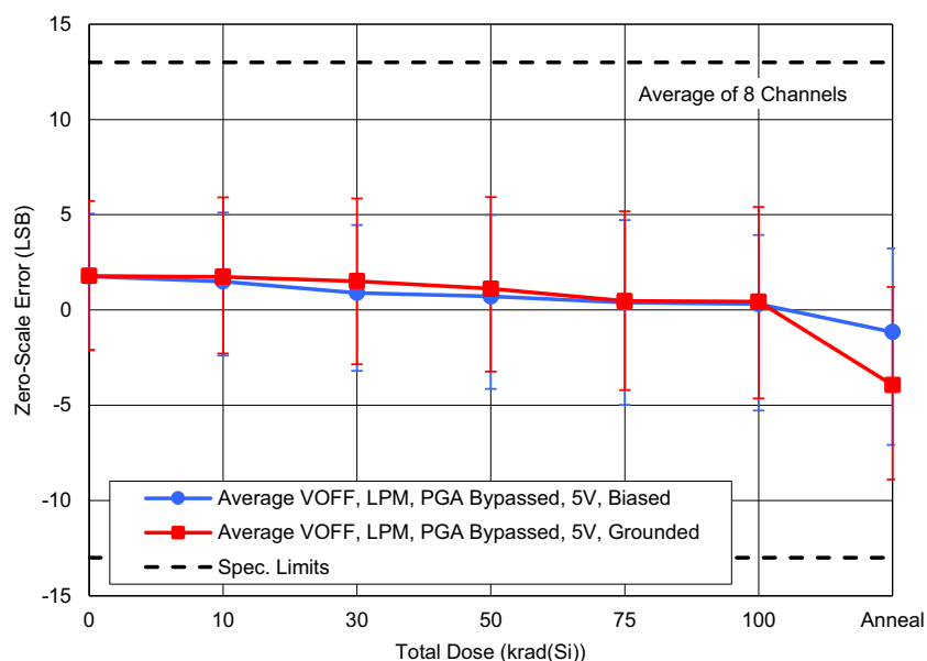
Figure 10. ISL73148SEH average zero-scale error (V OFF ) in low power mode with AV CC = 5V and PGA bypassed as a function of LDR irradiation and anneal for biased and grounded configurations. The error bars (if visible) represent the minimum and maximum measured values across all channels. The datasheet limits are a minimum of -13LSB and a maximum of 13LSB.
