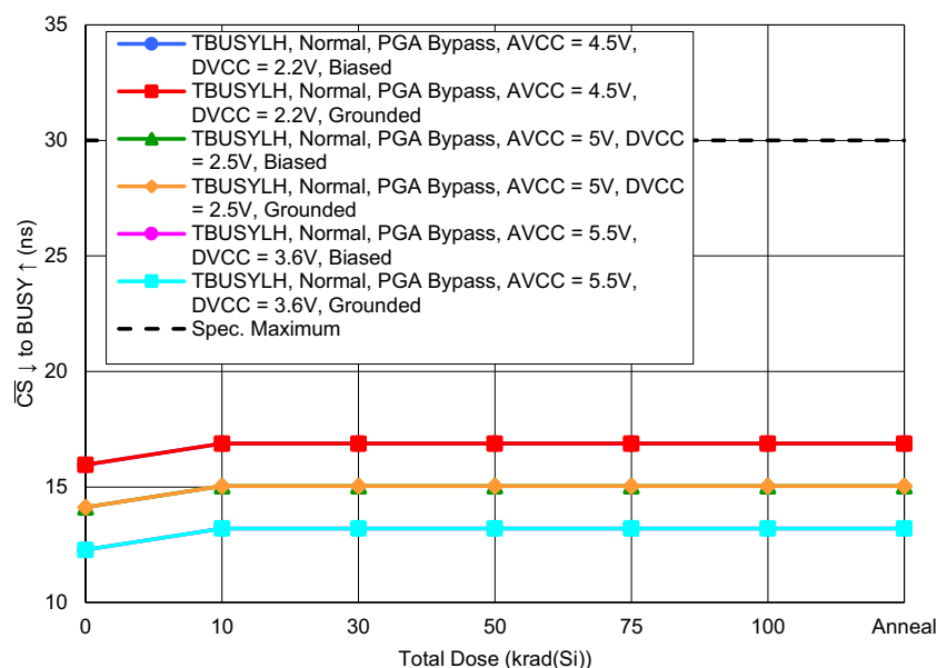
Figure 62. ISL73148SEH \overline{CS}_{\downarrow} to BUSY_{\uparrow} ( t_{BUSYLH} ) in normal operating mode with PGA bypassed, C_L = 10pF and with AV_{CC} = 4.5V and DV_{CC} = 2.2V or AV_{CC} = 5V and DV_{CC} = 2.5V or AV_{CC} = 5.5V and DV_{CC} = 3.6V as a function of LDR irradiation and anneal for biased and grounded configurations. The error bars (if visible) represent the minimum and maximum measured values. The datasheet limit is a maximum of 30ns.
