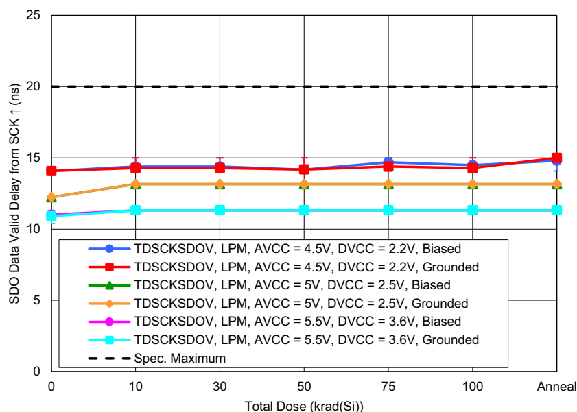
Figure 68. ISL73148SEH SDO Data Valid Delay from SCK ↑ ( t_{DSCKSDOV} ) in low power mode with C_L = 10\text{pF} , and with AV_{CC} = 4.5\text{V} and DV_{CC} = 2.2\text{V} or AV_{CC} = 5\text{V} and DV_{CC} = 2.5\text{V} or AV_{CC} = 5.5\text{V} and DV_{CC} = 3.6\text{V} as a function of LDR irradiation and anneal for biased and grounded configurations. The error bars (if visible) represent the minimum and maximum measured values. The datasheet limit is a maximum of 20ns.
