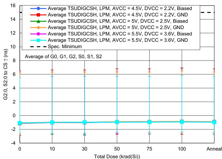
Figure 76. ISL73148SEH average G2:0, S2:0 to CS↑ ( t_{SUDIGCSH} ) in low power mode with AV_{CC} = 4.5V and DV_{CC} = 2.2V or AV_{CC} = 5V and DV_{CC} = 2.5V or AV_{CC} = 5.5V and DV_{CC} = 3.6V as a function of LDR irradiation and anneal for biased and grounded configurations. The error bars (if visible) represent the minimum and maximum measured values across all pins. The datasheet limit is a minimum of 15ns.
