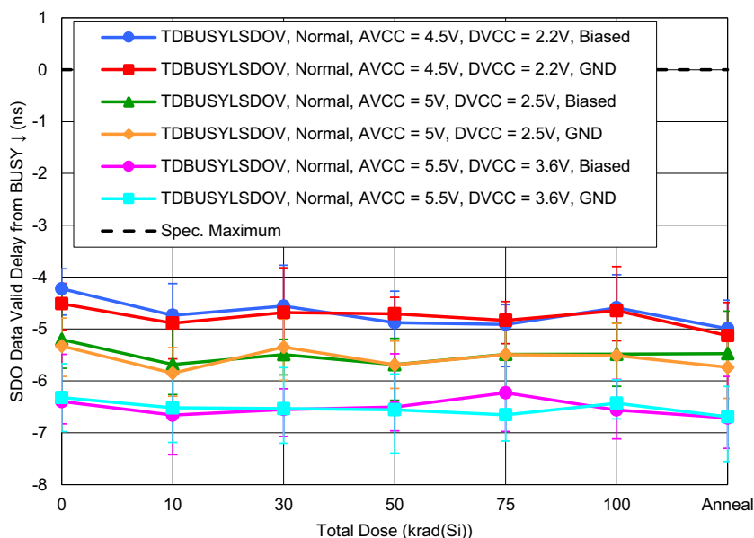
Figure 65. ISL73148SEH SDO Data Valid Delay from BUSY ↓ ( t_{\text{DBUSYLSDOV}} ) in normal operating mode with C_L = 10\text{pF} and with \text{AV}_{\text{CC}} = 4.5\text{V} and \text{DV}_{\text{CC}} = 2.2\text{V} or \text{AV}_{\text{CC}} = 5\text{V} and \text{DV}_{\text{CC}} = 2.5\text{V} or \text{AV}_{\text{CC}} = 5.5\text{V} and \text{DV}_{\text{CC}} = 3.6\text{V} as a function of LDR irradiation and anneal for biased and grounded configurations. The error bars (if visible) represent the minimum and maximum measured values. The datasheet limit is a maximum of 0ns.
