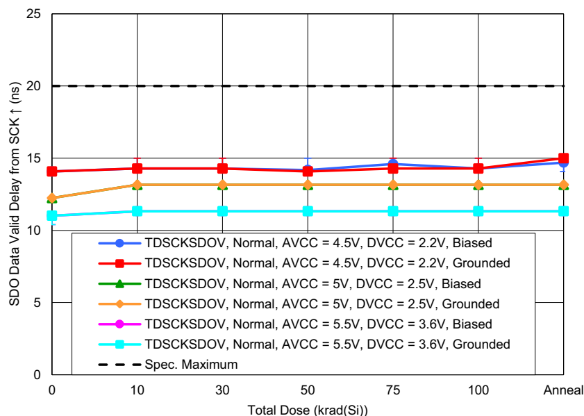
Figure 67. ISL73148SEH SDO Data Valid Delay from SCK ↑ ( t_{DSCKSDOV} ) in normal operating mode with C_L = 10\text{pF} , and with AV_{CC} = 4.5\text{V} and DV_{CC} = 2.2\text{V} or AV_{CC} = 5\text{V} and DV_{CC} = 2.5\text{V} or AV_{CC} = 5.5\text{V} and DV_{CC} = 3.6\text{V} as a function of LDR irradiation and anneal for biased and grounded configurations. The error bars (if visible) represent the minimum and maximum measured values. The datasheet limit is a maximum of 20ns.
