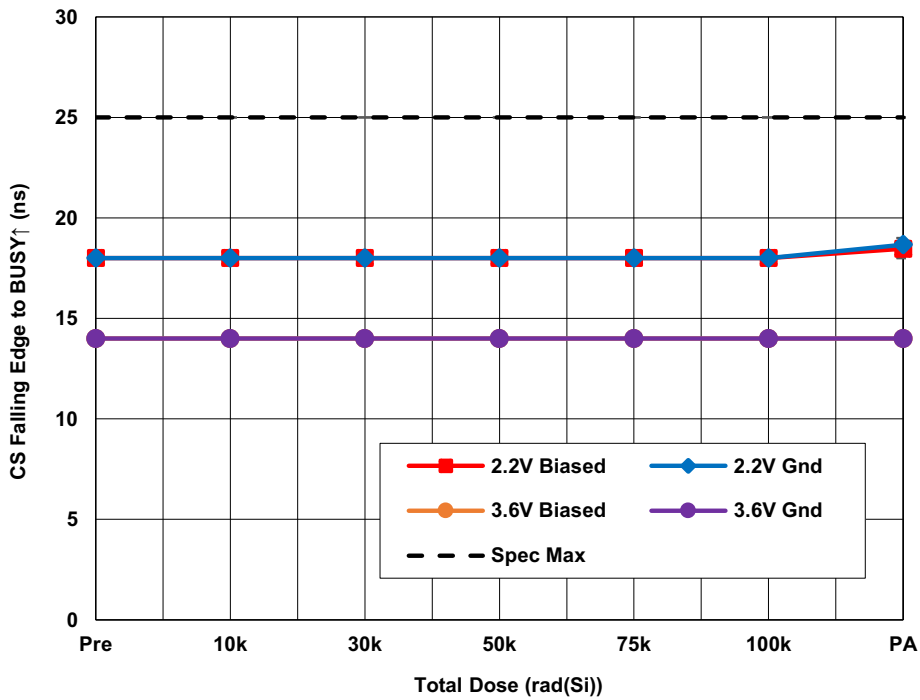
Figure 28. ISL73141SEHMF7 average \overline{CS} falling edge to BUSY rising edge ( t_{BUSYLH} ) with AV_{CC} = 4.5V , DV_{CC} = 2.2V and AV_{CC} = 5.5V , DV_{CC} = 3.6V , REF = 4.096V , f_{SAMP} = 1Msps , A_{IN} = -1dbFS and C_L = 10pF as a function of LDR irradiation and anneal. The error bars represent the minimum and maximum measured values. The datasheet limit is 25ns maximum.
