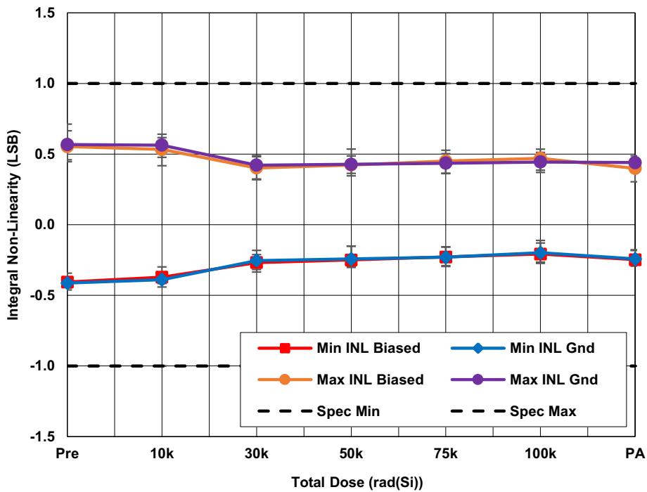
Figure 4. ISL73141SEHMF7 average minimum and maximum integral non-linearity (INL) with AV_{CC} = 5V , DV_{CC} = 2.5V , REF = 4.096V , f_{SAMP} = 1Mpsps , and A_{IN} = full-scale sine wave as a function of LDR irradiation and anneal. The error bars represent the minimum and maximum measured values. The datasheet limits are -1 LSB minimum and 1 LSB maximum.
