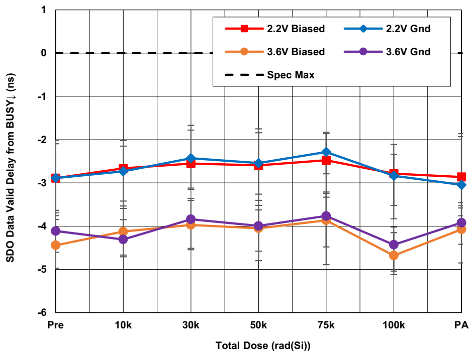
Figure 29. ISL73141SEHMF7 average SDO data valid delay from BUSY falling edge ( t_{DBUSYLSDOV} ) with AV_{CC} = 4.5V , DV_{CC} = 2.2V and AV_{CC} = 5.5V , DV_{CC} = 3.6V , REF = 4.096V , f_{SAMP} = 1Msps , A_{IN} = -1dbFS and C_L = 10pF as a function of LDR irradiation and anneal. The error bars represent the minimum and maximum measured values. The datasheet limit is 0ns maximum.
