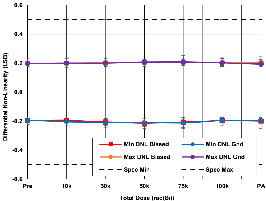
Figure 5. ISL73141SEHMF7 average minimum and maximum differential non-linearity (DNL) with AV_{CC} = 5V , DV_{CC} = 2.5V , REF = 4.096V , f_{SAMP} = 1Mpsps , and A_{IN} = full-scale sine wave as a function of LDR irradiation and anneal. The error bars represent the minimum and maximum measured values. The datasheet limits are -0.5 LSB minimum and 0.5 LSB maximum.
