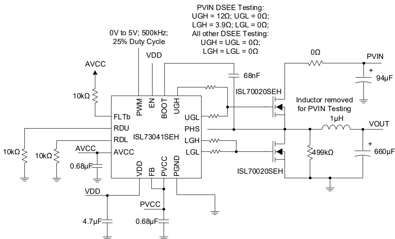
Figure 1. ISL73041SEH DSEE Test Board Schematic
