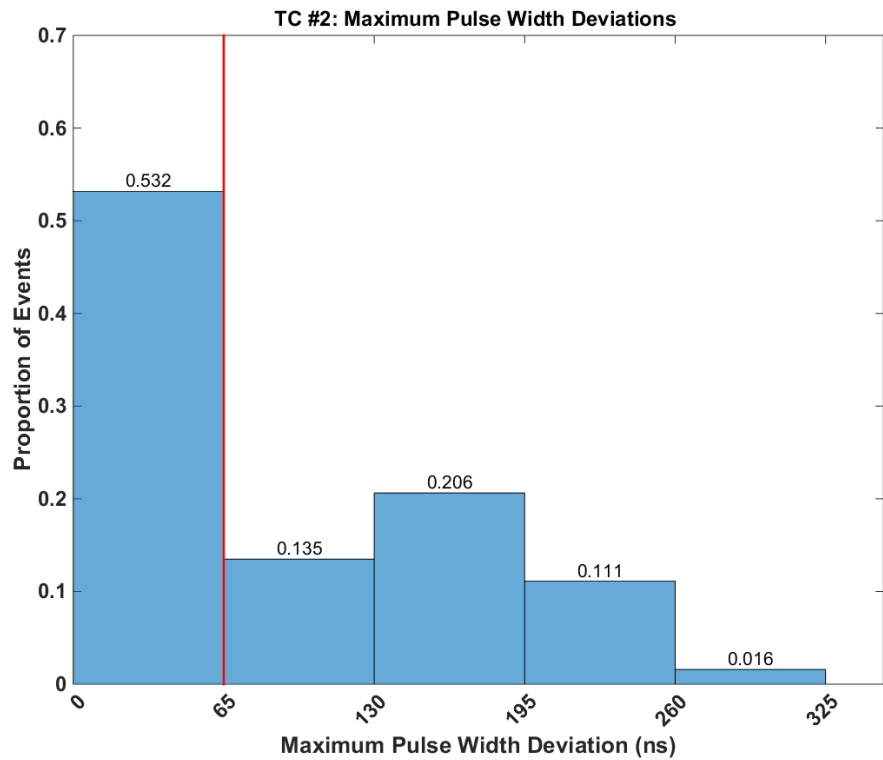
Figure 5. ISL73041SEH TC #2: Maximum Pulse Width Deviations
