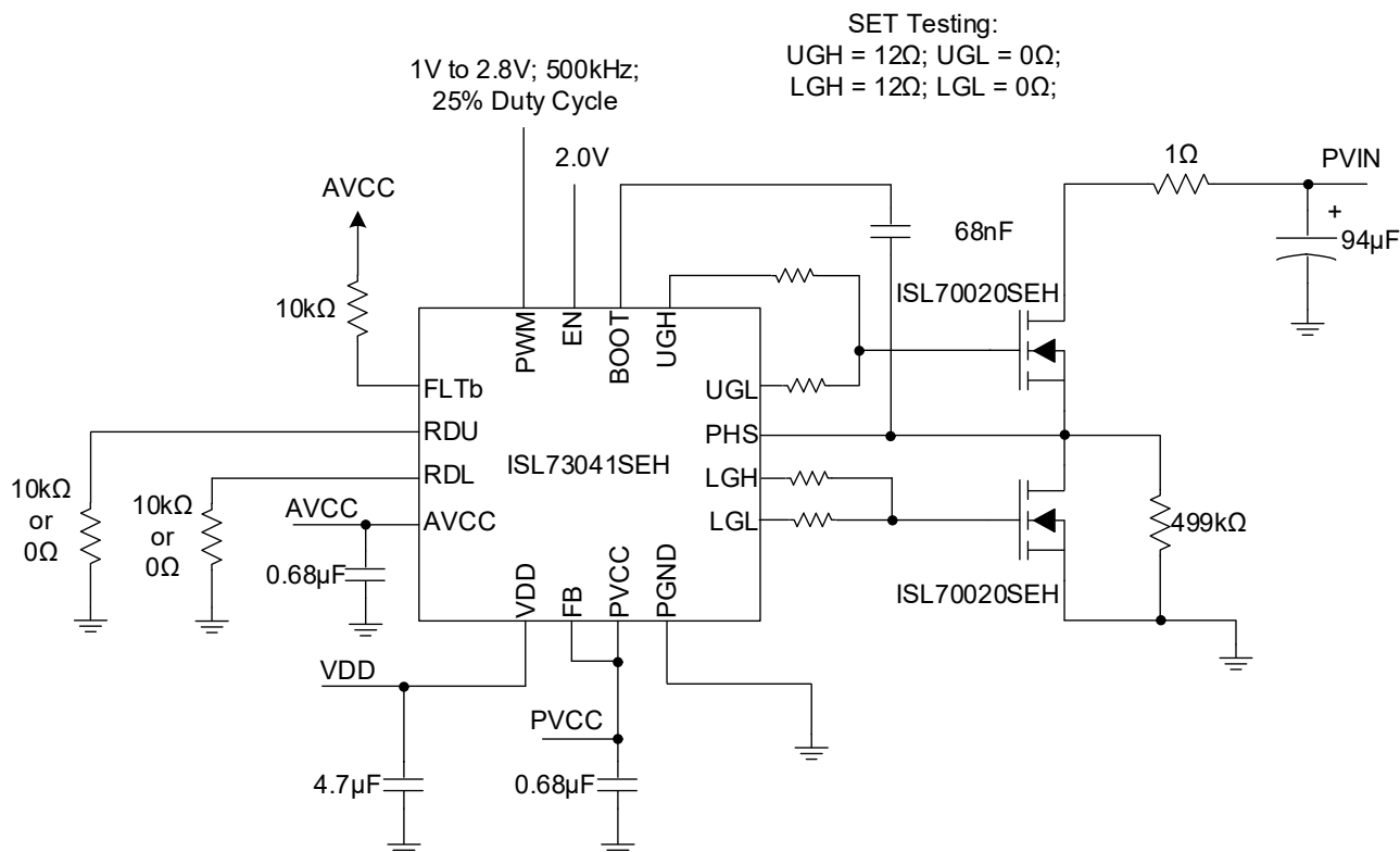
Figure 2. ISL73041SEH SET Test Board Schematic
