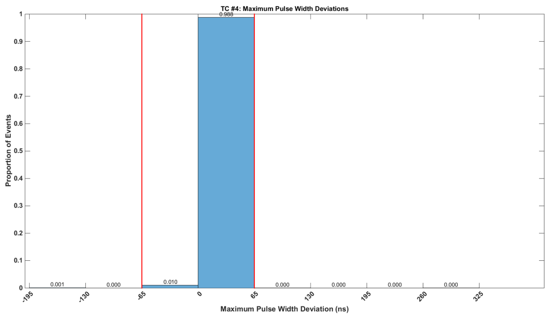
Figure 18. ISL73041SEH TC #4: Maximum Pulse Width Deviations
