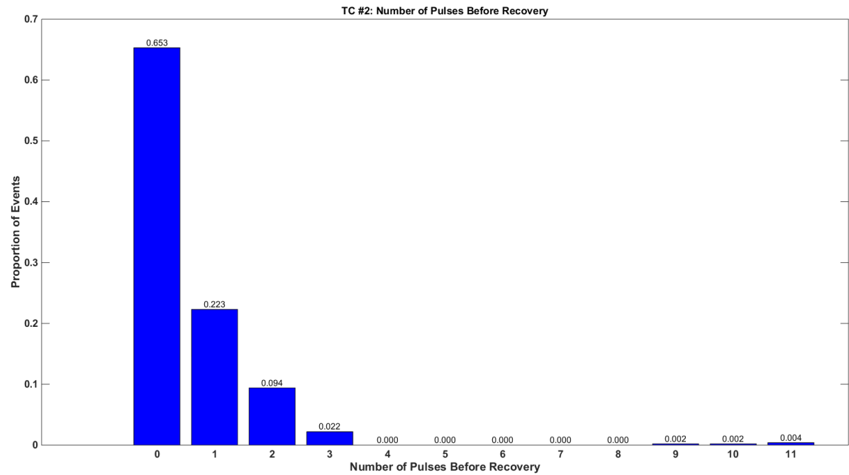
Figure 16. ISL73041SEH TC #2: Pulses Until Recovery
