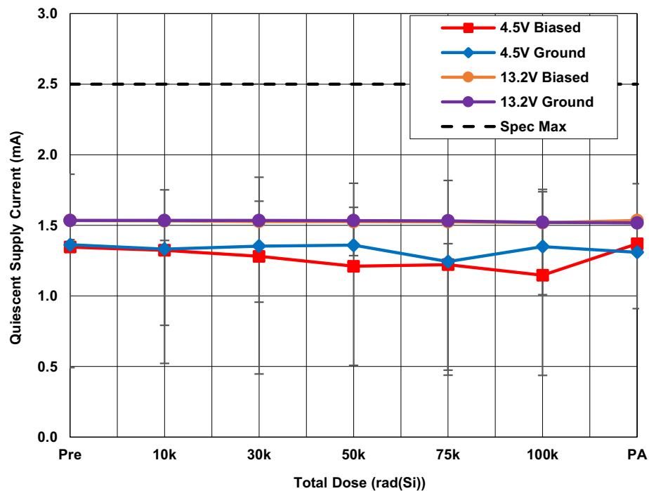
Figure 4. ISL73033SLHM average quiescent supply current ( I_{DDQ} ) with V_{DD} = 4.5V and 13.2V as a function of LDR irradiation and anneal. The error bars represent the minimum and maximum measured values. The datasheet limit is 2.5mA maximum.
