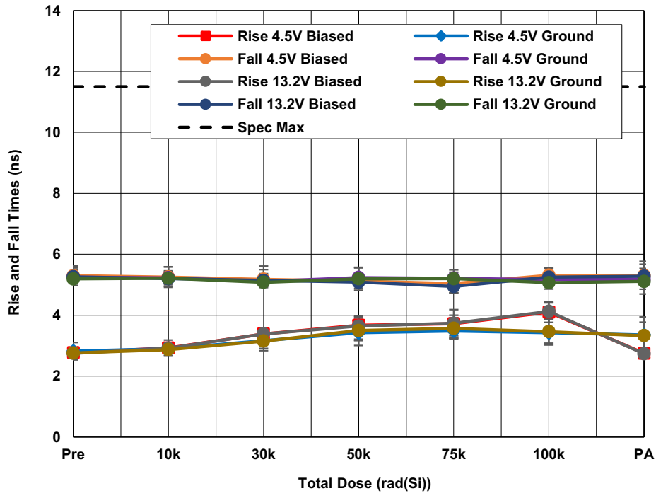
Figure 22. ISL73033SLHM average rise and fall times ( t_{\text{RISE}} , t_{\text{FALL}} ) with V_{\text{DD}} = 4.5\text{V} and 13.2\text{V} as a function of LDR irradiation and anneal. The error bars represent the minimum and maximum measured values. The datasheet limit is 11.5ns maximum.
