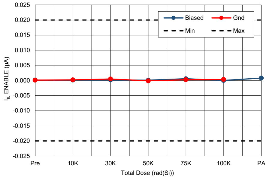
Figure 25. ISL73007SEH low enable current ( EN_{IL} ) with as a function of LDR irradiation and anneal for biased and grounded configurations. The error bars (if visible) represent the minimum and maximum measured values. The post-irradiation datasheet limits are -0.02\mu\text{A} minimum and 0.02\mu\text{A} maximum.
