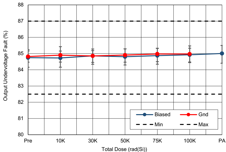
Figure 33. ISL73007SEH output undervoltage fault (UVflt) with PV_{IN} = 5V as a function of LDR irradiation and anneal for biased and grounded configurations. The error bars (if visible) represent the minimum and maximum measured values. The post-irradiation datasheet limits are 82.5% minimum and 87% maximum.
