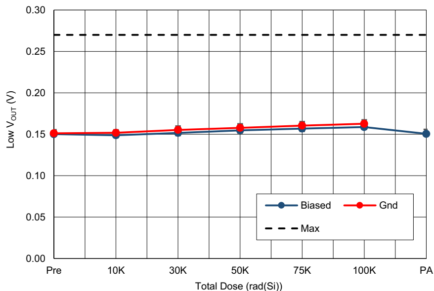
Figure 35. ISL73007SEH low V_{OUT} ( PG_{VOL} ) with PVIN = 18V , FB = 0V , EN = 0V , and IPG = 10mA , as a function of LDR irradiation and anneal for biased and grounded configurations. The error bars (if visible) represent the minimum and maximum measured values. The post-irradiation datasheet limit is 0.27V maximum.
