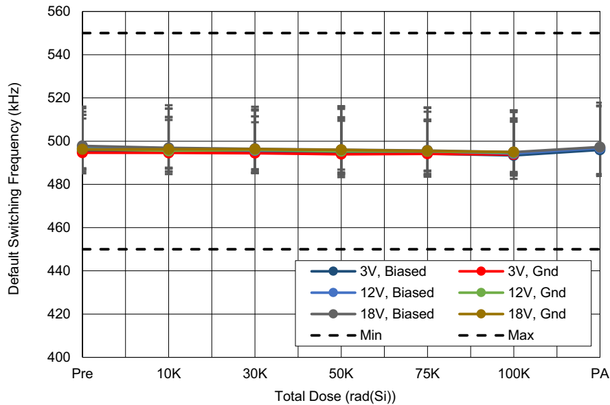
Figure 13. ISL73007SEH default switching frequency ( f_{SWd} ) with PVIN = 3V, 12V, and 18V ; FS = VCC as a function of LDR irradiation and anneal for biased and grounded configurations. The error bars (if visible) represent the minimum and maximum measured values. The post-irradiation datasheet limits are 450kHz minimum and 550kHz maximum.
