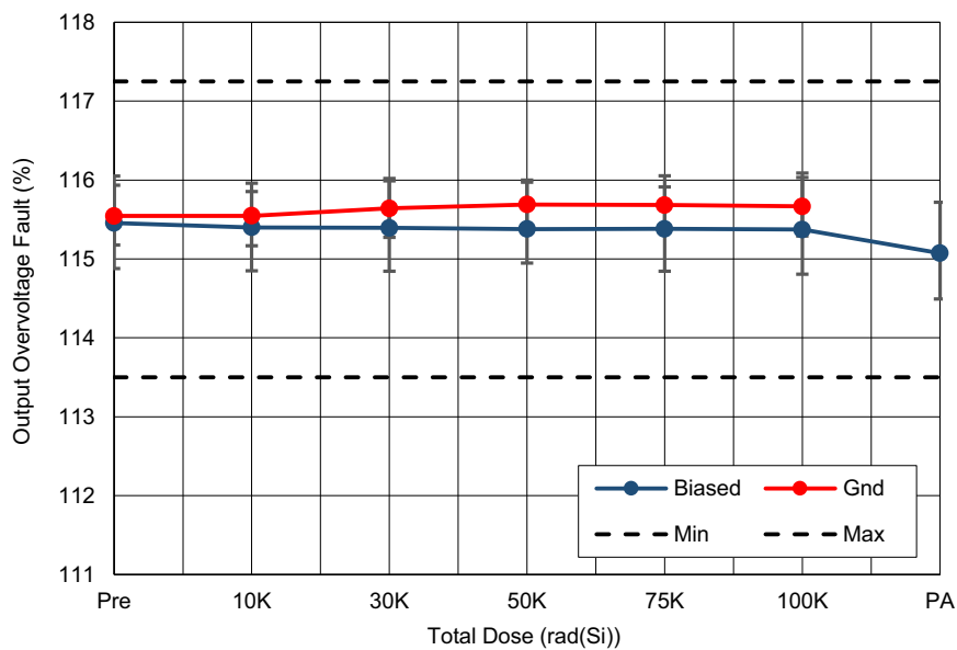
Figure 32. ISL73007SEH output overvoltage fault (OVflt) with PV_{IN} = 5V as a function of LDR irradiation and anneal for biased and grounded configurations. The error bars (if visible) represent the minimum and maximum measured values. The post-irradiation datasheet limits are 113.5% minimum and 117.25% maximum.
