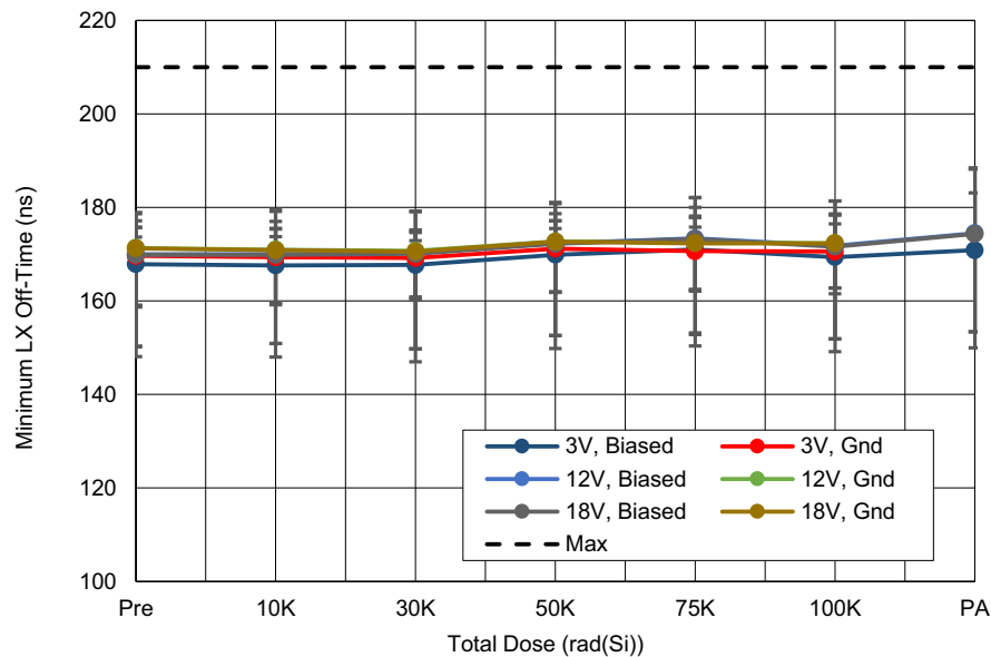
Figure 41. ISL73007SEH minimum LX off-time ( t_{\text{MIN\_OFF}} ) with \text{PVIN} = 3\text{V} , 12\text{V} , and 18\text{V} as a function of LDR irradiation and anneal for biased and grounded configurations. The error bars (if visible) represent the minimum and maximum measured values. The post-irradiation datasheet limit is 210ns maximum.
