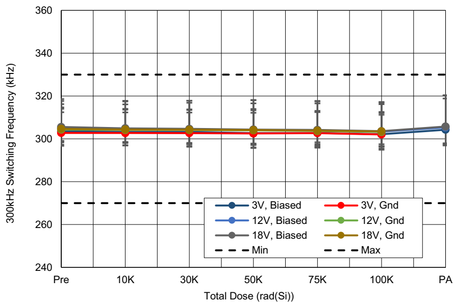
Figure 14. ISL73007SEH 300kHz switching frequency ( f_{SW3} ) with PVIN = 3V, 12V, and 18V ; FS = 174k\Omega to GND and VSLOPE = 1.2V as a function of LDR irradiation and anneal for biased and grounded configurations. The error bars (if visible) represent the minimum and maximum measured values. The post-irradiation datasheet limits are 270kHz minimum and 330kHz maximum.
