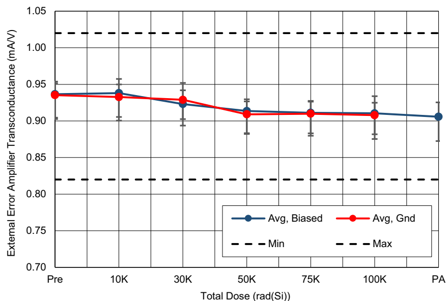
Figure 12. ISL73007SEH external error amplifier transconductance ( EA_{transcon2} ) with PV_{IN} = 5V , delta COMP current/delta FB voltage (10mV), as a function of LDR irradiation and anneal for biased and grounded configurations. The error bars (if visible) represent the minimum and maximum measured values. The post-irradiation datasheet limits are 0.82mA/V minimum and 1.02mA/V maximum.
