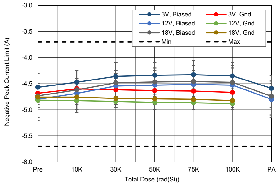
Figure 11. ISL73007SEH negative peak current limit ( -I_{PLIMIT} ) at PV_{IN} = 3V , 12V, and 18V, as a function of LDR irradiation and anneal for biased and grounded configurations. The error bars (if visible) represent the minimum and maximum measured values. The post-irradiation datasheet limits are -5.7A minimum and -3.7A maximum.
