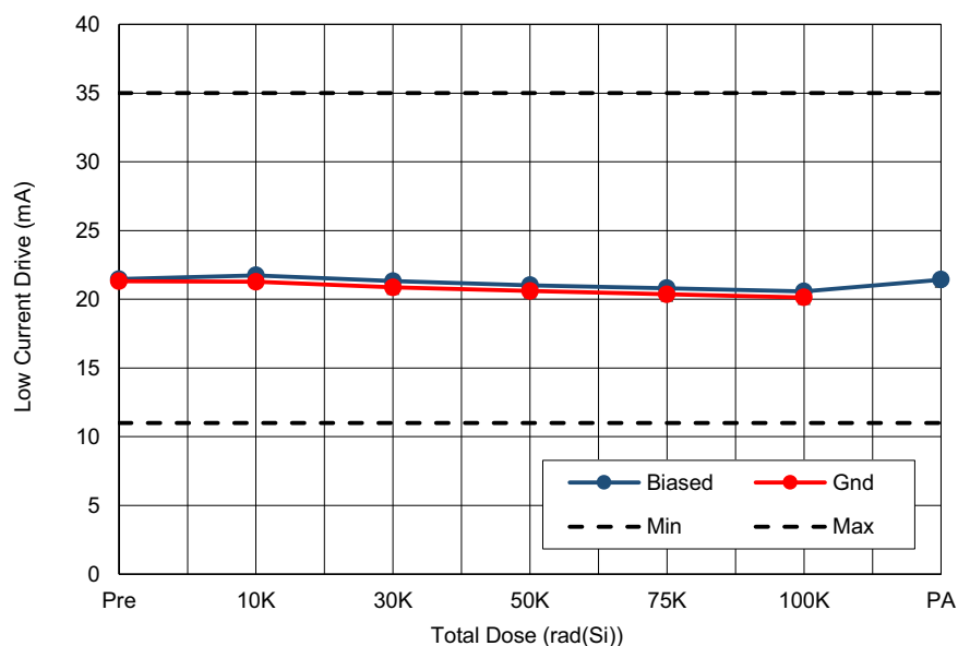
Figure 34. ISL73007SEH low current drive ( PG_{I_{OL}} ) with PV_{IN} = 3V , PG = 0.4V , and EN = 0V , as a function of LDR irradiation and anneal for biased and grounded configurations. The error bars (if visible) represent the minimum and maximum measured values. The post-irradiation datasheet limits are 11mA minimum and 35mA maximum.
