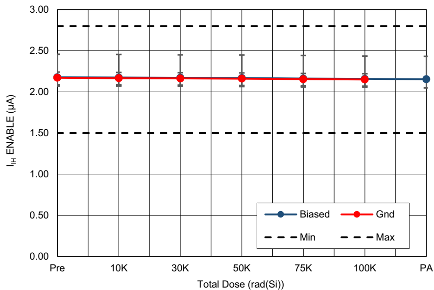
Figure 26. ISL73007SEH high enable current ( EN_{IH} ) with as a function of LDR irradiation and anneal for biased and grounded configurations. The error bars (if visible) represent the minimum and maximum measured values. The post-irradiation datasheet limits are 1.5\mu\text{A} minimum and 2.8\mu\text{A} maximum.
