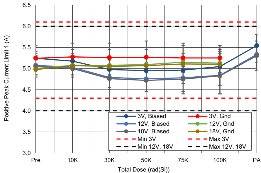
Figure 9. ISL73007SEH positive peak current limit ( I_{PLIMIT1} ) at PVIN = 3V , 12V, and 18V, as a function of LDR irradiation and anneal for biased and grounded configurations. The error bars (if visible) represent the minimum and maximum measured values. The post-irradiation datasheet limits are 4.3A minimum and 6.1A maximum for PVIN = 3V (shown in red) and 4A minimum and 6A maximum for PVIN \geq 5V (shown in black).
