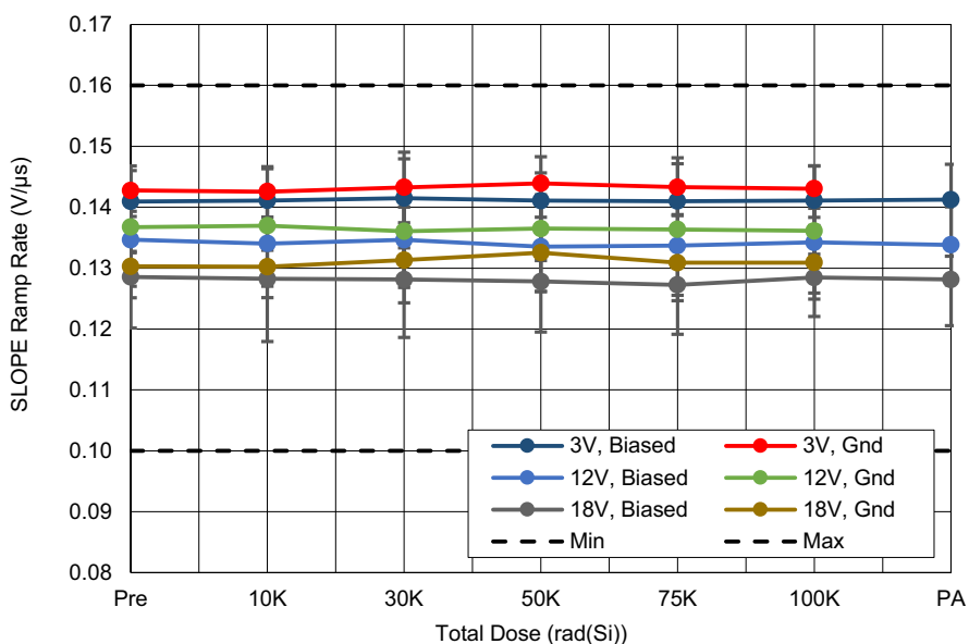
Figure 18. ISL73007SEH internal SLOPE ramp rate ( t_{SLOPE} ) with PV_{IN} = 3V, 12V, and 18V ; ( V_{COMP} at 80% DC - V_{COMP} at 20% DC) / ( t_{MIN\_ON} at 80% DC - t_{MIN\_ON} at 20% DC) as a function of LDR irradiation and anneal for biased and grounded configurations. The error bars (if visible) represent the minimum and maximum measured values. The post-irradiation datasheet limits are 0.1V/\mu s minimum and 0.16V/\mu s maximum.
