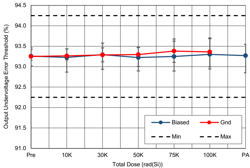
Figure 31. ISL73007SEH undervoltage fault threshold (UVP) with PV_{IN} = 5V as a function of LDR irradiation and anneal for biased and grounded configurations. The error bars (if visible) represent the minimum and maximum measured values. The post-irradiation datasheet limits are 92.25% minimum and 94.25% maximum.
