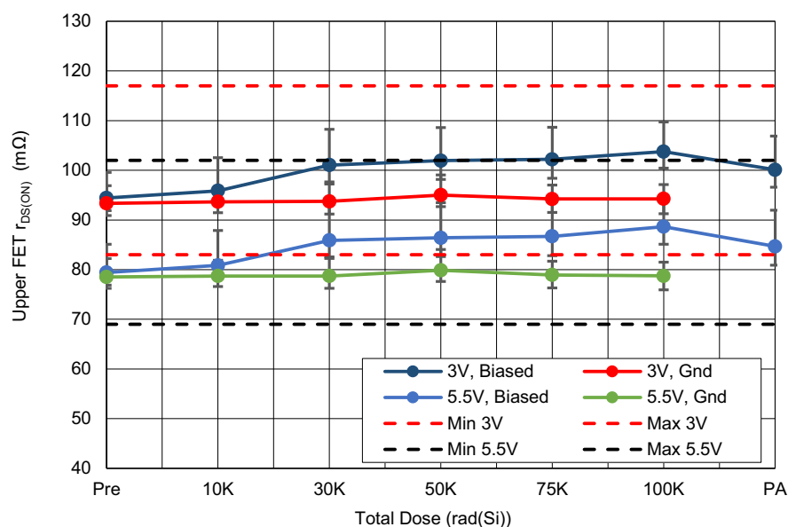
Figure 42. ISL73007SEH post-rad CDFP upper FET ON-resistance ( 25\text{UPR}_{\text{DS(on)3}} , 25\text{UPR}_{\text{DS(on)5}} ) with \text{PVIN} = 3\text{V} and 5.5\text{V} , and I_{\text{OUT}} = 200\text{mA} , as a function of LDR irradiation and anneal for biased and grounded configurations. The error bars (if visible) represent the minimum and maximum measured values. The post-irradiation datasheet limits are 83 \text{m}\Omega minimum and 117 \text{m}\Omega maximum for \text{PVIN} = 3\text{V} (shown in red) and 69 \text{m}\Omega minimum and 102 \text{m}\Omega maximum for \text{PVIN} = 5.5\text{V} (shown in black).
