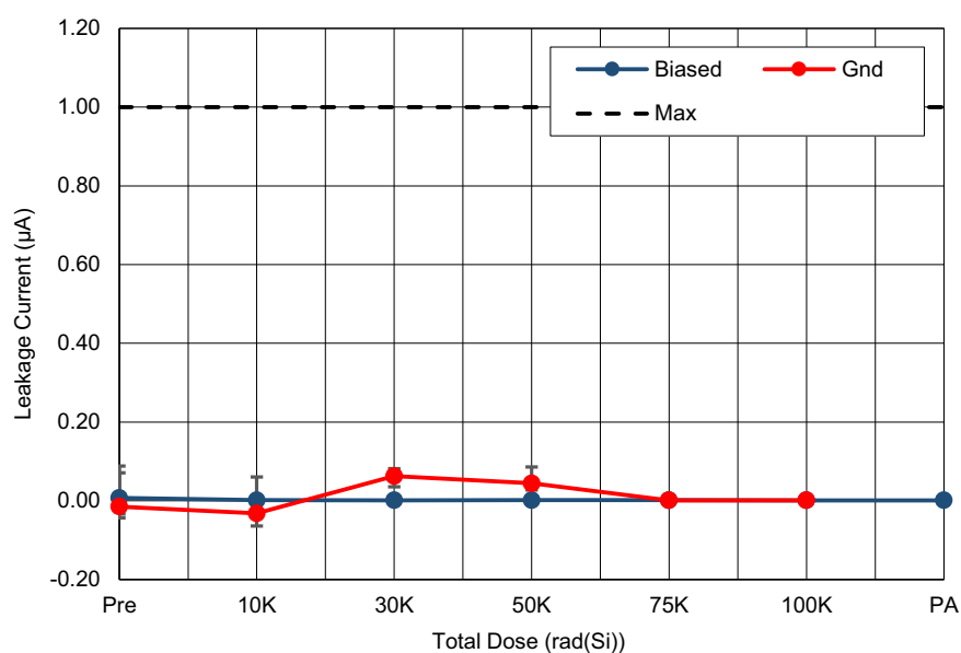
Figure 36. ISL73007SEH leakage ( I_{LKGP} ) with PVIN = PG = 18V , as a function of LDR irradiation and anneal for biased and grounded configurations. The error bars (if visible) represent the minimum and maximum measured values. The post-irradiation datasheet limit is 1 \mu A maximum.
