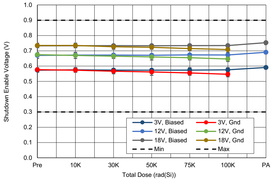
Figure 23. ISL73007SEH shutdown enable voltage ( SB\_EN_{VIL} ) with PVIN = 3V, 12V, and 18V as a function of LDR irradiation and anneal for biased and grounded configurations. The error bars (if visible) represent the minimum and maximum measured values. The post-irradiation datasheet limits are 0.3V minimum and 0.9V maximum.
