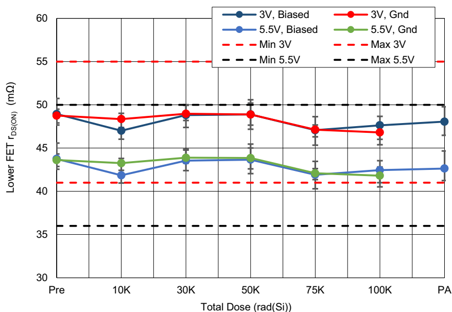
Figure 43. ISL73007SEH post-rad CDFP lower FET ON-resistance ( 25LWR_{DS0N\_3} , 25LWR_{DS0N\_3} ) with PVIN = 3V and 5.5V , and I_{OUT} = 200mA , as a function of LDR irradiation and anneal for biased and grounded configurations. The error bars (if visible) represent the minimum and maximum measured values. The post-irradiation datasheet limits are 41m\Omega minimum and 55m\Omega maximum for PVIN = 3V (shown in red) and 36m\Omega minimum and 50m\Omega maximum for PVIN = 5.5V (shown in black).
