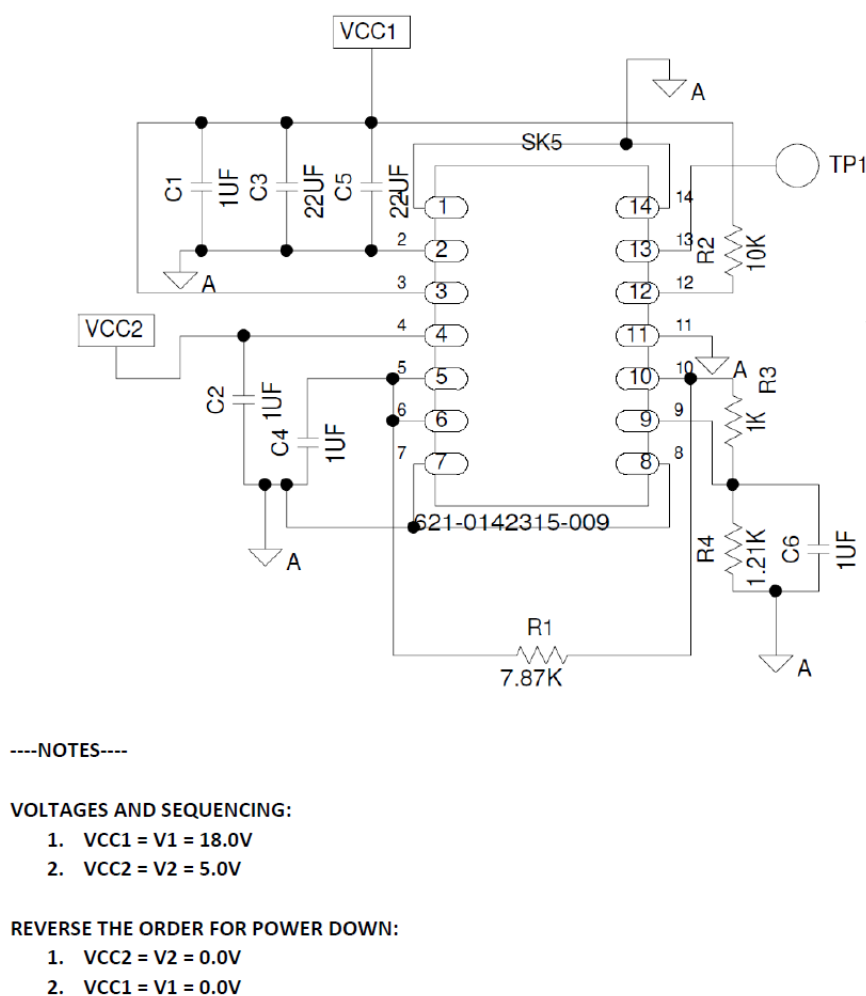
Figure 2. ISL73006SLH Irradiation Bias Configuration
