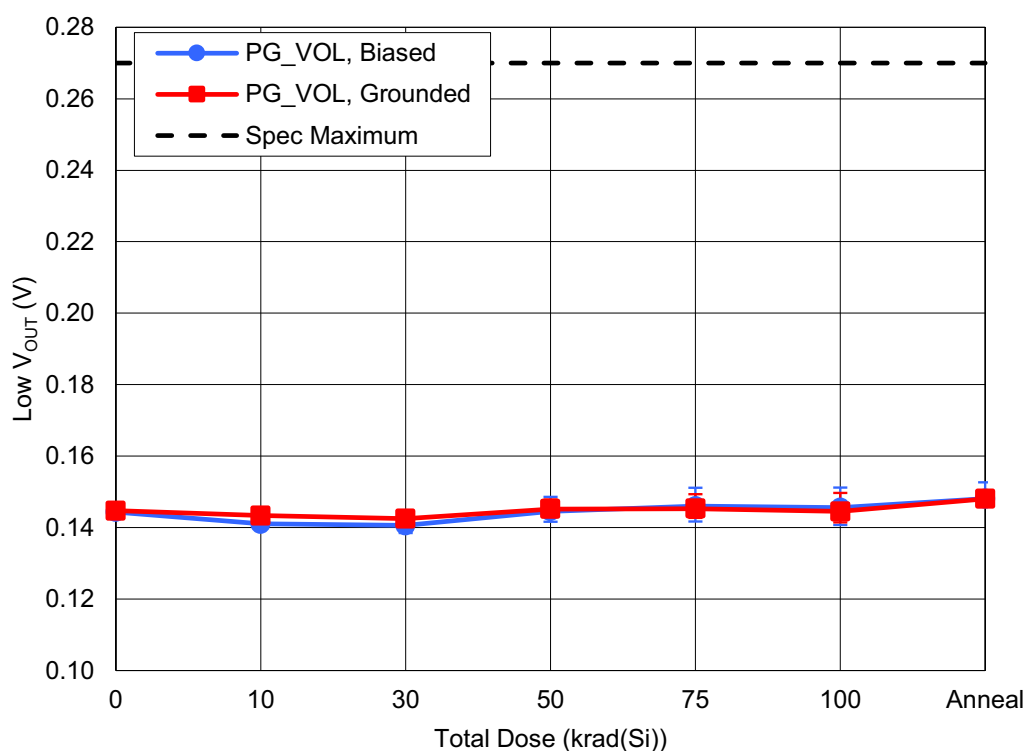
Figure 36. ISL73006SLH Low VOUT (PG_VOL) as a function of LDR irradiation and anneal for biased and grounded configurations. The error bars (if visible) represent the minimum and maximum measured values. The datasheet limit is a maximum of 0.27V.
