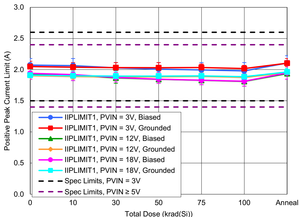
Figure 13. ISL73006SLH Positive Peak Current Limit ( I_{PLIMIT1} ) with PVIN = 3V , 12V , or 18V as a function of LDR irradiation and anneal for biased and grounded configurations. The error bars (if visible) represent the minimum and maximum measured values. The datasheet limits are a minimum of 1.5A and a maximum of 2.6A when PVIN = 3V or a minimum of 1.4A and a maximum of 2.4A when PVIN \geq 5V .
