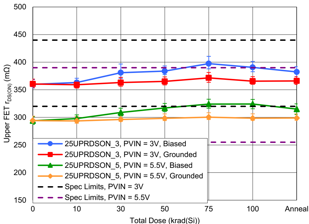
Figure 43. ISL73006SLH Post Rad CDFP Upper FET r_{DS(ON)} (25UPR_DS(ON)_3, 25UPR_DS(ON)_5) with PVIN = 3V or 5.5V as a function of LDR irradiation and anneal for biased and grounded configurations. The error bars (if visible) represent the minimum and maximum measured values. The datasheet limits are a minimum of 320mΩ and a maximum of 440mΩ when PVIN = 3V or a minimum of 255mΩ and a maximum of 390mΩ when PVIN = 5.5V.
