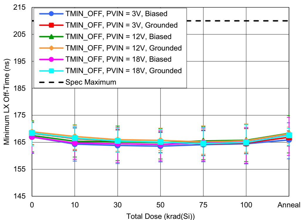
Figure 42. ISL73006SLH Minimum LX Off-Time ( t_{\text{MIN\_OFF}} ) with PVIN = 3V, 12V or 18V as a function of LDR irradiation and anneal for biased and grounded configurations. The error bars (if visible) represent the minimum and maximum measured values. The datasheet limit is a maximum of 210ns.
