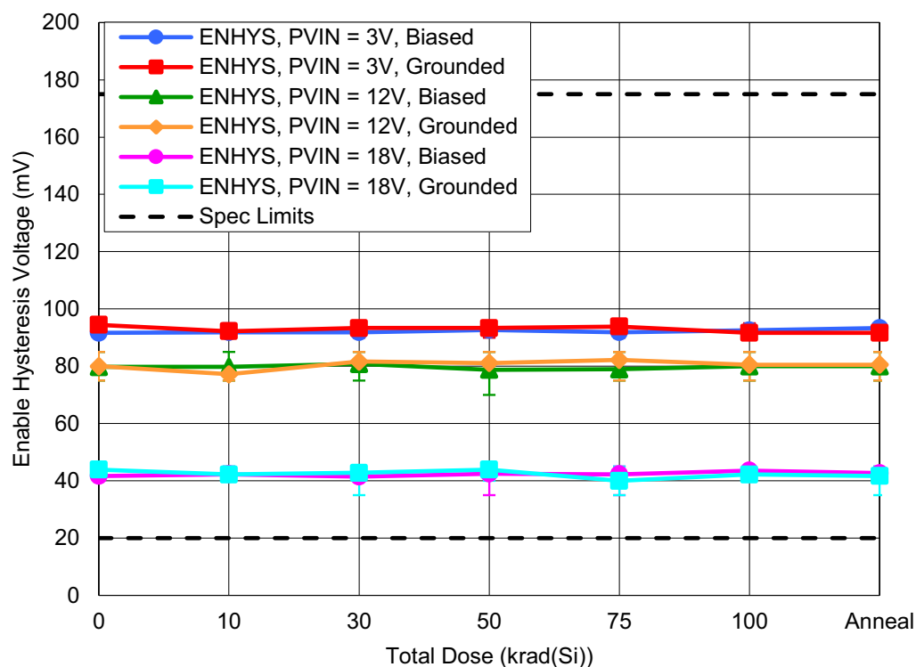
Figure 25. ISL73006SLH Enable Hysteresis Voltage ( EN_{HYS} ) with PVIN = 3V, 12V, or 18V as a function of LDR irradiation and anneal for biased and grounded configurations. The error bars (if visible) represent the minimum and maximum measured values. The datasheet limits are a minimum of 20mV and a maximum of 175mV.
