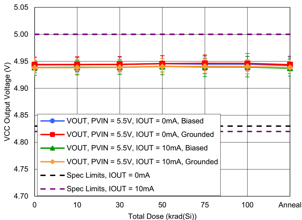
Figure 30. ISL73006SLH V_{CC} Output Voltage ( V_{OUT_{5V,0mA}} , V_{OUT_{5V,10mA}} ) with PV_{IN} = 5.5V , and with I_{OUT} = 0mA or 10mA as a function of LDR irradiation and anneal for biased and grounded configurations. The error bars (if visible) represent the minimum and maximum measured values. The datasheet limits are a minimum of 4.83V and a maximum of 5V when I_{OUT} = 0mA or a minimum of 4.82V and a maximum of 5V when I_{OUT} = 10mA .
