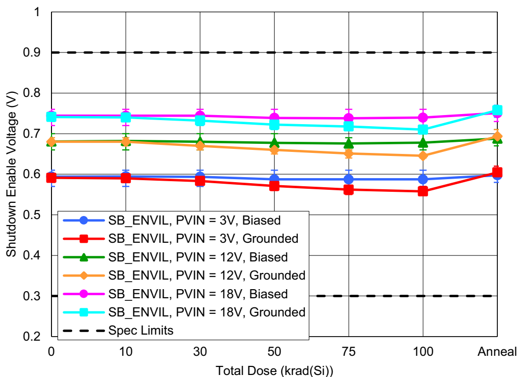
Figure 24. ISL73006SLH Shutdown Enable Voltage ( SB\_EN_{VIL} ) with PVIN = 3V , 12V , or 18V as a function of LDR irradiation and anneal for biased and grounded configurations. The error bars (if visible) represent the minimum and maximum measured values. The datasheet limits are a minimum of 0.3V and a maximum of 0.9V .
