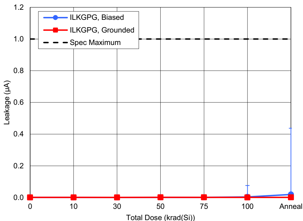
Figure 37. ISL73006SLH Leakage ( I_{LKGP} ) with PVIN = PGOOD = 18V as a function of LDR irradiation and anneal for biased and grounded configurations. The error bars (if visible) represent the minimum and maximum measured values. The datasheet limit is a maximum of 1\mu A .
