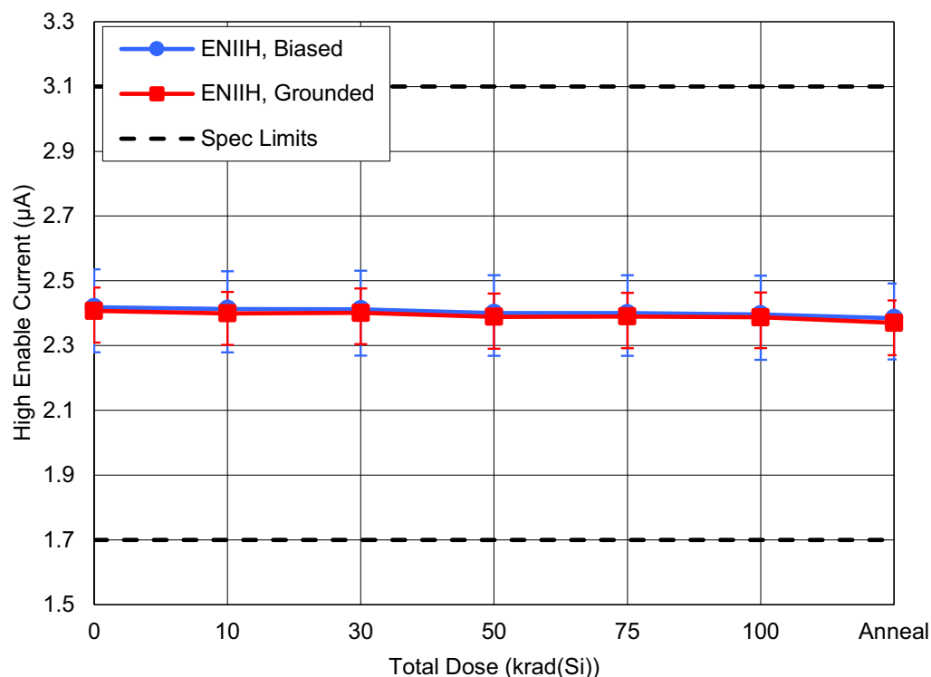
Figure 27. ISL73006SLH High Enable Current ( EN_{IH} ) as a function of LDR irradiation and anneal for biased and grounded configurations. The error bars (if visible) represent the minimum and maximum measured values. The datasheet limits are a minimum of 1.7 \mu A and a maximum of 3.1 \mu A .
