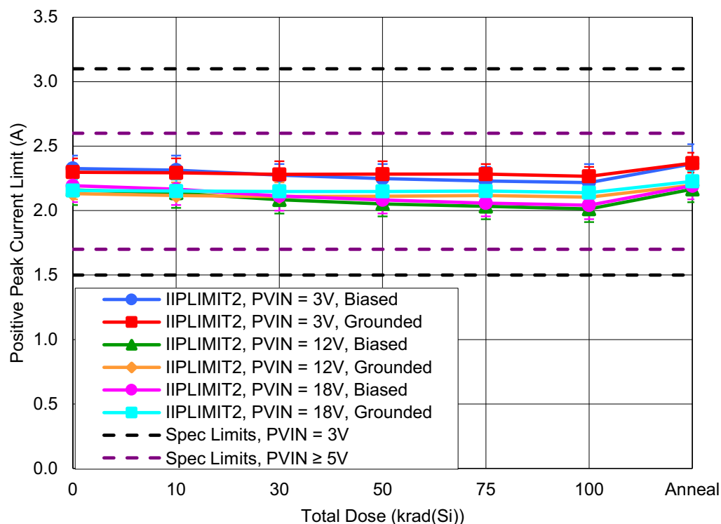
Figure 14. ISL73006SLH Positive Peak Current Limit ( I_{PLIMIT2} ) with PVIN = 3V , 12V , or 18V as a function of LDR irradiation and anneal for biased and grounded configurations. The error bars (if visible) represent the minimum and maximum measured values. The datasheet limits are a minimum of 1.5A and a maximum of 3.1A when PVIN = 3V or a minimum of 1.7A and a maximum of 2.6A when PVIN \geq 5V .
