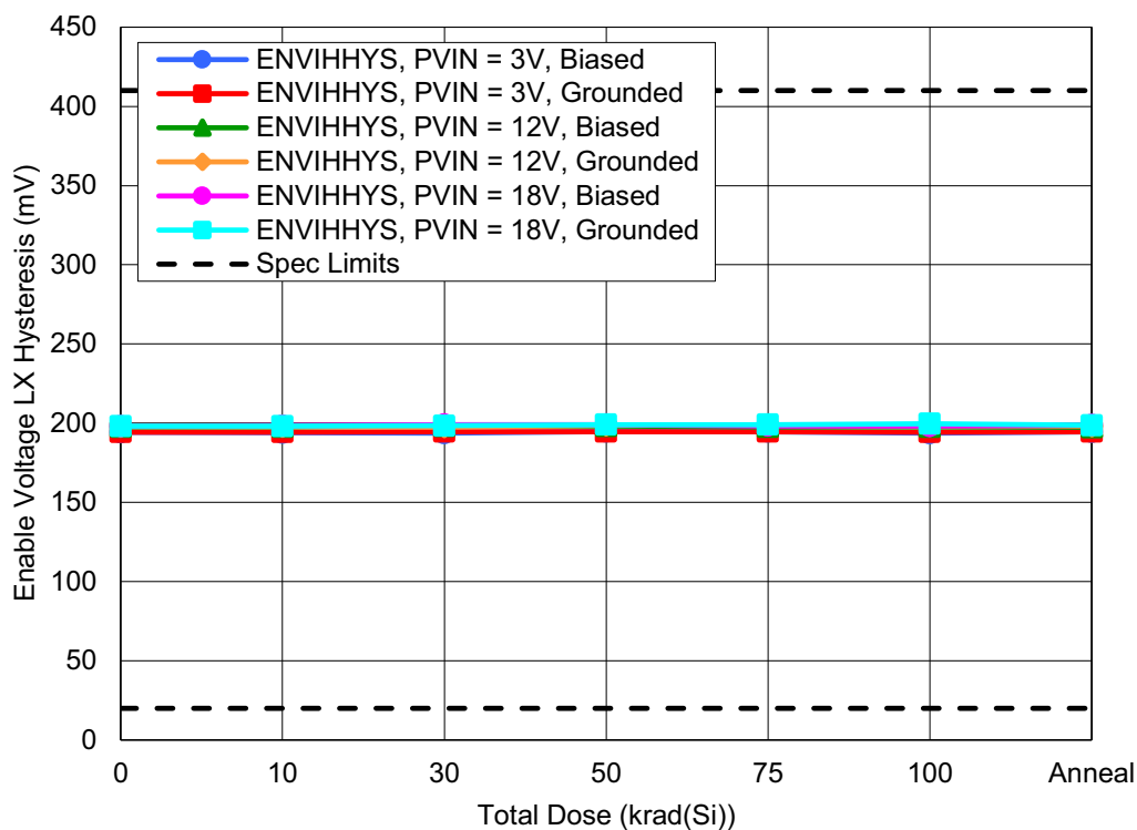
Figure 22. ISL73006SLH Enable Voltage LX Hysteresis ( EN_{VLHys} ) with PVIN = 3V, 12V , or 18V as a function of LDR irradiation and anneal for biased and grounded configurations. The error bars (if visible) represent the minimum and maximum measured values. The datasheet limits are a minimum of 20mV and a maximum of 410mV .
