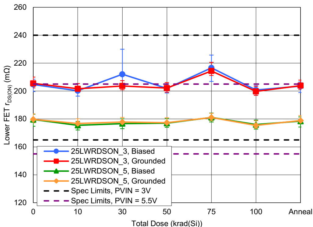
Figure 44. ISL73006SLH Post Rad CDFP Lower FET r_{DS(ON)} (25LWR_DS(ON)_3, 25LWR_DS(ON)_5) with PVIN = 3V or 5.5V as a function of LDR irradiation and anneal for biased and grounded configurations. The error bars (if visible) represent the minimum and maximum measured values. The datasheet limits are a minimum of 165mΩ and a maximum of 240mΩ when PVIN = 3V or a minimum of 155mΩ and a maximum of 205mΩ when PVIN = 5.5V.
