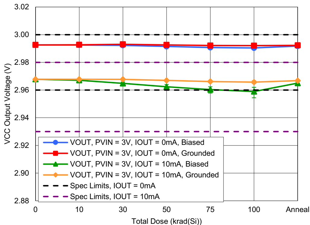
Figure 29. ISL73006SLH V_{CC} Output Voltage ( V_{OUT_{3V,0mA}} , V_{OUT_{3V,10mA}} ) with PV_{IN} = 3V , and with I_{OUT} = 0mA or 10mA as a function of LDR irradiation and anneal for biased and grounded configurations. The error bars (if visible) represent the minimum and maximum measured values. The datasheet limits are a minimum of 2.96V and a maximum of 3V when I_{OUT} = 0mA or a minimum of 2.93V and a maximum of 2.98V when I_{OUT} = 10mA .
