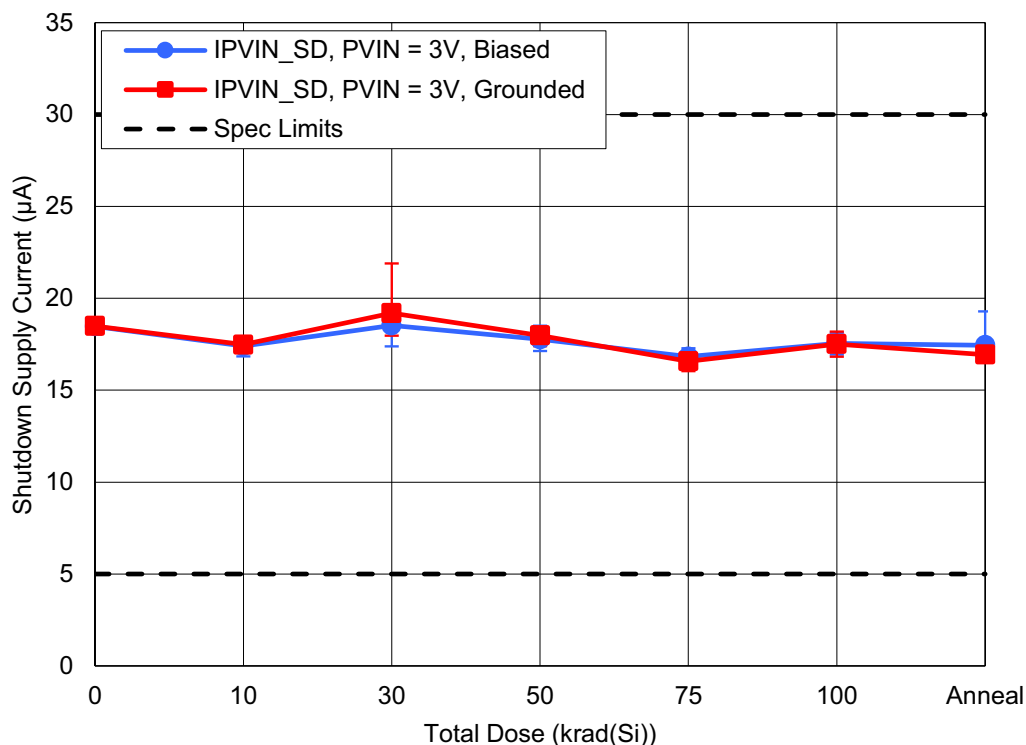
Figure 9. ISL73006SLH Shutdown Supply Current ( I_{PVIN\_SD} ) with PV_{IN} = 3V as a function of LDR irradiation and anneal for biased and grounded configurations. The error bars (if visible) represent the minimum and maximum measured values. The datasheet limits are a minimum of 5 \mu A and a maximum of 30 \mu A .
