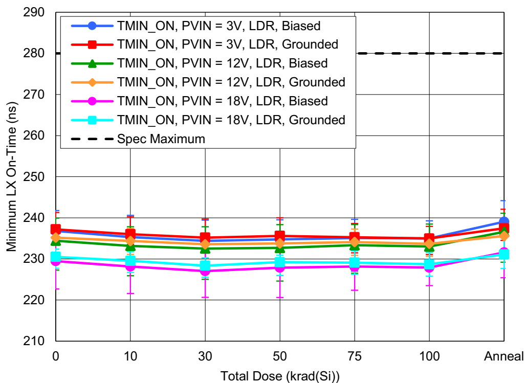
Figure 41. ISL73006SLH Minimum LX On-Time ( t_{\text{MIN\_ON}} ) with PVIN = 3V, 12V or 18V as a function of LDR irradiation and anneal for biased and grounded configurations. The error bars (if visible) represent the minimum and maximum measured values. The datasheet limit is a maximum of 280ns.
