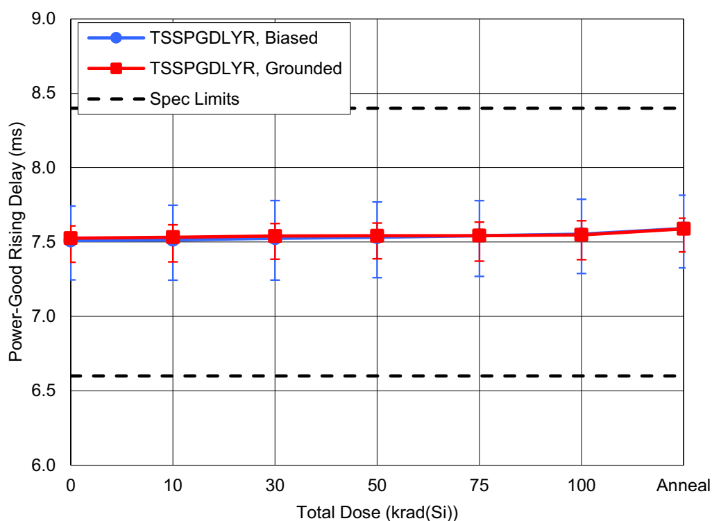
Figure 38. ISL73006SLH Power-Good Rising Delay ( t_{SPGDLYR} ) with PVIN = 5.5V at 500kHz as a function of LDR irradiation and anneal for biased and grounded configurations. The error bars (if visible) represent the minimum and maximum measured values. The datasheet limits are a minimum of 6.6ms and a maximum of 8.4ms .
