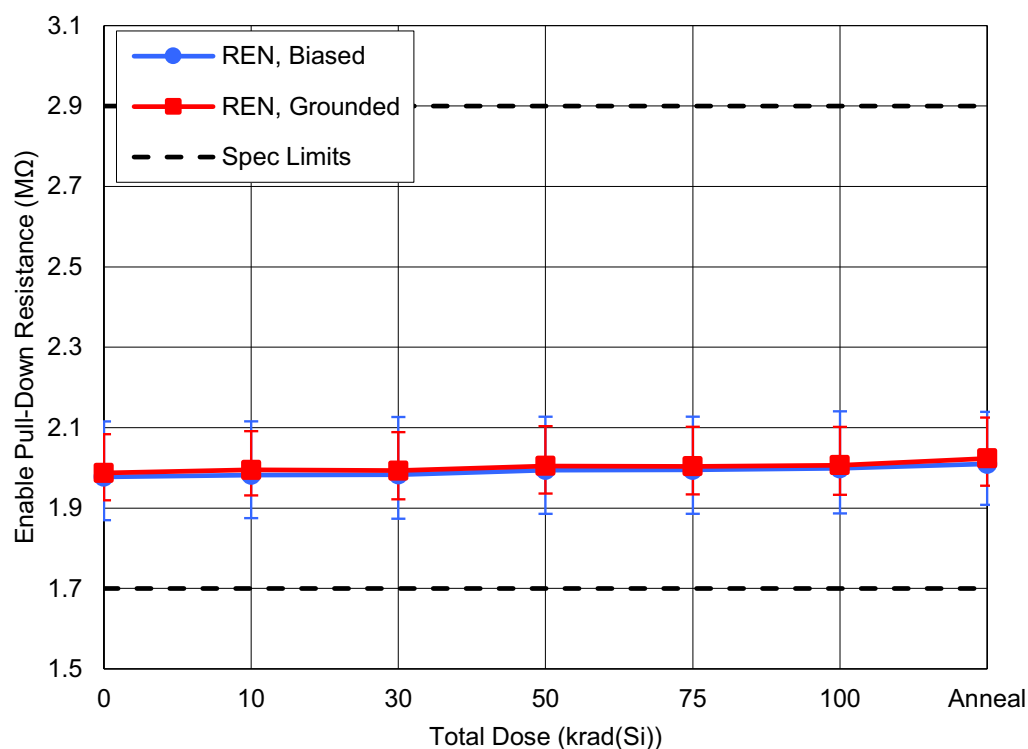
Figure 28. ISL73006SLH Enable Pull-Down Resistance ( R_{EN} ) with PV_{IN} = 12V as a function of LDR irradiation and anneal for biased and grounded configurations. The error bars (if visible) represent the minimum and maximum measured values. The datasheet limits are a minimum of 1.7 M\Omega and a maximum of 2.9 M\Omega .
