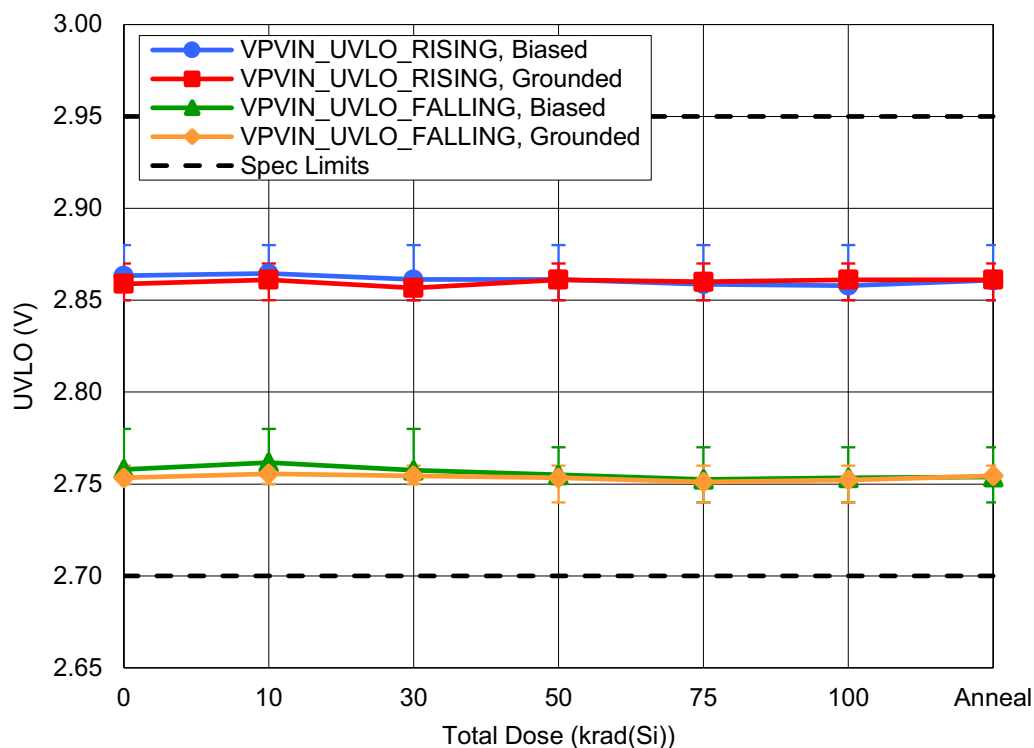
Figure 3. ISL73006SLH Rising and Falling Undervoltage Lockout ( V_{PIN\_UVLO} ) as a function of LDR irradiation and anneal for biased and grounded configurations. The error bars (if visible) represent the minimum and maximum measured values. The datasheet limits are a minimum of 2.7V for Falling Undervoltage Lockout and a maximum of 2.95V for Rising Undervoltage Lockout.
