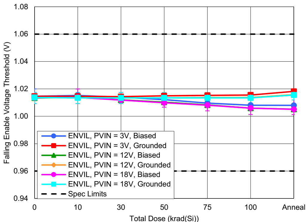
Figure 21. ISL73006SLH Falling Enable Voltage Threshold ( EN_{VIL} ) with PVIN = 3V, 12V , or 18V as a function of LDR irradiation and anneal for biased and grounded configurations. The error bars (if visible) represent the minimum and maximum measured values. The datasheet limits are a minimum of 0.96V and a maximum of 1.06V .
