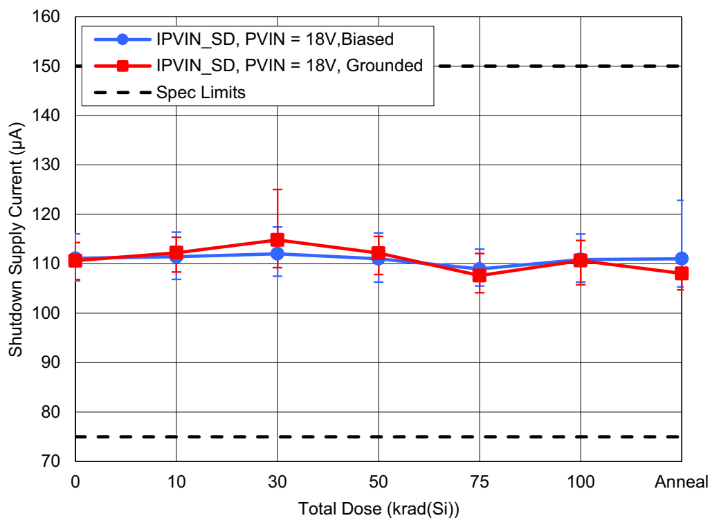
Figure 10. ISL73006SLH Shutdown Supply Current ( I_{PVIN\_SD} ) with PV_{IN} = 18V as a function of LDR irradiation and anneal for biased and grounded configurations. The error bars (if visible) represent the minimum and maximum measured values. The datasheet limits are a minimum of 75 \mu A and a maximum of 150 \mu A .
