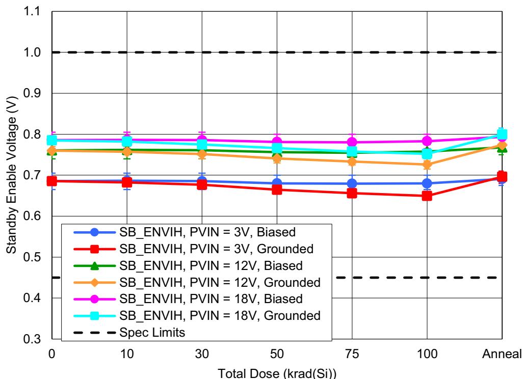
Figure 23. ISL73006SLH Standby Enable Voltage ( SB\_EN_{VIH} ) with PVIN = 3V , 12V , or 18V as a function of LDR irradiation and anneal for biased and grounded configurations. The error bars (if visible) represent the minimum and maximum measured values. The datasheet limits are a minimum of 0.45V and a maximum of 1V .
