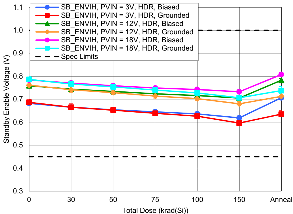
Figure 23. ISL73006SLH Standby Enable Voltage ( SB\_EN_{VIH} ) with PVIN = 3V , 12V , or 18V as a function of HDR irradiation and anneal for biased and grounded configurations. The error bars (if visible) represent the minimum and maximum measured values. The datasheet limits are a minimum of 0.45V and a maximum of 1V .
