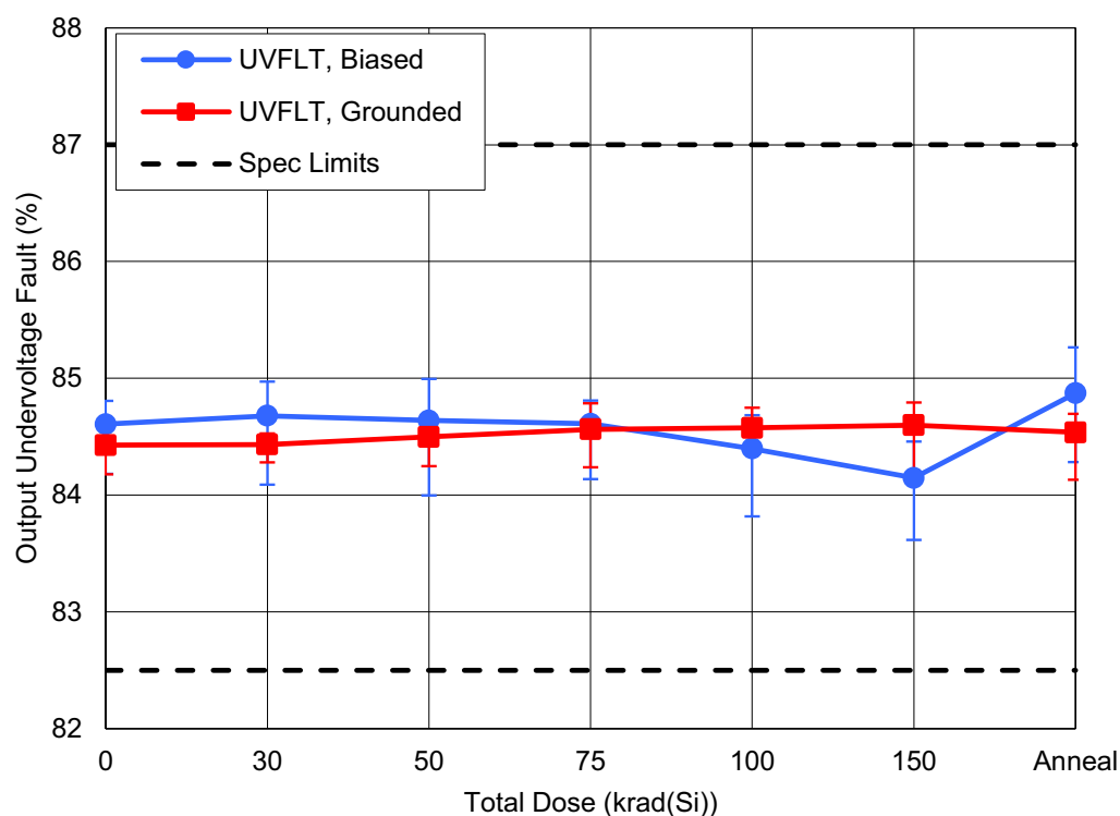
Figure 34. ISL73006SLH Output Undervoltage Fault (UV flt ) as a function of HDR irradiation and anneal for biased and grounded configurations. The error bars (if visible) represent the minimum and maximum measured values. The datasheet limits are a minimum of 82.5% and a maximum of 87%.
