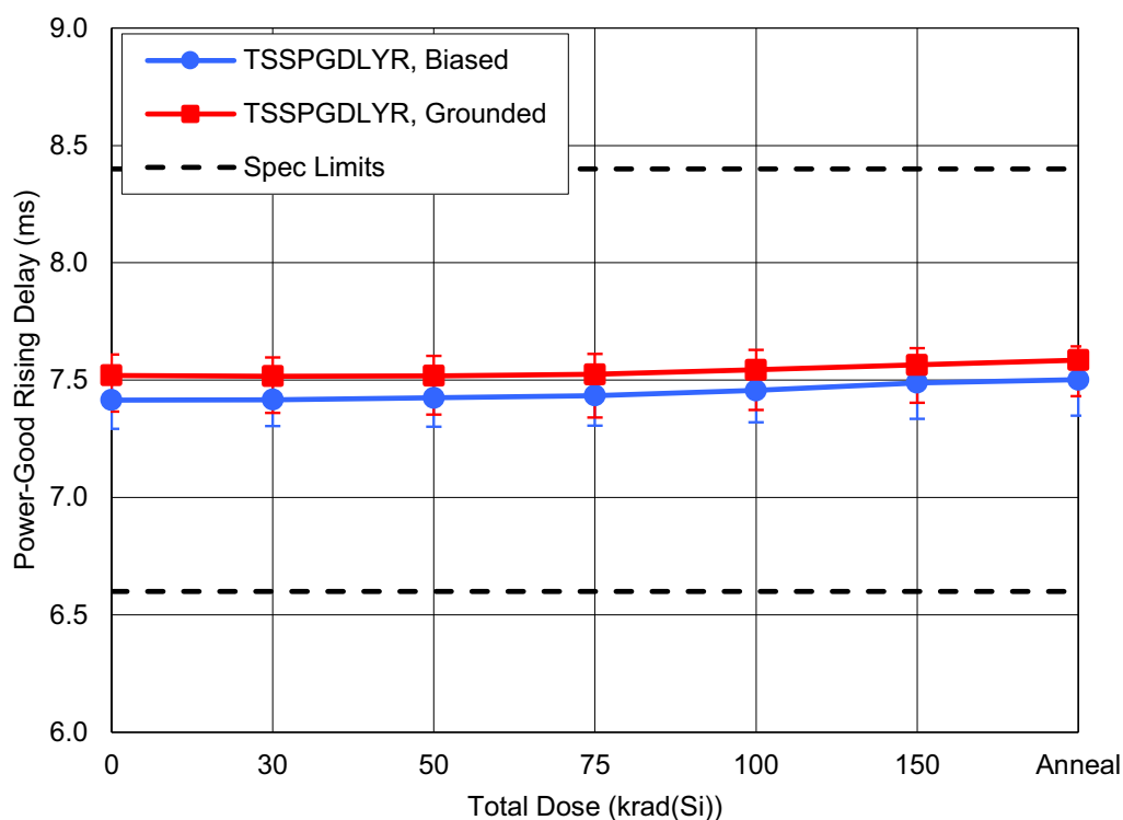
Figure 38. ISL73006SLH Power-Good Rising Delay ( t_{SPGDLYR} ) with PVIN = 5.5V at 500kHz as a function of HDR irradiation and anneal for biased and grounded configurations. The error bars (if visible) represent the minimum and maximum measured values. The datasheet limits are a minimum of 6.6ms and a maximum of 8.4ms.
