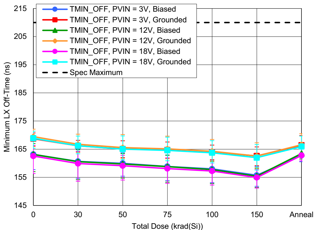
Figure 42. ISL73006SLH Minimum LX Off-Time ( t_{\text{MIN\_OFF}} ) with PVIN = 3V, 12V or 18V as a function of HDR irradiation and anneal for biased and grounded configurations. The error bars (if visible) represent the minimum and maximum measured values. The datasheet limit is a maximum of 210ns.
