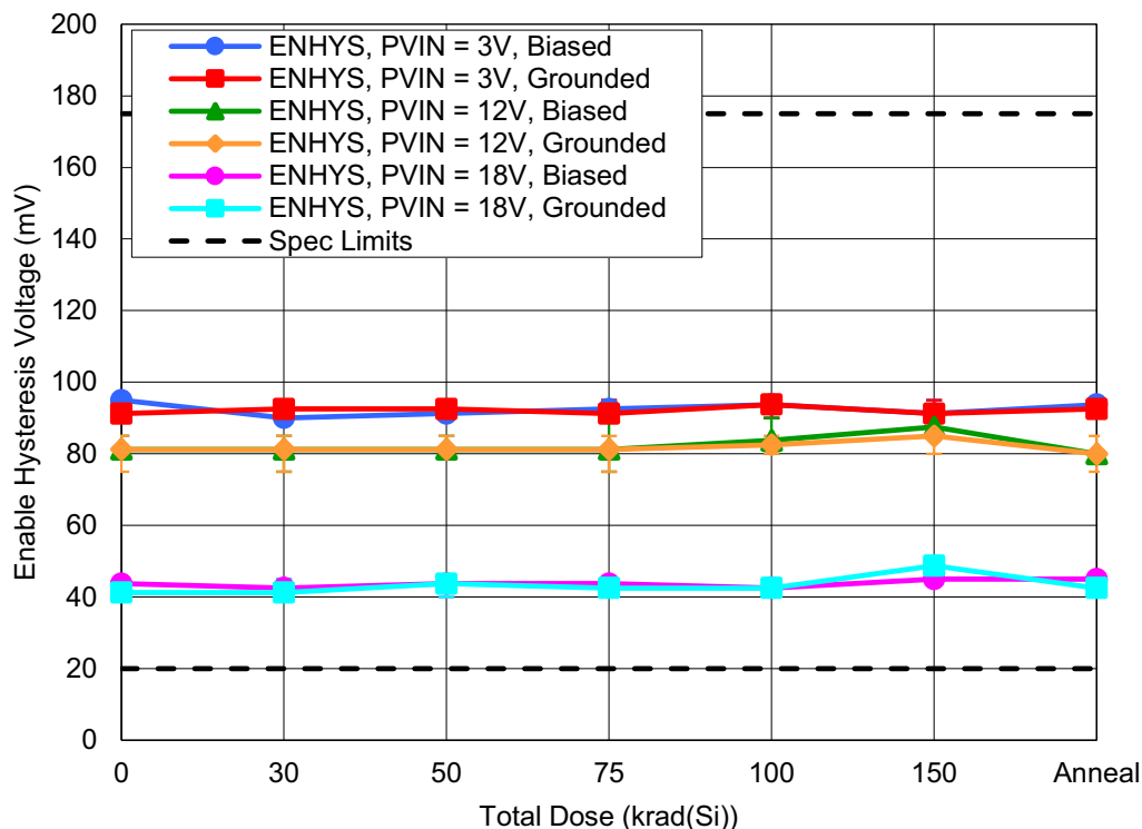
Figure 25. ISL73006SLH Enable Hysteresis Voltage ( EN_{HYS} ) with PVIN = 3V , 12V , or 18V as a function of HDR irradiation and anneal for biased and grounded configurations. The error bars (if visible) represent the minimum and maximum measured values. The datasheet limits are a minimum of 20mV and a maximum of 175mV .
