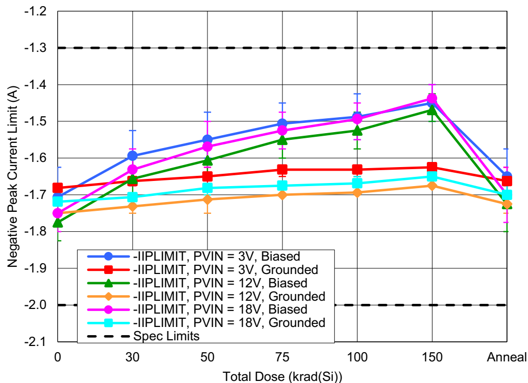
Figure 15. ISL73006SLH Negative Peak Current Limit ( -I_{PLIMIT} ) with PVIN = 3V, 12V, or 18V as a function of HDR irradiation and anneal for biased and grounded configurations. The error bars (if visible) represent the minimum and maximum measured values. The datasheet limits are a minimum of -2A and a maximum of -1.3A.
