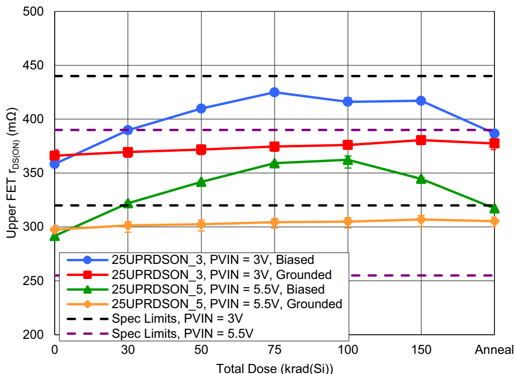
Figure 43. ISL73006SLH Post Rad CDFP Upper FET r_{DS(ON)} (25UPR_DS(ON)_3, 25UPR_DS(ON)_5) with PVIN = 3V or 5.5V as a function of HDR irradiation and anneal for biased and grounded configurations. The error bars (if visible) represent the minimum and maximum measured values. The datasheet limits are a minimum of 320mΩ and a maximum of 440mΩ when PVIN = 3V or a minimum of 255mΩ and a maximum of 390mΩ when PVIN = 5.5V.
