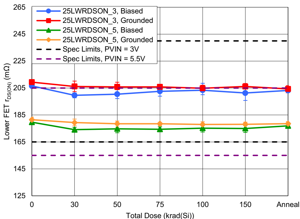
Figure 44. ISL73006SLH Post Rad CDFP Lower FET r_{DS(ON)} (25LWR_DS(ON)_3, 25LWR_DS(ON)_5) with PVIN = 3V or 5.5V as a function of HDR irradiation and anneal for biased and grounded configurations. The error bars (if visible) represent the minimum and maximum measured values. The datasheet limits are a minimum of 165mΩ and a maximum of 240mΩ when PVIN = 3V or a minimum of 155mΩ and a maximum of 205mΩ when PVIN = 5.5V.
