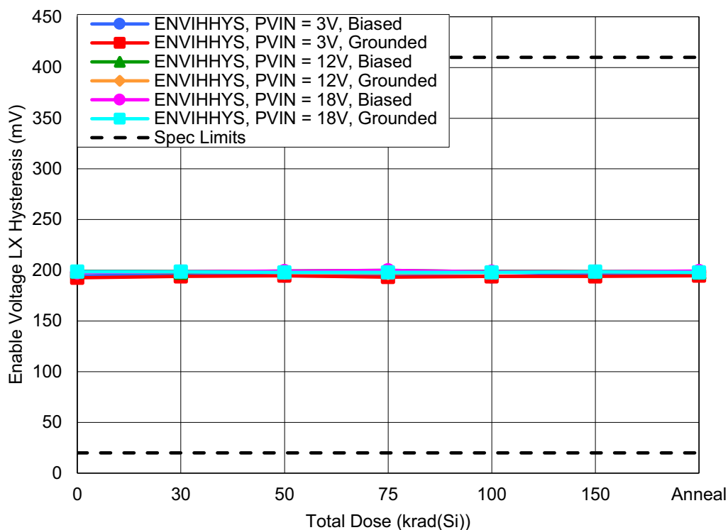
Figure 22. ISL73006SLH Enable Voltage LX Hysteresis ( EN_{VILHys} ) with PVIN = 3V, 12V , or 18V as a function of HDR irradiation and anneal for biased and grounded configurations. The error bars (if visible) represent the minimum and maximum measured values. The datasheet limits are a minimum of 20mV and a maximum of 410mV .
