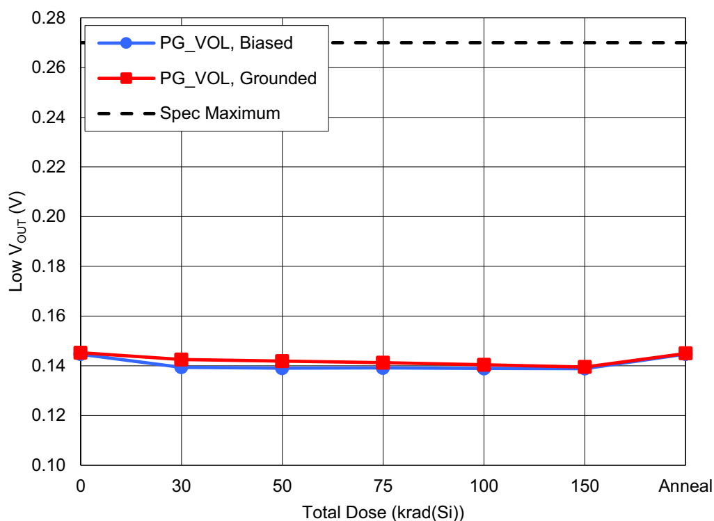
Figure 36. ISL73006SLH Low VOUT (PG_VOL) as a function of HDR irradiation and anneal for biased and grounded configurations. The error bars (if visible) represent the minimum and maximum measured values. The datasheet limit is a maximum of 0.27V.
