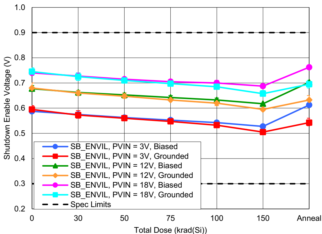
Figure 24. ISL73006SLH Shutdown Enable Voltage ( SB\_EN_{VIL} ) with PVIN = 3V , 12V , or 18V as a function of HDR irradiation and anneal for biased and grounded configurations. The error bars (if visible) represent the minimum and maximum measured values. The datasheet limits are a minimum of 0.3V and a maximum of 0.9V .
