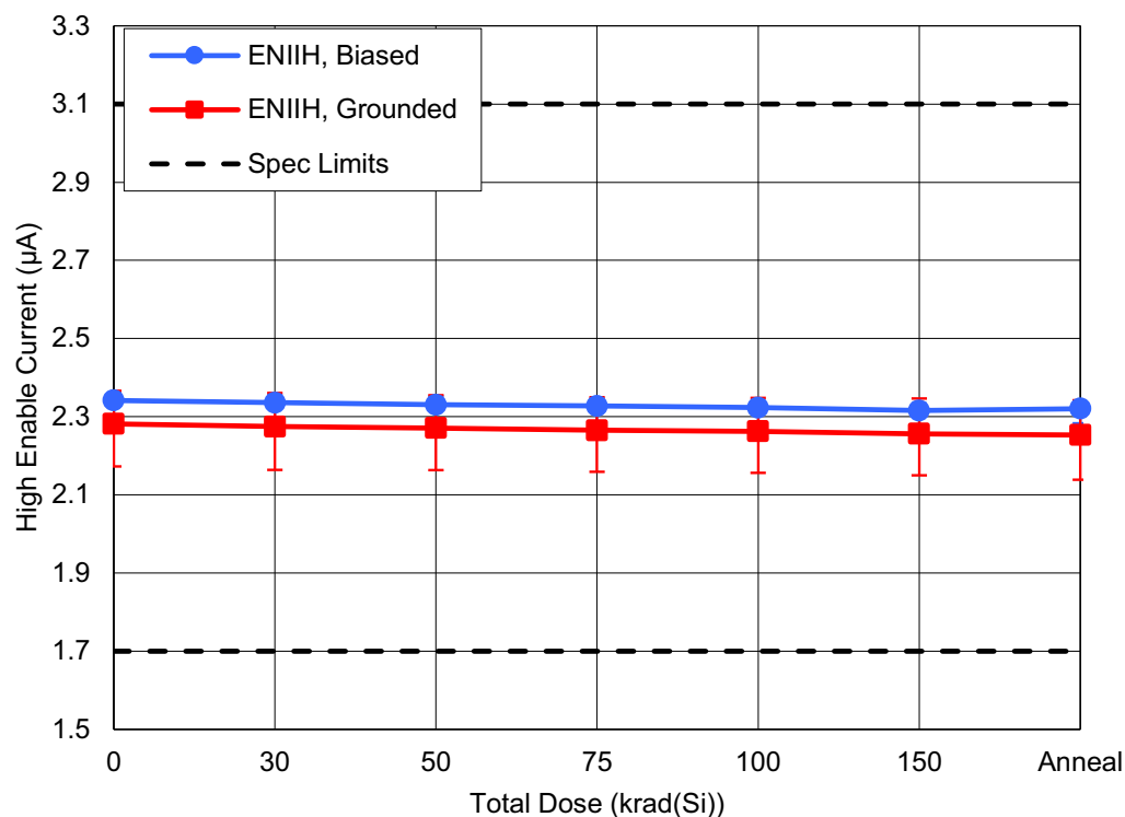
Figure 27. ISL73006SLH High Enable Current ( EN_{IH} ) as a function of HDR irradiation and anneal for biased and grounded configurations. The error bars (if visible) represent the minimum and maximum measured values. The datasheet limits are a minimum of 1.7 \mu A and a maximum of 3.1 \mu A .
