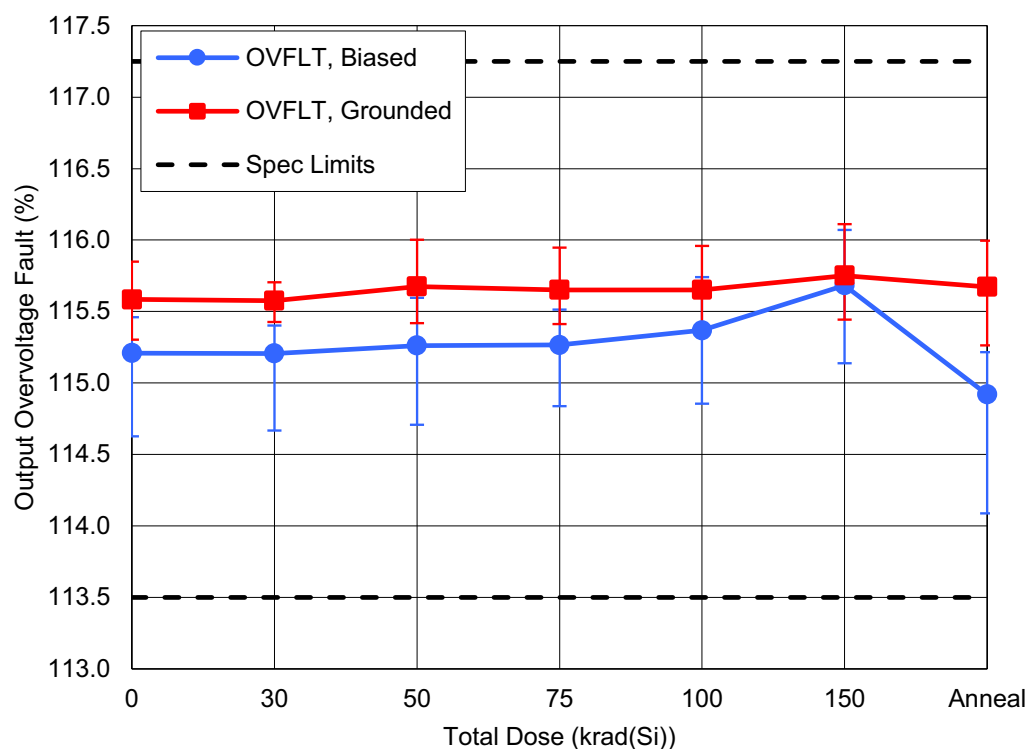
Figure 33. ISL73006SLH Output Overvoltage Fault (OV flt ) as a function of HDR irradiation and anneal for biased and grounded configurations. The error bars (if visible) represent the minimum and maximum measured values. The datasheet limits are a minimum of 113.5% and a maximum of 117.25%.
