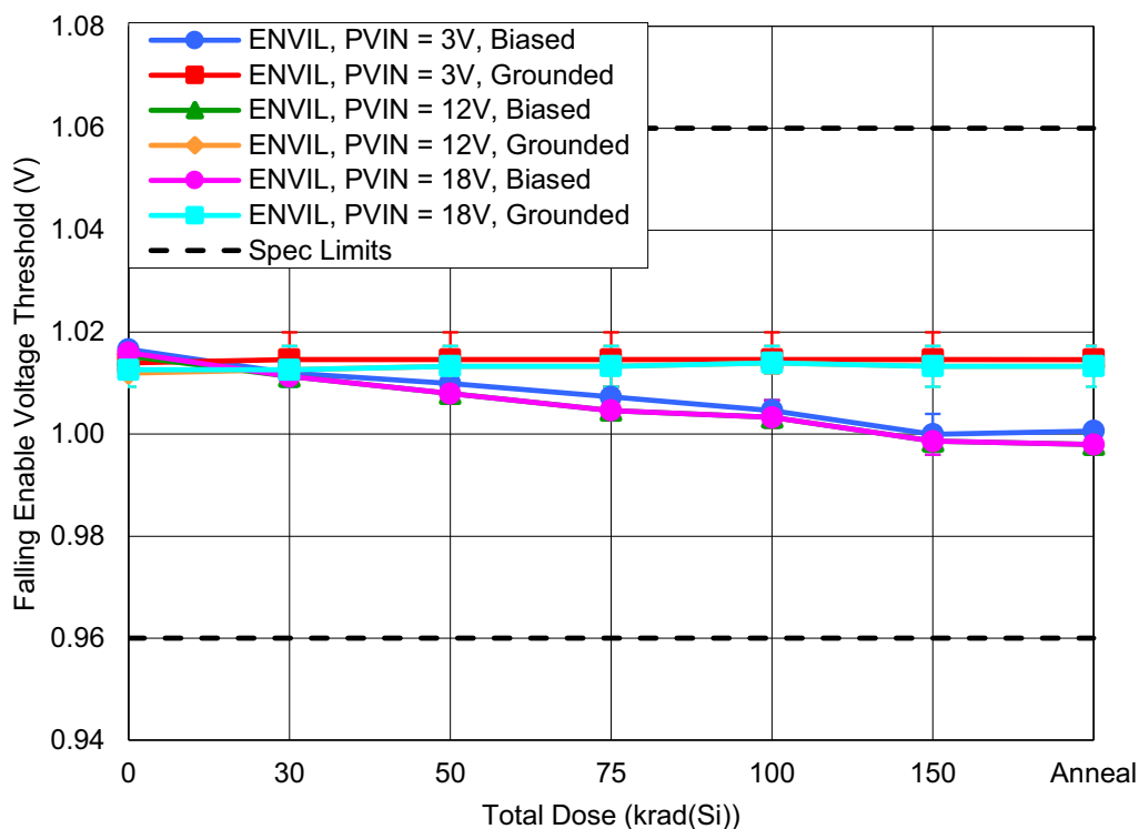
Figure 21. ISL73006SLH Falling Enable Voltage Threshold ( EN_{VIL} ) with PVIN = 3V, 12V , or 18V as a function of HDR irradiation and anneal for biased and grounded configurations. The error bars (if visible) represent the minimum and maximum measured values. The datasheet limits are a minimum of 0.96V and a maximum of 1.06V .
