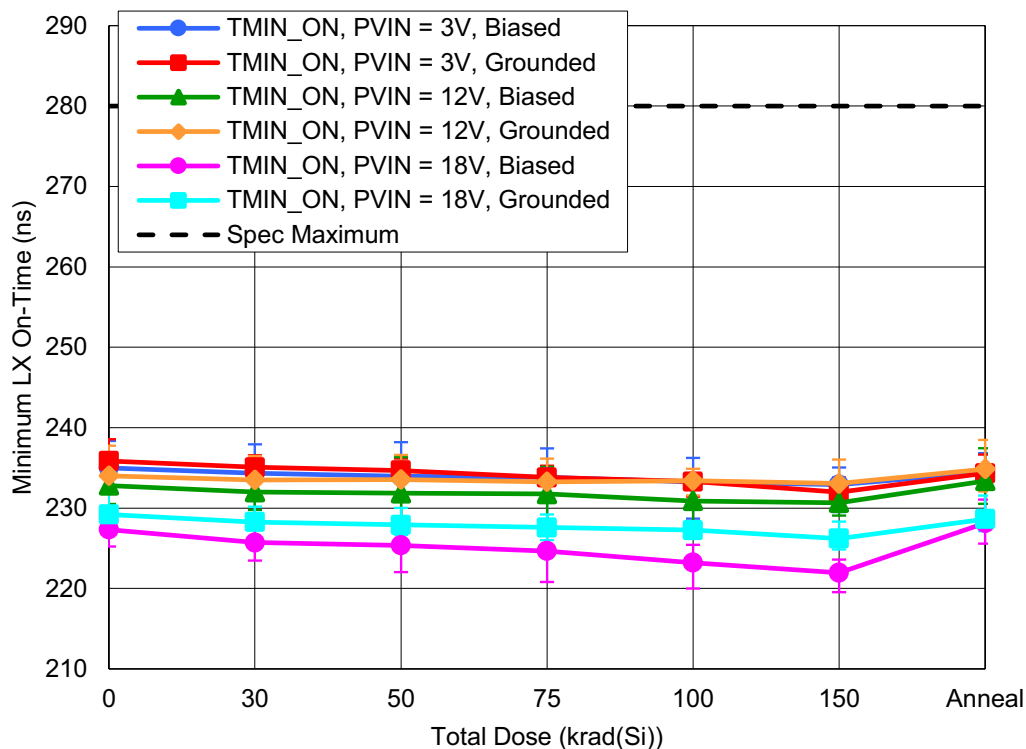
Figure 41. ISL73006SLH Minimum LX On-Time ( t_{\text{MIN\_ON}} ) with PVIN = 3V, 12V or 18V as a function of HDR irradiation and anneal for biased and grounded configurations. The error bars (if visible) represent the minimum and maximum measured values. The datasheet limit is a maximum of 280ns.
