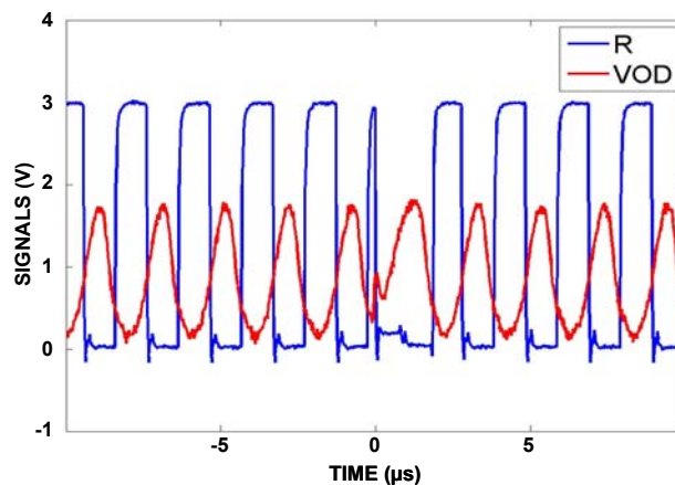
FIGURE 7B. TRANSMIT FAST OPEN CM
