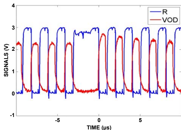
FIGURE 7A. TRANSMIT FAST -7V CM AND V REF
