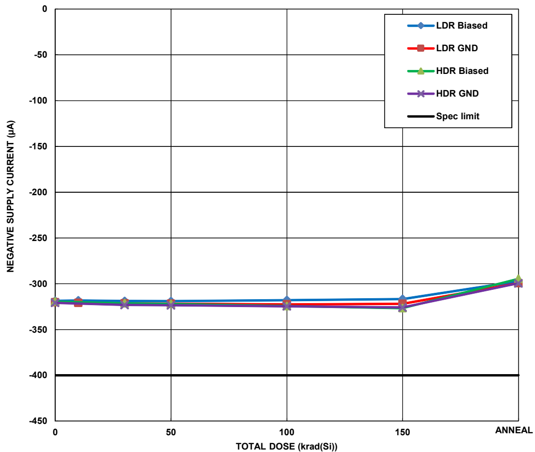
FIGURE 4. Median ISL71841SEH negative supply current as a function of total dose irradiation at high and low dose rate for the biased (per Figure 2 ) and unbiased (all pins grounded) cases. The low dose rate was 0.0085rad(Si)/s and the high dose rate was 69.7rad(Si)/s. Irradiations were followed by a 168-hour biased anneal at +100 °C. Sample size for the low dose rate cells was 13 and sample size for the high dose rate cells was 4. The post-irradiation SMD limit is -400µA minimum.
