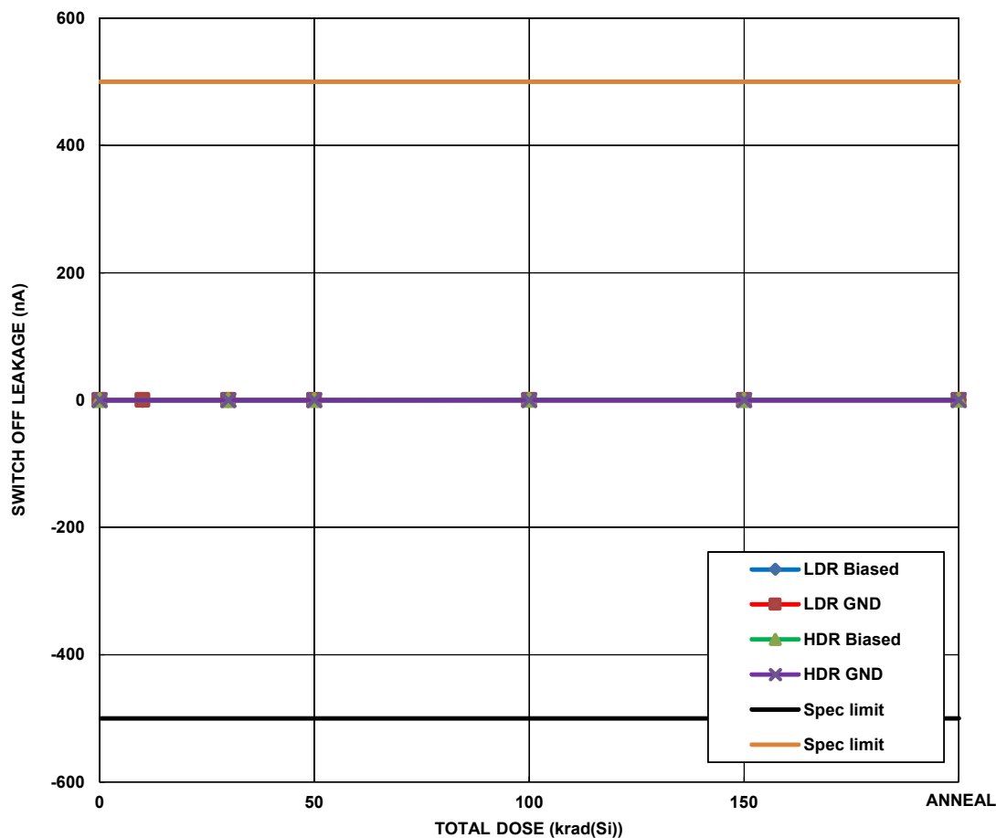
FIGURE 22. ISL71841SEH switch OFF leakage ( I_{D(OFF)} ) into the drain of an unselected channel, average of the medians of all 32 channels, supply voltage \pm 15.0V , input overvoltage -35.0V , as a function of total dose irradiation at high and low dose rate for the biased (Figure 2) and unbiased (all pins grounded) cases. The low dose rate was 0.0085\text{rad(Si)}/s and the high dose rate was 69.7\text{rad(Si)}/s . Irradiations were followed by a 168-hour biased anneal at +100^\circ\text{C} . Sample size for the low dose rate cells was 13 and sample size for the high dose rate cells was 4. The post-irradiation SMD limits are -500\text{nA} to +500\text{nA} .
