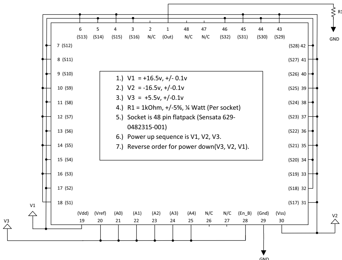
FIGURE 2. IRRADIATION BIAS CONFIGURATION AND POWER SUPPLY SEQUENCING FOR THE ISL71841SEH
