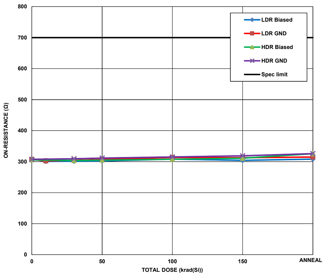
FIGURE 10. ISL71841SEH ON-resistance, average of the medians of all 32 channels, \pm 15\text{V} supplies, 1.0\text{mA} output current, -15.0\text{V} input voltage, as a function of total dose irradiation at high and low dose rate for the biased (Figure 2) and unbiased (all pins grounded) cases. The low dose rate was 0.0085\text{rad(Si)}/\text{s} and the high dose rate was 69.7\text{rad(Si)}/\text{s} . Irradiations were followed by a 168-hour biased anneal at +100^\circ\text{C} . Sample size for the low dose rate cells was 13 and sample size for the high dose rate cells was 4. The post-irradiation SMD limit is 700\Omega maximum.
