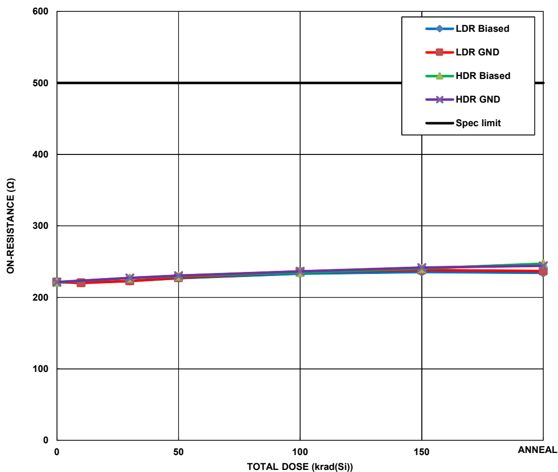
FIGURE 11. ISL71841SEH ON resistance, average of the medians of all 32 channels, \pm 15\text{V} supplies, 1.0\text{mA} output current, -5.0\text{V} input voltage, as a function of total dose irradiation at high and low dose rate for the biased (Figure 2) and unbiased (all pins grounded) cases. The low dose rate was 0.0085\text{rad(Si)/s} and the high dose rate was 69.7\text{rad(Si)/s} . Irradiations were followed by a 168-hour biased anneal at +100^\circ\text{C} . Sample size for the low dose rate cells was 13 and sample size for the high dose rate cells was 4. The post-irradiation SMD limit is 500\Omega maximum.
