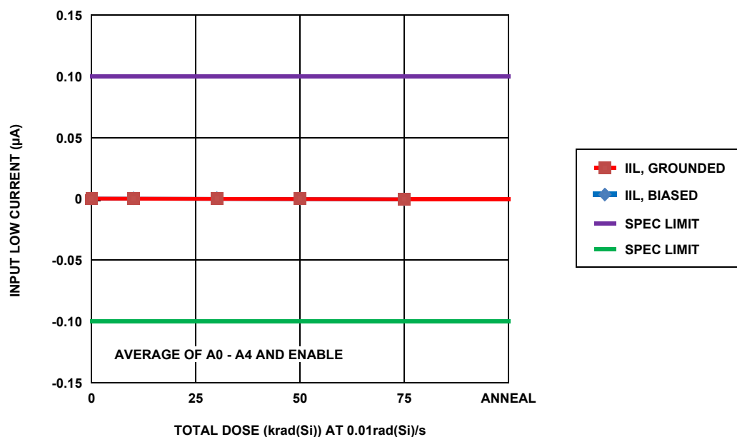
FIGURE 14. ISL71831SEH input LOW current, average of address pins A0 through A4 and Enable pin, as a function of low dose rate total dose irradiation for the unbiased (all pins grounded) and the biased (per Figure 1 ) cases. The dose rate was 8.554mrad(Si)/s to 9.322mrad(Si)/s. Sample size for each of the two cells was 16. The post-irradiation SMD limits are -0.1µA to 0.1µA.
