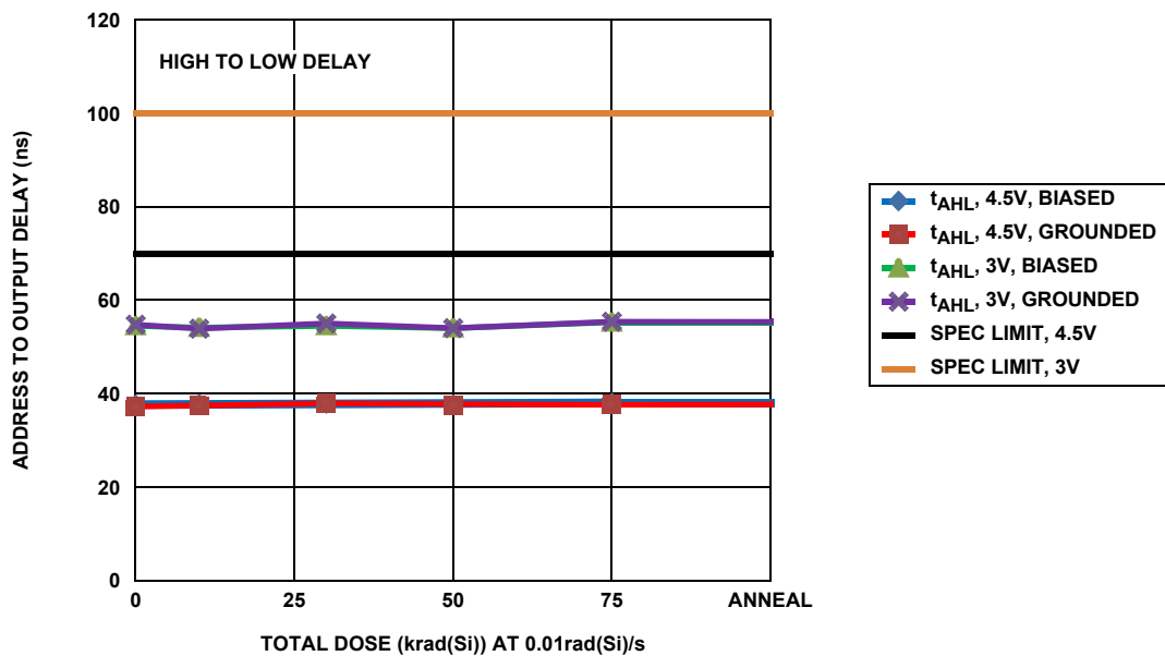
FIGURE 19. ISL71831SEH address input to multiplexer output delay, HIGH to LOW, as a function of low dose rate total dose irradiation for the unbiased (all pins grounded) and the biased (per Figure 1 ) cases. The dose rate was 8.554mrad(Si)/s to 9.322mrad(Si)/s. Sample size for each of the two cells was 16. The post-irradiation SMD limits are 70ns maximum (4.5V) and 100ns maximum (3V).
