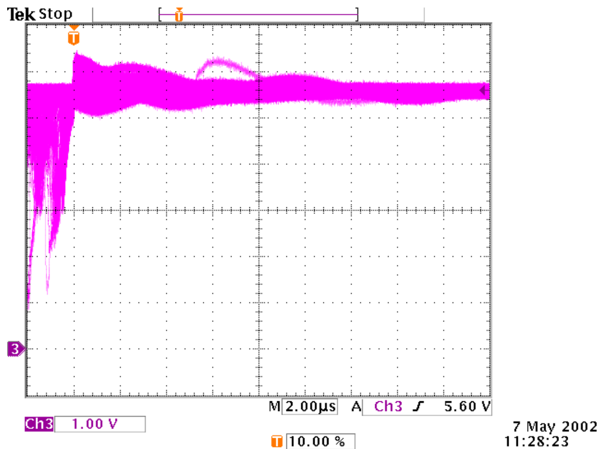
Figure 16: ISL7124SRH SEE response using Kr, LET= 28MeV/mg.cm 2 .
