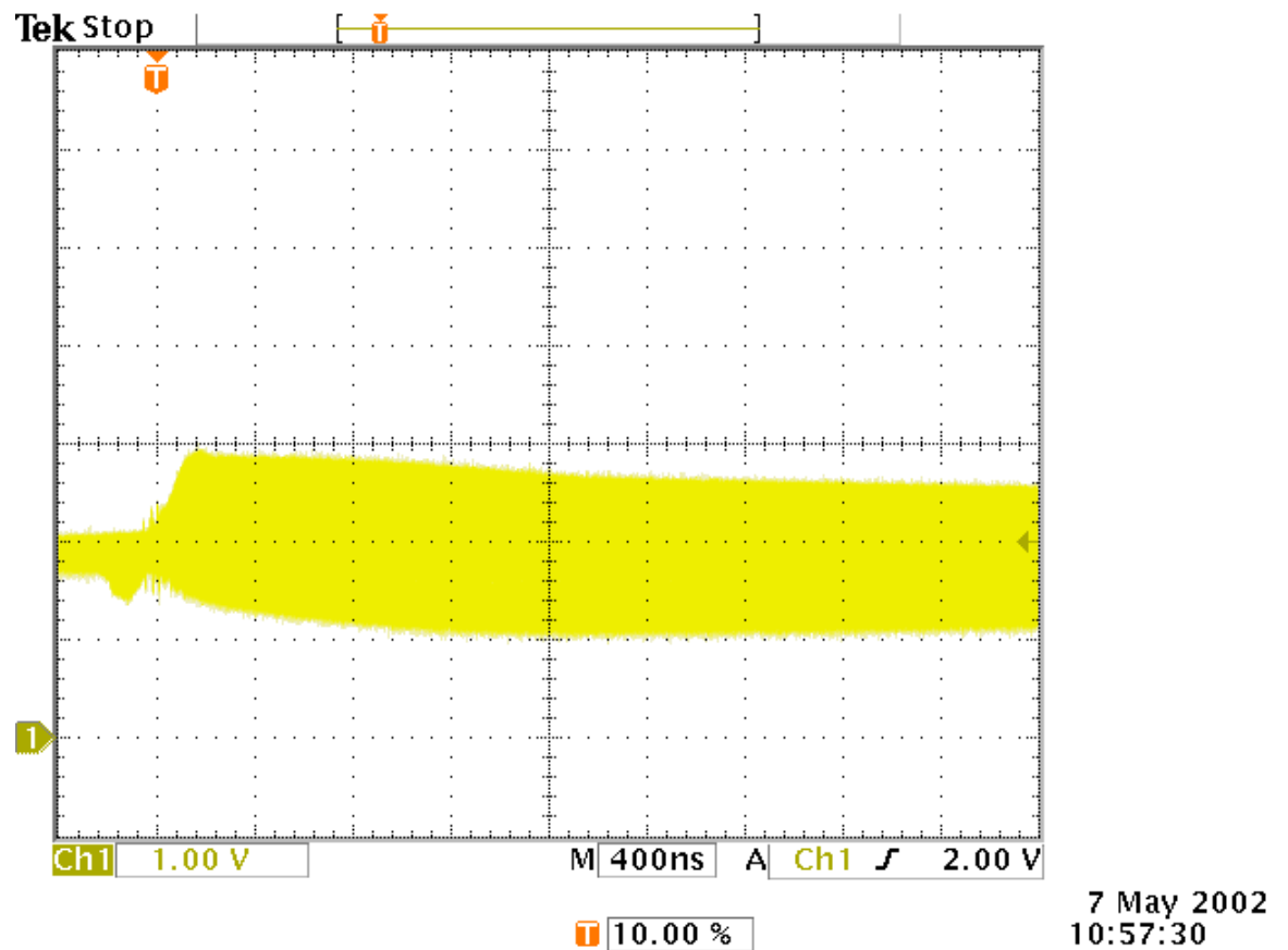
Figure 10: ISL7124SRH SEE response using Kr, LET= 36MeV/mg.cm 2 .
