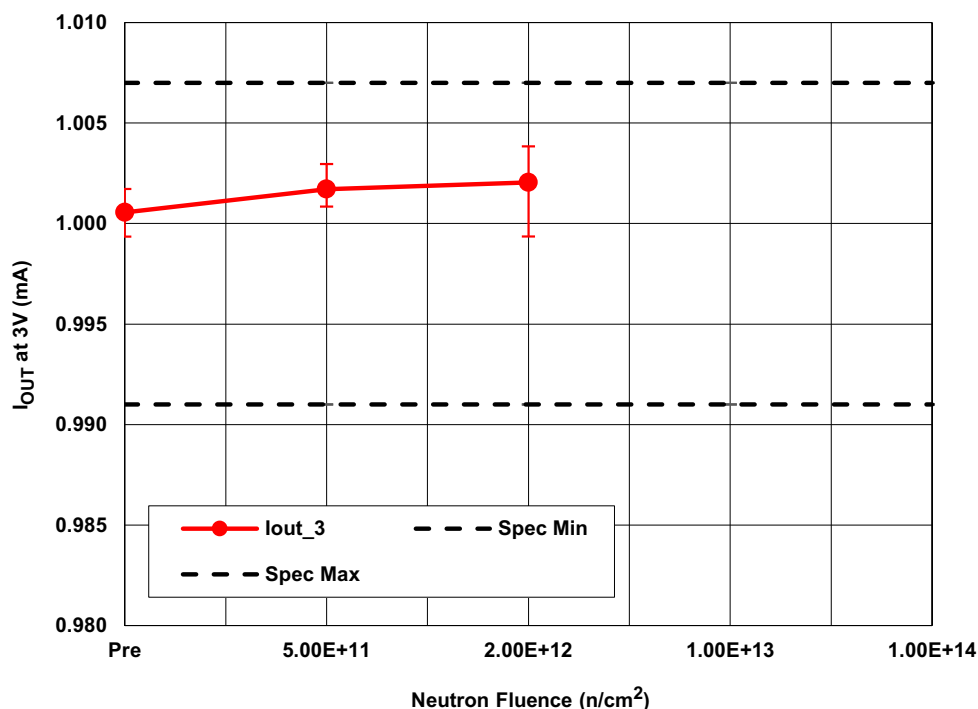
Figure 5. ISL70592SEH output current at 3V ( I_{OUT} ), following irradiation to each neutron fluence level. The error bars represent the minimum and maximum measured values. The 1 \times 10^{13} \text{ n/cm}^2 and 1 \times 10^{14} \text{ n/cm}^2 data are not shown because they could not be accurately measured. The post-irradiation SMD limits are 0.9910mA minimum and 1.0070mA maximum.
