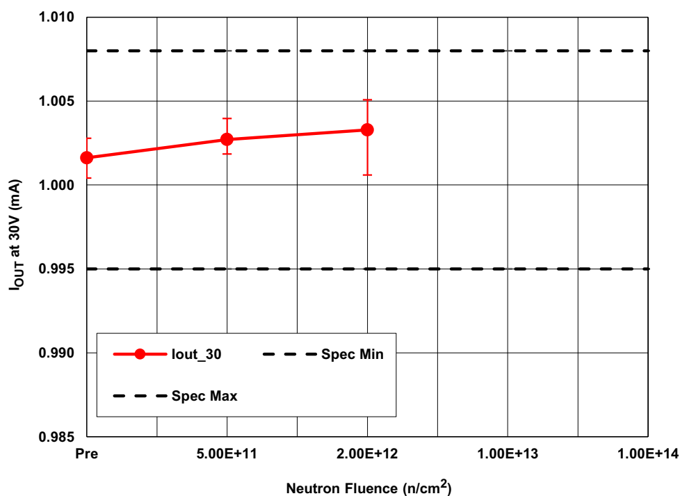
Figure 2. ISL70592SEH output current at 30V ( I_{O30V} ), following irradiation to each neutron fluence level. The error bars represent the minimum and maximum measured values. The 1 \times 10^{13} n/cm^2 and 1 \times 10^{14} n/cm^2 data are not shown because they could not be accurately measured. The post-irradiation SMD limits are 0.9950mA minimum and 1.0080mA maximum.
