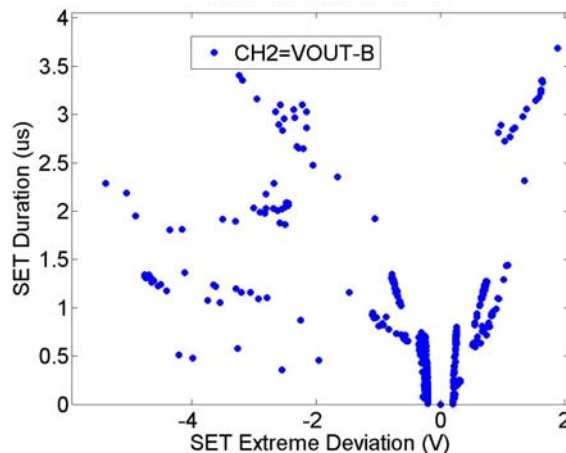
FIGURE 6. DEVICE 6, CHANNEL B, RUN 201, V_S = \pm 5V , LET = 28 \text{ MeV} \cdot \text{cm}^2/\text{mg}
