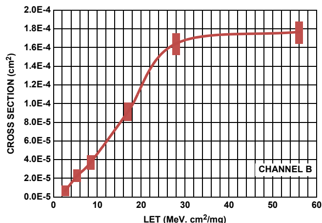
Figure 6. Channel B SET Cross Section vs LET for V_S = \pm 18V with 90% Confidence Level Interval Bars
