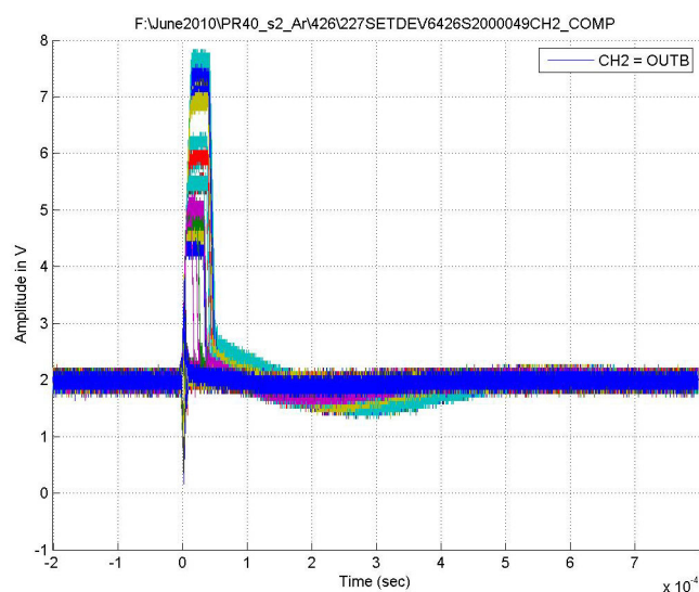
Figure 20. Typical Capture at V_S = \pm 18V , Channel B, LET = 17MeV \cdot cm^2/mg , Run 404
