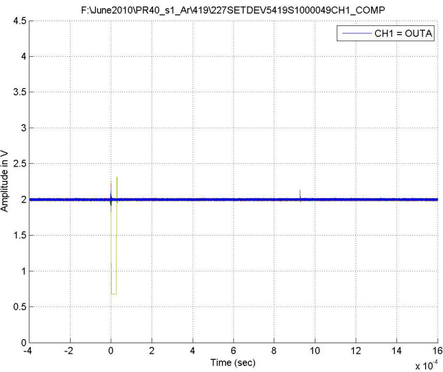
Figure 13. Typical Capture at V_S = \pm 4.5V , Channel A, LET = 8.5MeV \cdot cm^2/mg , Run 419
