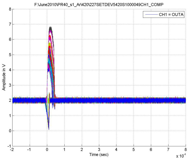
Figure 15. Typical Capture at V_S = \pm 18V , Channel A, LET = 8.5MeV \cdot cm^2/mg^2 , Run 420
