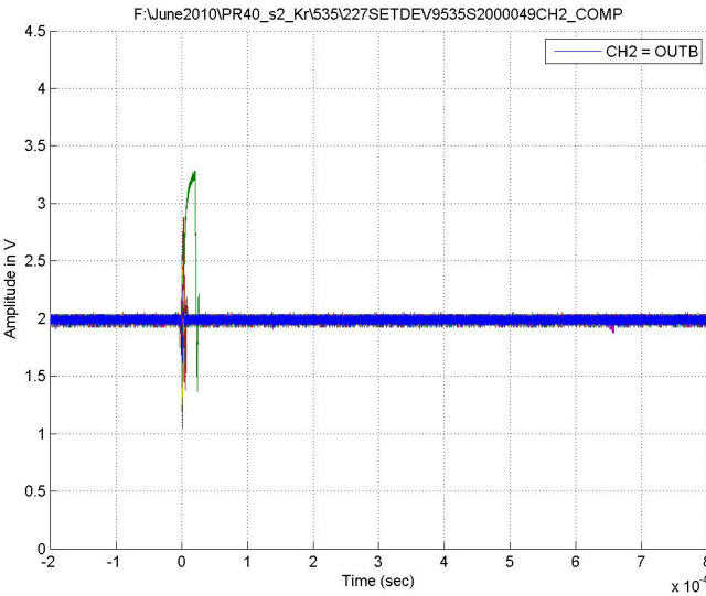
Figure 26. Typical Capture at V_S = \pm 4.5V , Channel B, LET = 56MeV \cdot cm^2/mg , Run 535
