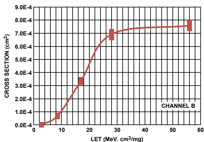
Figure 4. Channel B SET Cross Section vs LET for V_S = \pm 4.5V with 90% Confidence Level Interval Bars
