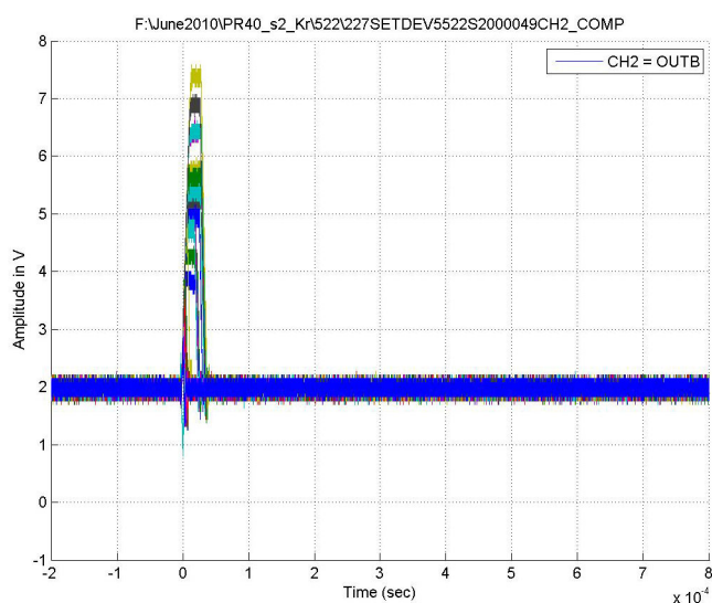
Figure 24. Typical Capture at V_S = \pm 18V , Channel B, LET = 28MeV \cdot cm^2/mg , Run 512
