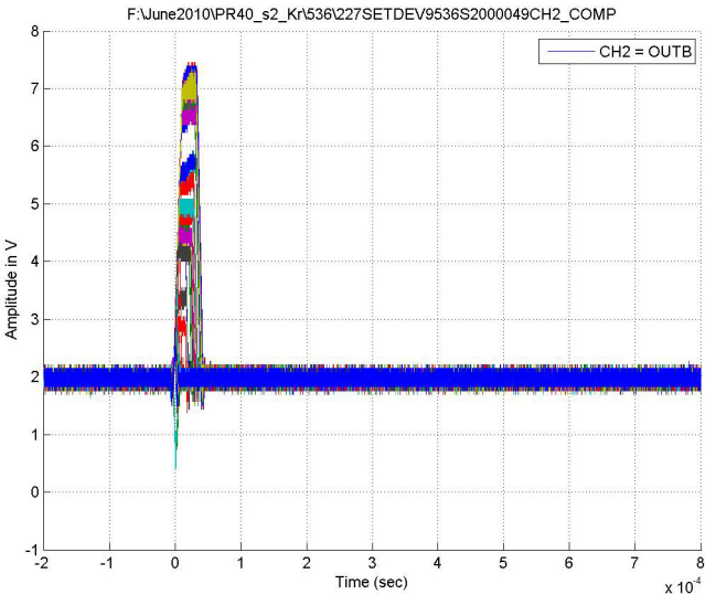
Figure 28. Typical Capture at V_S = \pm 18V , Channel B, LET = 56MeV \cdot cm^2/mg , Run 536
