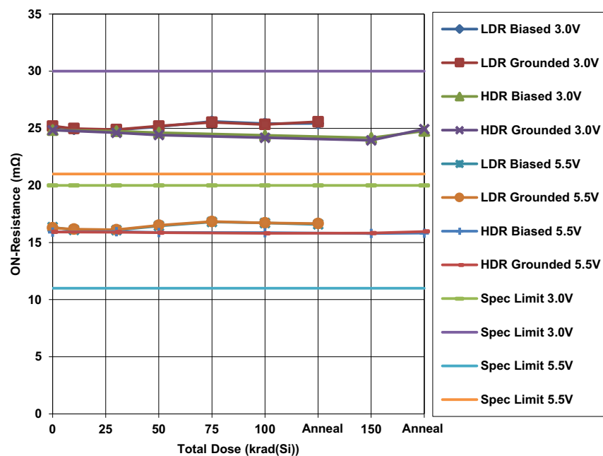
Figure 3. ISL70062SEH switch ON-resistance, 3.0V and 5.5V supply voltage, V_{SWI} = 1.0V , as a function of total dose irradiation at LDR and HDR for the biased and unbiased cases. The irradiations were followed by a high temperature biased anneal at 100°C for 168 hours. The LDR was 0.01rad(Si)/s and the HDR was 72rad(Si)/s. Sample sizes are given in Table 1. The post-irradiation SMD limits are 20mΩ to 30mΩ (3.0V supply) and 11mΩ to 21mΩ (5.5V supply).
