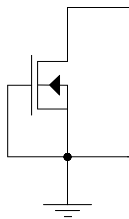
Figure 4. ISL70024SEH TID Bias Schematics (Grounded)
