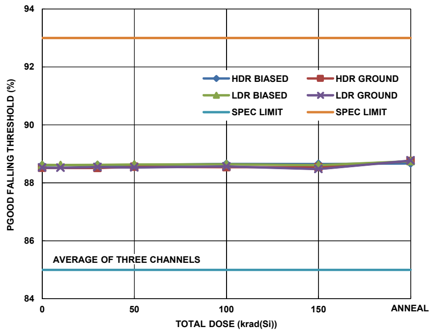
FIGURE 23. ISL70003SEH PG00D falling threshold, average of three channels, as a function of total dose irradiation at low and high dose rate for the unbiased and biased cases. The irradiations were followed by a high temperature biased anneal at 100 °C for 168 hours. The low dose rate was 0.01rad(Si)/s and the high dose rate was 64.9rad(Si)/s. Sample size for each cell was six. The SMD limits are 85% to 93%.
