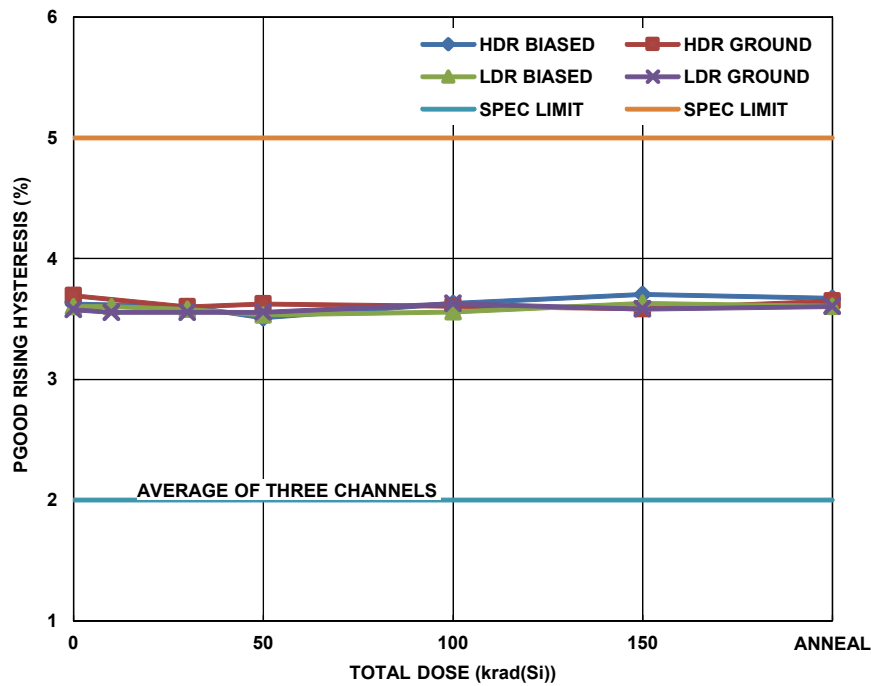
FIGURE 22. ISL70003SEH PG00D rising hysteresis, average of three channels, as a function of total dose irradiation at low and high dose rate for the unbiased and biased cases. The irradiations were followed by a high temperature biased anneal at 100 °C for 168 hours. The low dose rate was 0.01rad(Si)/s and the high dose rate was 64.9rad(Si)/s. Sample size for each cell was six. The SMD limits are 2% to 5%.
