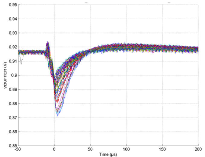
FIGURE 31. BUFFER COMPOSITE SET PLOT, RUN 211, V_{\text{IN}} = 3\text{V}
