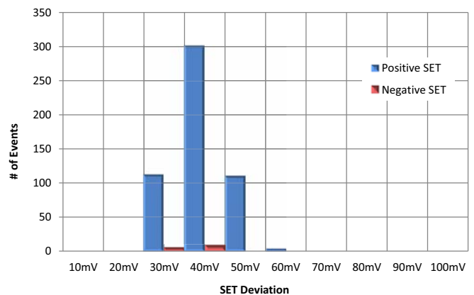
FIGURE 8. HISTOGRAM PLOT FOR RUN 220, f_{SW} = 500\text{kHz} EXTERNAL OSCILLATOR
