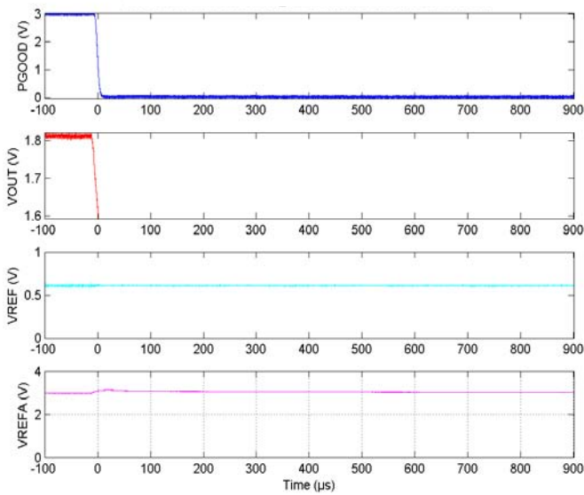
FIGURE 23. SEFI, RUN 204 CAPTURE 2, V_{IN} = 3V
