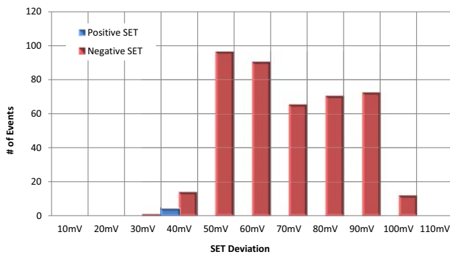
FIGURE 17. HISTOGRAM PLOT FOR RUN 210, f sw = 300kHz INTERNAL OSCILLATOR
