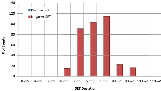
FIGURE 15. HISTOGRAM PLOT FOR RUN 207, f sw = 300kHz INTERNAL OSCILLATOR
