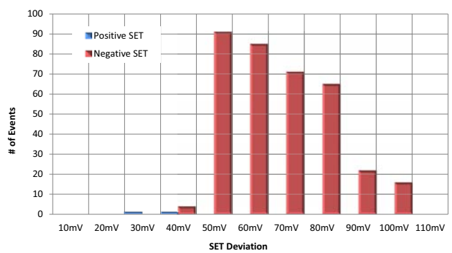
FIGURE 18. HISTOGRAM PLOT FOR RUN 211, f sw = 500kHz EXTERNAL OSCILLATOR
