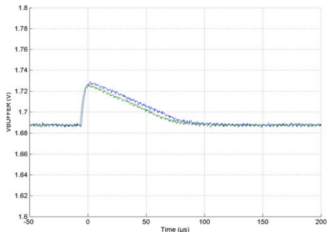
FIGURE 33. BUFFER COMPOSITE SET PLOT, RUN 217, V_{\text{IN}} = 13.2\text{V}
