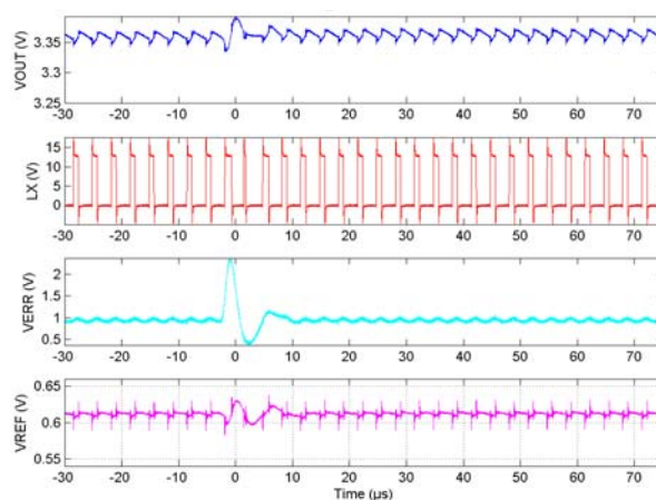
FIGURE 21. POSITIVE SET, RUN 217 CAPTURE 117, V_{IN} = 13.2V
