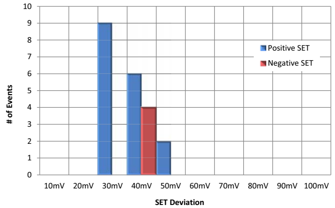
FIGURE 10. HISTOGRAM PLOT FOR RUN 222, f_{SW} = 500\text{kHz} EXTERNAL OSCILLATOR
