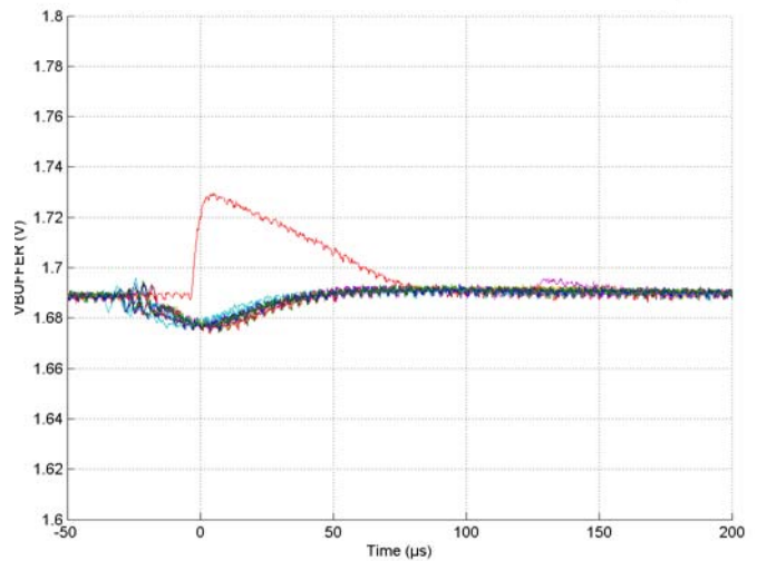
FIGURE 32. BUFFER COMPOSITE SET PLOT, RUN 215, V_{\text{IN}} = 13.2\text{V}
