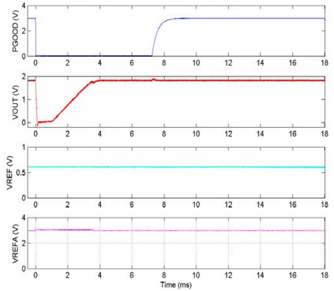
FIGURE 24. SEFI, RUN 208 CAPTURE 1, V_{IN} = 3V
