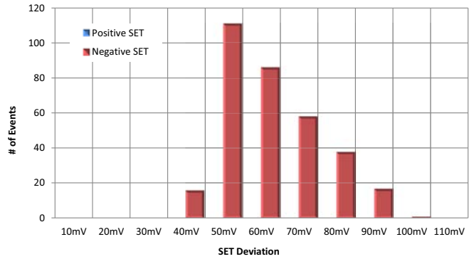
FIGURE 16. HISTOGRAM PLOT FOR RUN 208, f sw = 500kHz EXTERNAL OSCILLATOR
