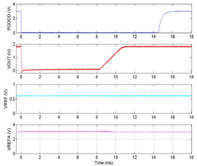
FIGURE 25. SEFI, RUN 204 CAPTURE 1, V_{IN} = 3V
