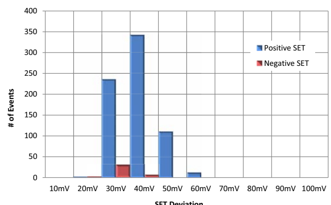
FIGURE 6. HISTOGRAM PLOT FOR RUN 218, f_{SW} = 500\text{kHz} EXTERNAL OSCILLATOR
