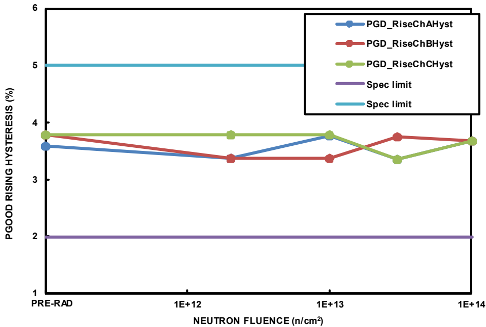
FIGURE 21. ISL70003SEH PG00D rising hysteresis, channels A (blue), B (red) and C (green), as a function of neutron irradiation, showing the median of the populations following irradiation to each level. Neutron fluences and sample sizes (in parentheses) were 2 \times 10^{12} n/cm 2 (5 samples), 1 \times 10^{13} n/cm 2 (5 samples), 3 \times 10^{13} n/cm 2 (5 samples) and 1 \times 10^{14} n/cm 2 (5 samples). The SMD limits are 2% to 5%.
