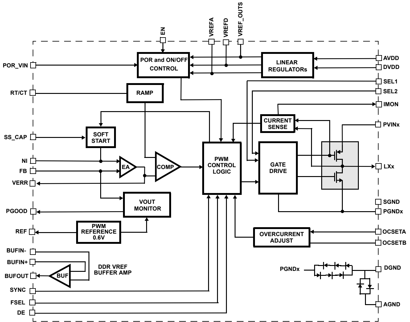
FIGURE 1. BLOCK DIAGRAM
