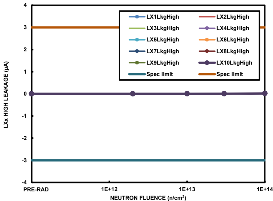
FIGURE 19. ISL70003SEH LXx high leakage current, each of ten power blocks, as a function of neutron irradiation, showing the median of the populations following irradiation to each level. Neutron fluences and sample sizes (in parentheses) were 2 \times 10^{12} n/cm 2 (5 samples), 1 \times 10^{13} n/cm 2 (5 samples), 3 \times 10^{13} n/cm 2 (5 samples) and 1 \times 10^{14} n/cm 2 (5 samples). The SMD limits are -3.0µA to +3.0µA.
