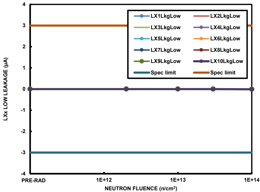
FIGURE 18. ISL70003SEH LXx low leakage current, each of ten power blocks, as a function of neutron irradiation, showing the median of the populations following irradiation to each level. Neutron fluences and sample sizes (in parentheses) were 2 \times 10^{12} n/cm 2 (5 samples), 1 \times 10^{13} n/cm 2 (5 samples), 3 \times 10^{13} n/cm 2 (5 samples) and 1 \times 10^{14} n/cm 2 (5 samples). The SMD limits are -3.0µA to +3.0µA.
