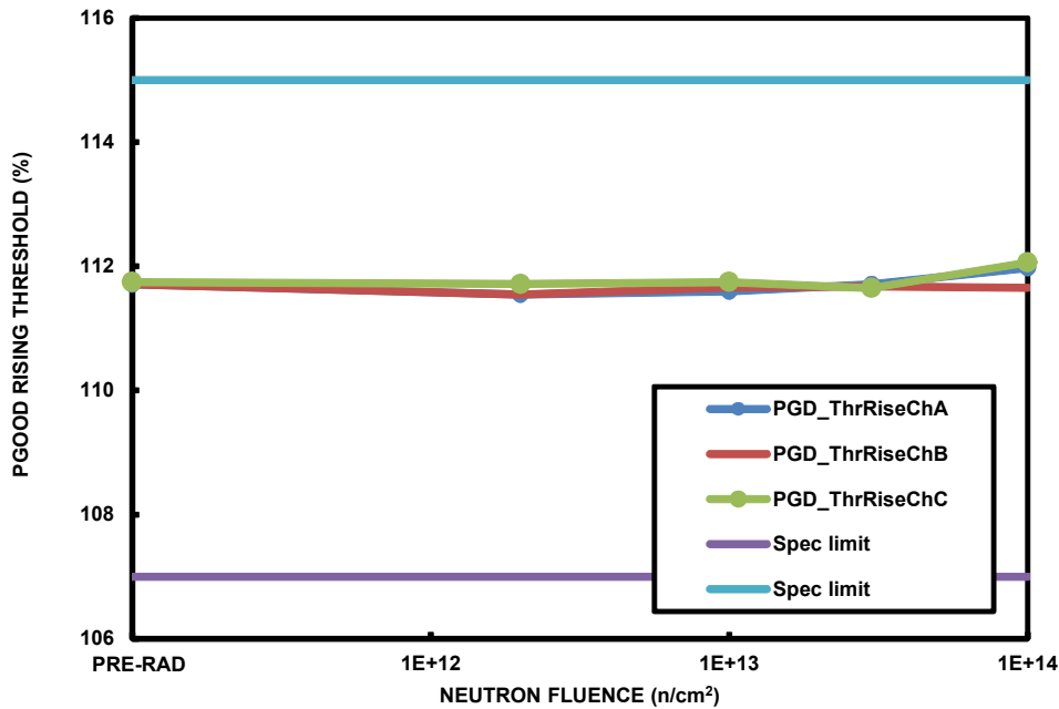
FIGURE 20. ISL70003SEH PG00D rising threshold, channels A (blue), B (red) and C (green), as a function of neutron irradiation, showing the median of the populations following irradiation to each level. Neutron fluences and sample sizes (in parentheses) were 2 \times 10^{12} n/cm 2 (5 samples), 1 \times 10^{13} n/cm 2 (5 samples), 3 \times 10^{13} n/cm 2 (5 samples) and 1 \times 10^{14} n/cm 2 (5 samples). The SMD limits are 107% to 118%.
