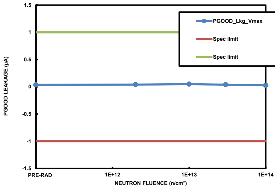
FIGURE 25. ISL70003SEH PGGOOD output leakage, 3V in (blue), as a function of neutron irradiation, showing the median of the populations following irradiation to each level. Neutron fluences and sample sizes (in parentheses) were 2 \times 10^{12} n/cm 2 (5 samples), 1 \times 10^{13} n/cm 2 (5 samples), 3 \times 10^{13} n/cm 2 (5 samples) and 1 \times 10^{14} n/cm 2 (5 samples). The SMD limits are -1.0µA to +1.0µA.
