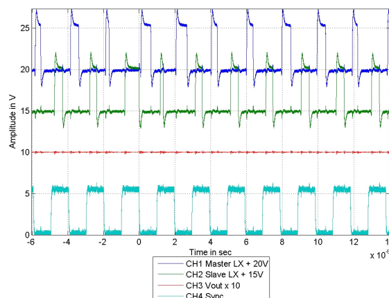
Figure 9. ISL70002SEH SET signature at LET = 86MeV·cm 2 /mg. The part is operated as a 2-phase converter at 5.5V input, with the Master irradiated. The trace colors and scale factors are as in Figure 4. The Master trace shows one narrowed LX pulse; this is followed by a wide Slave pulse and recovery of the converter. Output voltage change is less than -1%.
