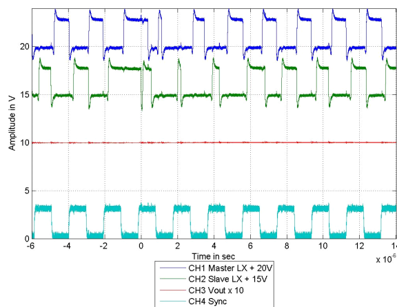
Figure 7. ISL70002SEH SET signature at LET = 86\text{MeV}\cdot\text{cm}^2/\text{mg} . The part is operated as a 2-phase converter at 3.0V input, with the Slave irradiated. The trace colors and scale factors are as in Figure 4. The Slave trace shows one wide LX pulse followed by narrow pulses and recovery of the converter. The output voltage change is less than -1%.
