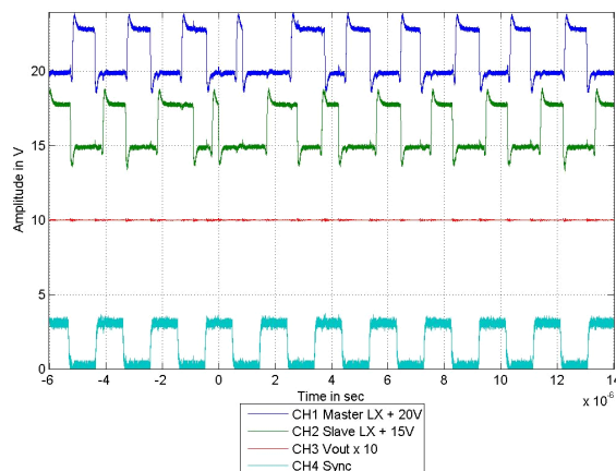
Figure 5. ISL70002SEH SET signature at LET = 86MeV•cm 2 /mg. The part is operated as a 2-phase converter at 3.0V input, with the Master irradiated. The trace colors and scale factors are as in Figure 4. Both the Master and Slave traces show one narrowed LX pulse followed by a wide pulse and recovery of the converter. The output voltage perturbation (red trace) is less than -1%.
