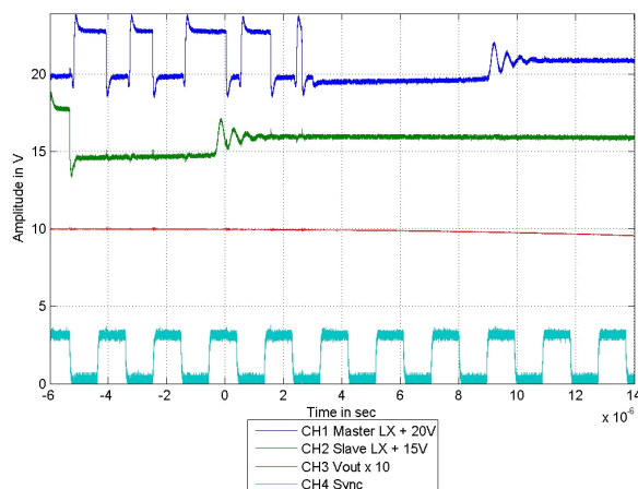
Figure 16. ISL70002SEH SEFI signature at LET = 86\text{MeV}\cdot\text{cm}^2/\text{mg} . The part is operated as a 2-phase converter at 3.0V input, with the Slave irradiated. The trace colors and scale factors are as in Figure 4. The Slave tri-states and alerts the Master which also tri-states. As each LX output tri-states, the current through each inductor decays to zero, the LX output rises to V_{OUT} and the part initiates a soft-start (SS) sequence; see the compressed time scale plot in Figure 18.
