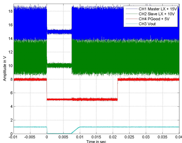
Figure 18. Compressed scale ISL70002SEH SEFI signature at LET = 86\text{MeV}\cdot\text{cm}^2/\text{mg} . The part is operated as a 2-phase converter at 3.0V input, with the Slave irradiated. The two upper traces show the Master (blue) and Slave (green) LX output waveforms. The lower trace (aqua) is the output voltage of the converter, and the red trace is the PGOOD output signal. Both LX outputs tri-state, and the part goes through a hiccup cycle followed by a normal soft-start without external intervention. Note: The horizontal axis is calibrated at 5ms per division.
