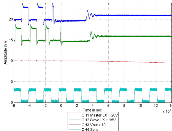
Figure 13. ISL70002SEH SEFI signature at LET = 86MeV·cm 2 /mg. The part is operated as a 2-phase converter at 3.0V input, with the Master irradiated. The trace colors and scale factors are as in Figure 4. Both LX outputs tri-state, the current through the inductor decays to zero, the LX output rises to V OUT and the part initiates a soft-start (SS) sequence; see the compressed time scale plots in Figure 14 and Figure 15 as examples.
