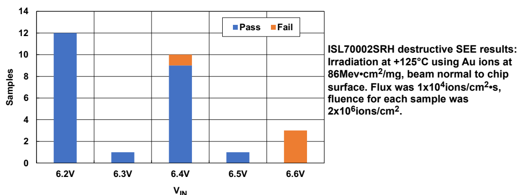
Figure 3. Summary of ISL70002SEH destructive SEE test results. [1]
