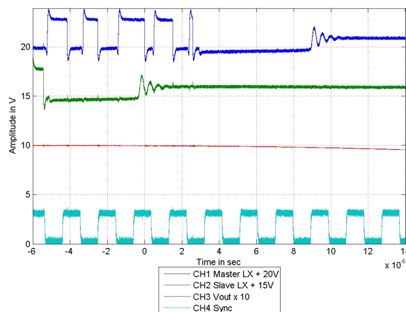
Figure 17. ISL70002SEH SEFI signature at LET = 86\text{MeV}\cdot\text{cm}^2/\text{mg} . The part is operated as a 2-phase converter at 3.0V input, with the Slave irradiated. The trace colors and scale factors are as in Figure 4. Both LX outputs tri-state, the current through the inductor decays to zero, the LX output rises to V_{OUT} and the part initiates a soft-start (SS) sequence; see the compressed time scale plot in Figure 18 as an example.
