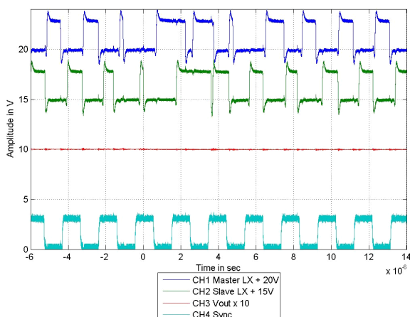
Figure 6. ISL70002SEH SET signature at LET = 86\text{MeV}\cdot\text{cm}^2/\text{mg} . The part is operated as a 2-phase converter at 3.0V input, with the Slave irradiated. The trace colors and scale factors are as in Figure 4. The Master and Slave traces show one narrow LX pulse followed by a wide pulse and recovery of the converter. Output voltage change is less than -1%.
