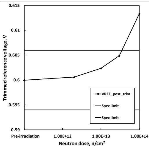
Fig. 13: ISL70001SRH trimmed reference voltage as a function of neutron irradiation. Sample size was 5 for each cell ( 2 \times 10^{12} n/cm 2 , 1 \times 10^{13} n/cm 2 , 3 \times 10^{13} n/cm 2 and 1 \times 10^{14} n/cm 2 ), with three control units. The data sheet limits are 0.594V to 0.606V.
