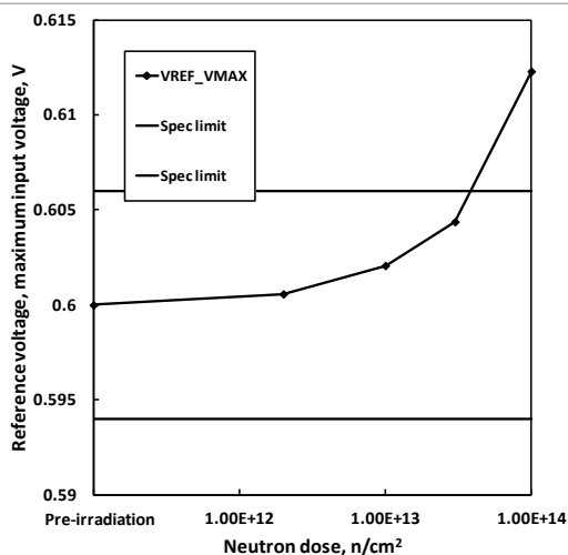
Fig. 16: ISL70001SRH reference output voltage, 5.5V in, as a function of neutron irradiation. Sample size was 5 for each cell ( 2 \times 10^{12} n/cm 2 , 1 \times 10^{13} n/cm 2 , 3 \times 10^{13} n/cm 2 and 1 \times 10^{14} n/cm 2 ), with three control units. The data sheet limits are 0.594V to 0.606V.
