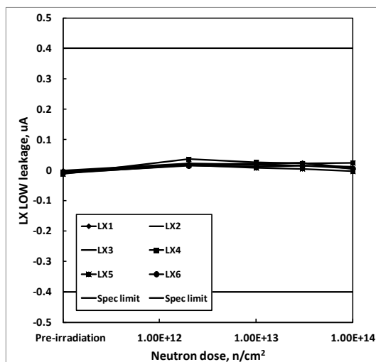
Fig. 11: ISL70001SRH LX LOW leakage current, all six LX outputs, as a function of neutron irradiation. Sample size was 5 for each cell ( 2 \times 10^{12} n/cm 2 , 1 \times 10^{13} n/cm 2 , 3 \times 10^{13} n/cm 2 and 1 \times 10^{14} n/cm 2 ), with three control units. The data sheet limits are -0.4uA to +0.4uA.
