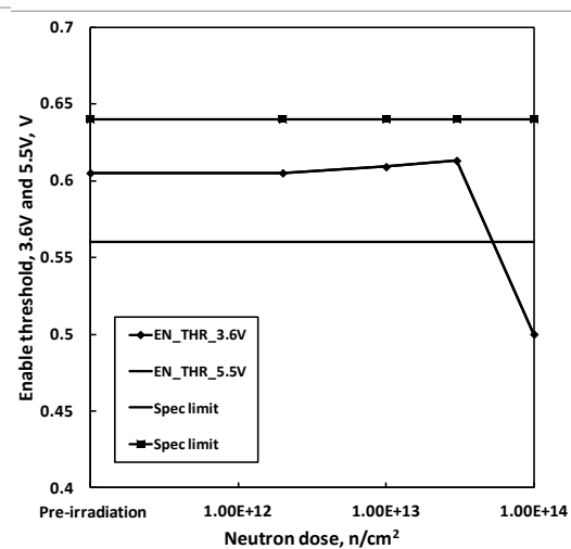
Fig. 33: ISL70001SRH ENABLE threshold, 3.6V and 5.5V in, as a function of neutron irradiation. Sample size was 5 for each cell ( 2 \times 10^{12} n/cm 2 , 1 \times 10^{13} n/cm 2 , 3 \times 10^{13} n/cm 2 and 1 \times 10^{14} n/cm 2 ). The data sheet limits are 0.56V to 0.64V.
