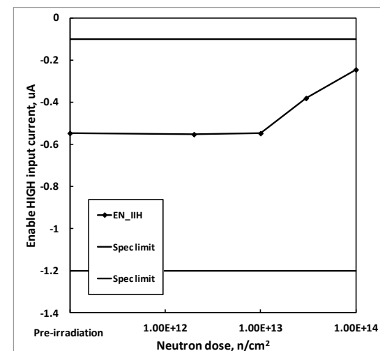
Fig. 3: ISL70001SRH enable HIGH input current as a function of neutron irradiation. Sample size was 5 for each cell ( 2 \times 10^{12} n/cm 2 , 1 \times 10^{13} n/cm 2 , 3 \times 10^{13} n/cm 2 and 1 \times 10^{14} n/cm 2 ), with three control units. The data sheet limits are -1.2uA to -0.1uA.
