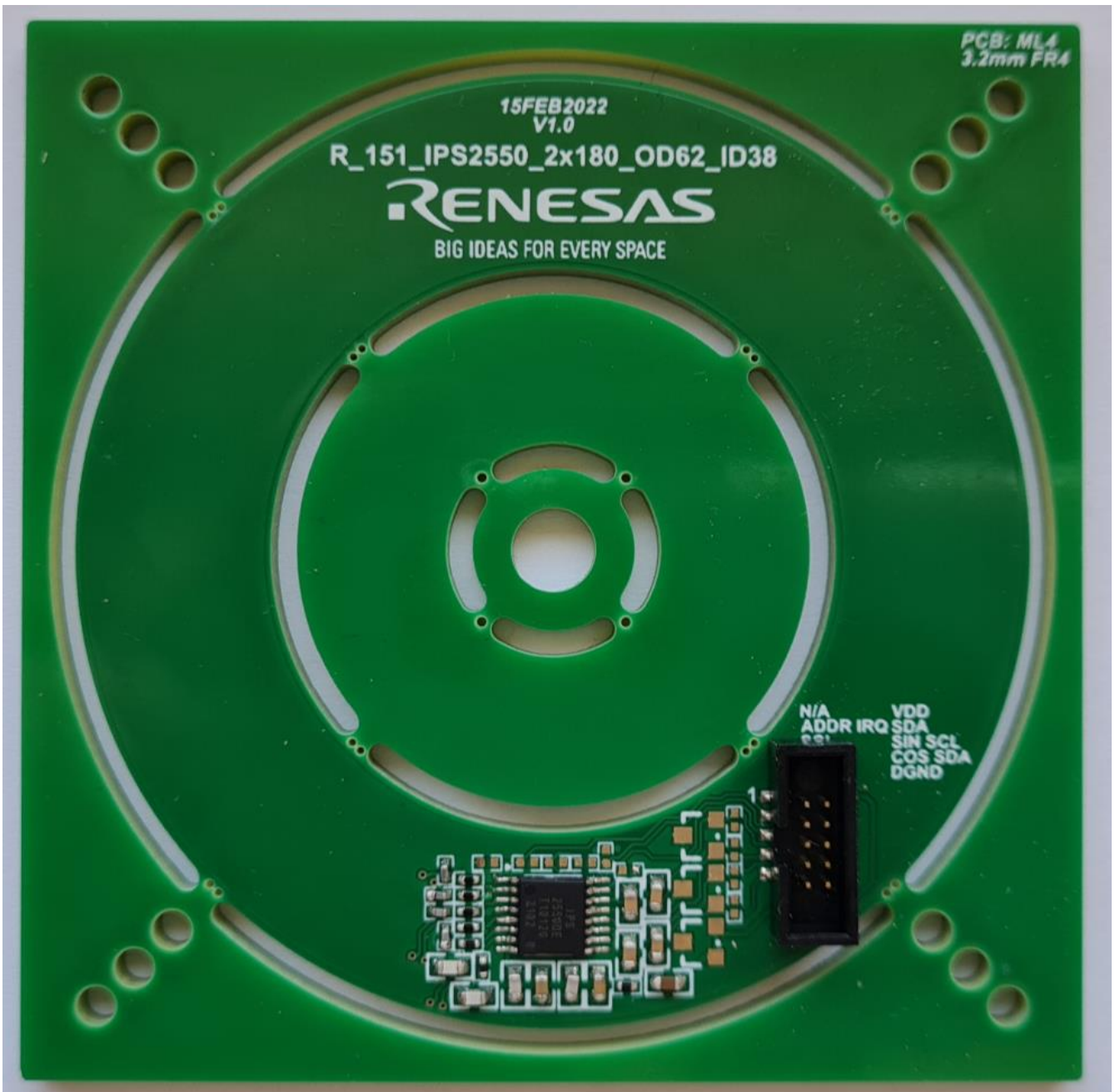
Figure 1. Sensor Board
