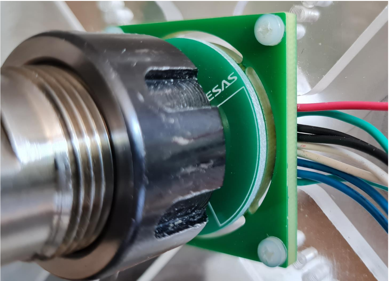
Figure 3. Setup
