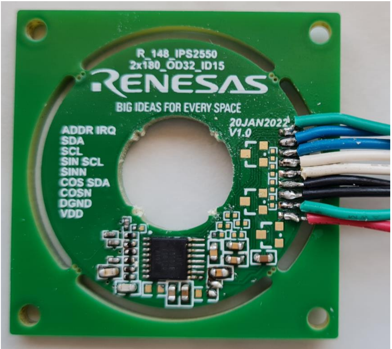
Figure 1. Sensor Board
