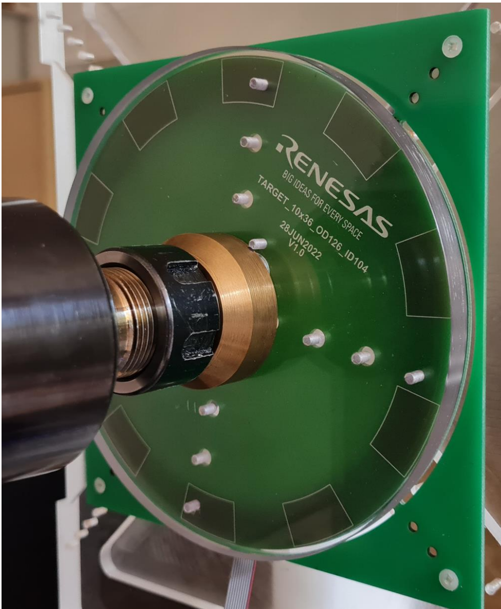
Figure 3. Setup
