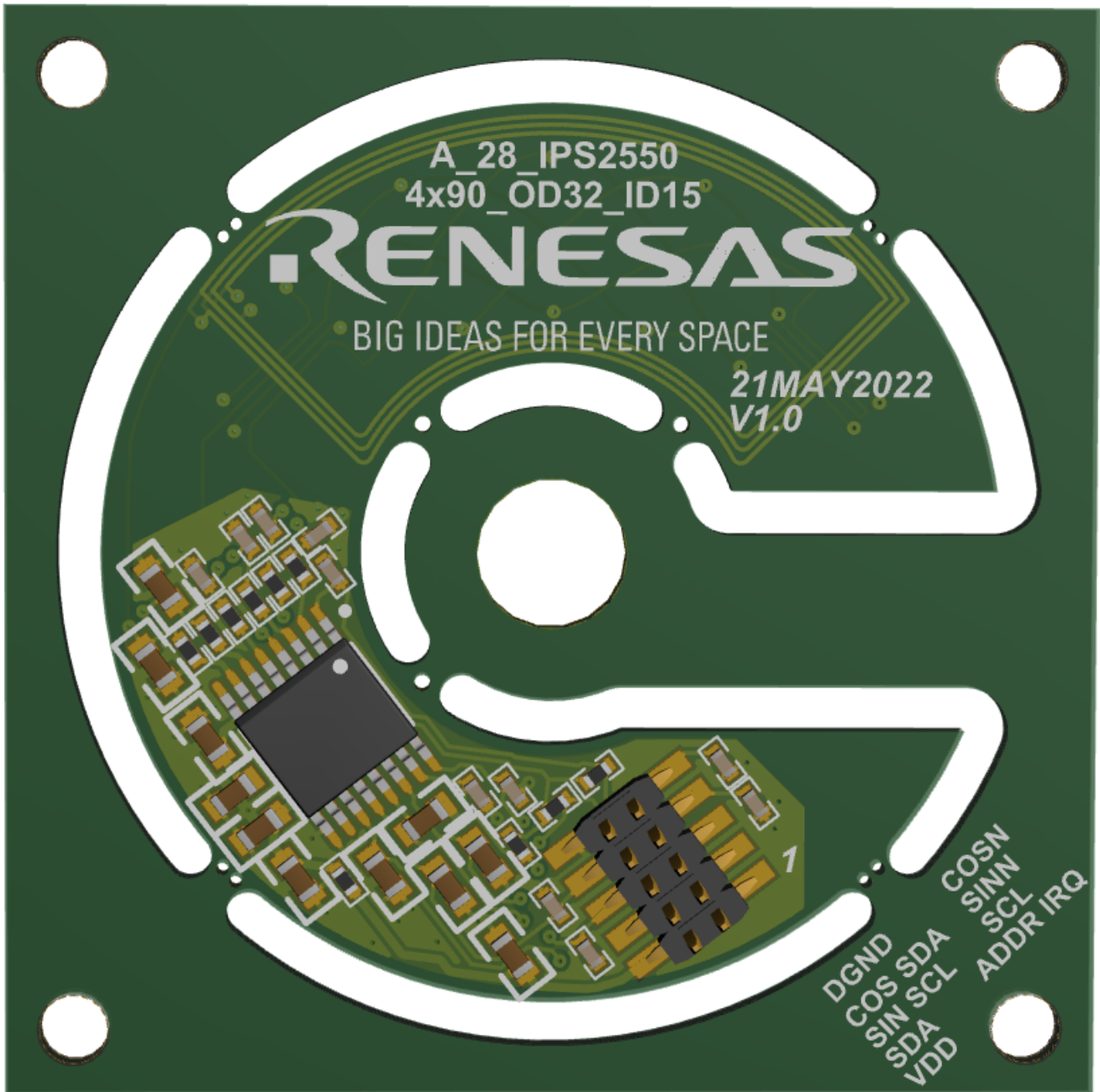
Figure 1. Sensor Board
