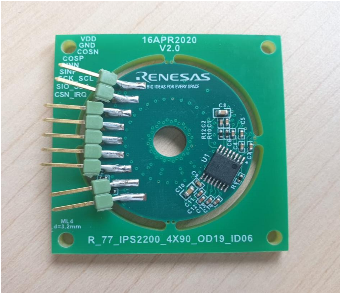
Figure 1. Sensor Board
