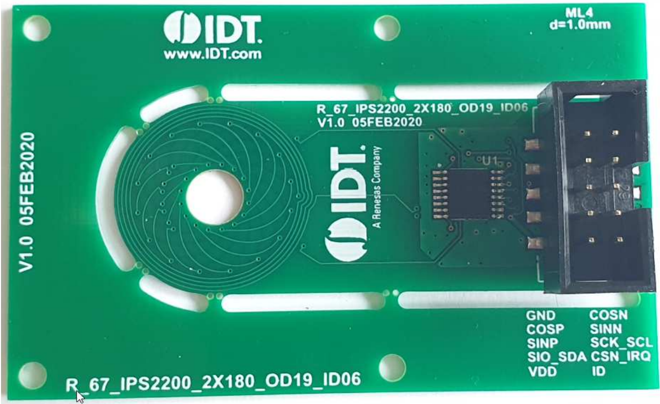
Figure 1. Sensor Board
