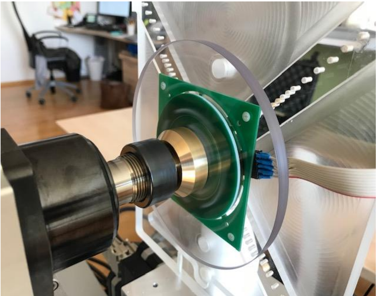
Figure 3. Setup
