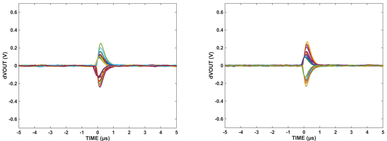
Figure 7. Composite extreme SET (20 most positive, 20 most negative, 20 longest duration outside \pm 80mV ) plots for CH1 at LET = 2.5 MeV \cdot cm^2/mg and DUT7 at \pm 5V (left) and DUT8 at \pm 15V (right)
