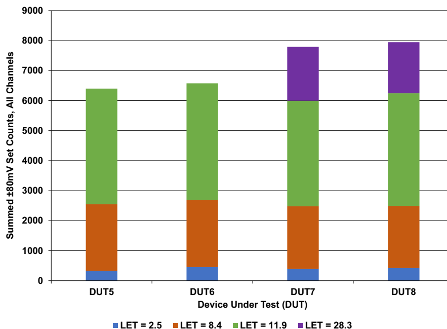
Figure 2. \pm 80\text{mV} SET Counts Summed for All Channels by DUT and Effective LET for Supplies of \pm 15\text{V}
