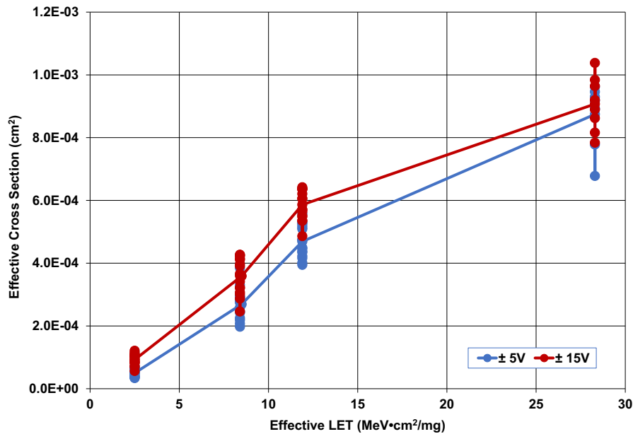
Figure 4. HS-OP470ARH \pm 80\text{mV} SET cross sections for all channels and all parts. Four parts are included for an effective LET of 2.5, 8.4, and 11.9\text{MeV}\cdot\text{cm}^2/\text{mg} , but only two parts are included for \text{LET} = 28.3\text{MeV}\cdot\text{cm}^2/\text{mg} . The lines connect the mean cross sections. The parts were configured as a non-inverting buffer with a gain of 11 and biased with an input of +0.2\text{V} .
