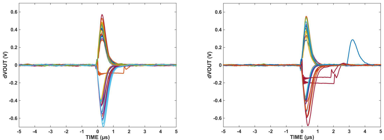
Figure 5. Composite extreme SET (20 most positive, 20 most negative, 20 longest duration outside \pm 80\text{mV} ) plots for CH1 at \text{LET} = 28.3\text{MeV}\cdot\text{cm}^2/\text{mg} and \pm 15\text{V} for DUT7 (left) and DUT8 (right)
