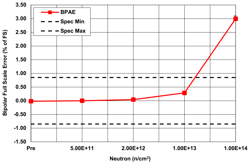
Figure 10. HS-565BxH bipolar full scale error (BPAE) with V_{CC} = +15V , V_{EE} = -15V , following irradiation to each level. The error bars (if visible) represent the minimum and maximum measured values. The post-irradiation SMD limits are -0.85% of F.S minimum and 0.85% of F.S. maximum.
