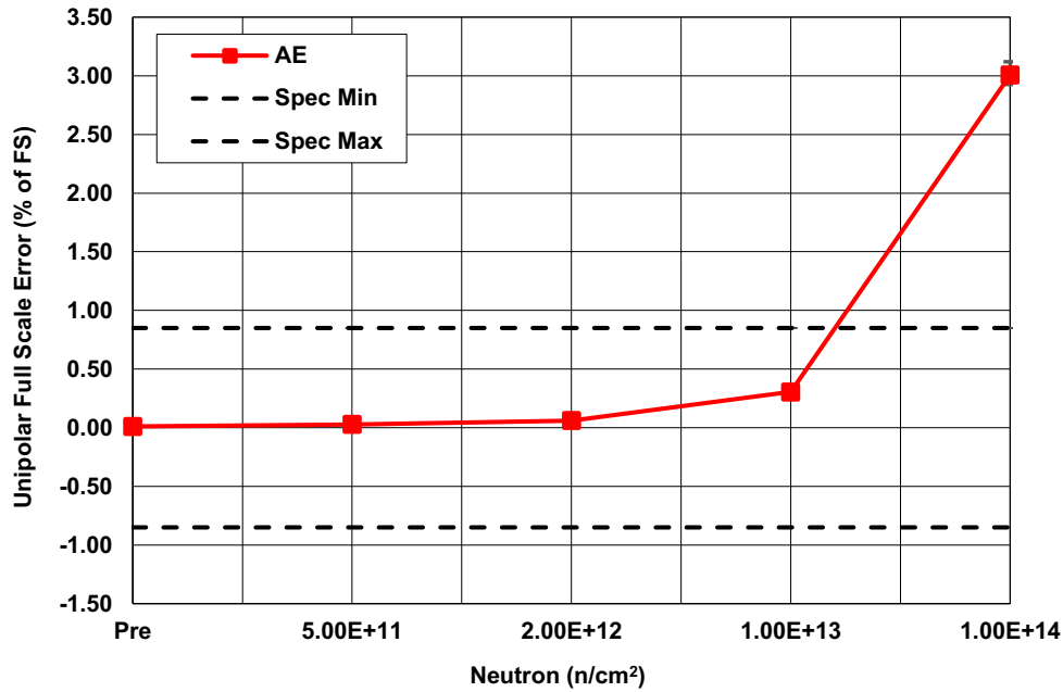
Figure 9. HS-565BxH unipolar full scale error (AE) with V_{CC} = +15V , V_{EE} = -15V , following irradiation to each level. The error bars (if visible) represent the minimum and maximum measured values. The post-irradiation SMD limits are -0.85% of F.S minimum and 0.85% of F.S. maximum.
