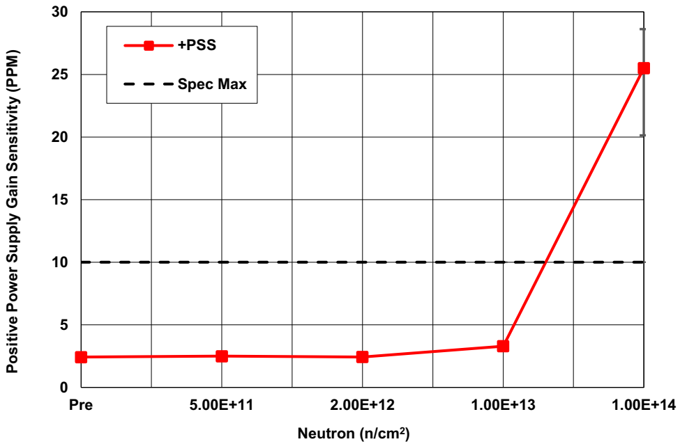
Figure 14. HS-565BxH positive power supply gain sensitivity (+PSS) with V_{CC} = +15V , V_{EE} = -15V , following irradiation to each level. The error bars (if visible) represent the minimum and maximum measured values. The post-irradiation SMD limit is 10(PPM \text{ of full scale})/(\% \Delta V_{CC}) maximum.
