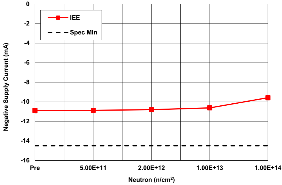
Figure 3. HS-565BxH negative power supply current ( I_{EE} ) with V_{CC} = +15V , V_{EE} = -15V , following irradiation to each level. The error bars (if visible) represent the minimum and maximum measured values. The post-irradiation SMD limit is -14.5mA minimum.
