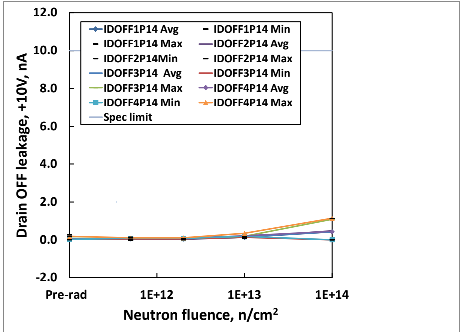
Fig. 8: HS-201HSRH drain OFF leakage at +10.0V as a function of neutron irradiation, each channel, showing the mean, minimum and maximum of the populations at each level. Sample size was 5 for each cell ( 5 \times 10^{11} n/cm 2 , 2 \times 10^{12} n/cm 2 , 1 \times 10^{13} n/cm 2 and 1 \times 10^{14} n/cm 2 ), with two control units. The post-irradiation SMD limit is +10.0nA maximum.
