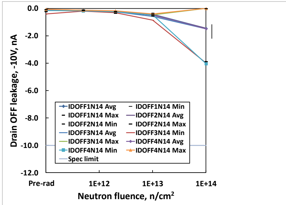
Fig. 9: HS-201HSRH drain OFF leakage at -10.0V as a function of neutron irradiation, each channel, showing the mean, minimum and maximum of the populations at each level. Sample size was 5 for each cell ( 5 \times 10^{11} n/cm 2 , 2 \times 10^{12} n/cm 2 , 1 \times 10^{13} n/cm 2 and 1 \times 10^{14} n/cm 2 ), with two control units. The post-irradiation SMD limit is -10.0nA maximum.
