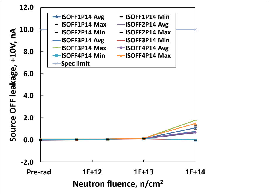
Fig. 6: HS-201HSRH source OFF leakage at +10.0V as a function of neutron irradiation, each channel, showing the mean, minimum and maximum of the populations at each level. Sample size was 5 for each cell ( 5 \times 10^{11} n/cm 2 , 2 \times 10^{12} n/cm 2 , 1 \times 10^{13} n/cm 2 and 1 \times 10^{14} n/cm 2 ), with two control units. The post-irradiation SMD limit is +10.0nA maximum.
