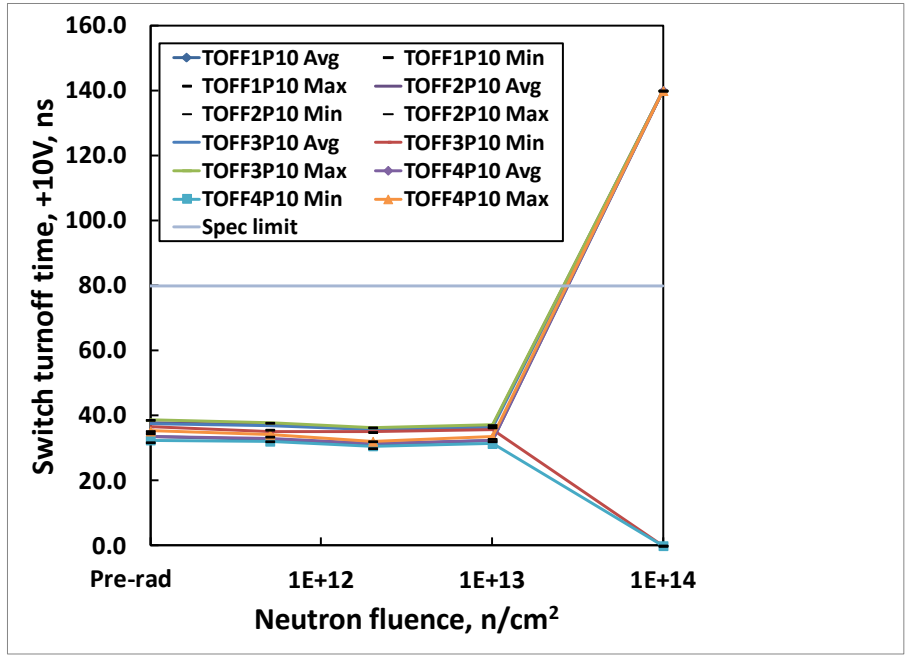
Fig. 14: HS-201HSRH switch turnoff time at +10.0V as a function of neutron irradiation, each channel, showing the mean, minimum and maximum of the populations at each level. Sample size was 5 for each cell ( 5 \times 10^{11} n/cm 2 , 2 \times 10^{12} n/cm 2 , 1 \times 10^{13} n/cm 2 and 1 \times 10^{14} n/cm 2 ), with two control units. The post-irradiation SMD limit is 80.0ns maximum.
