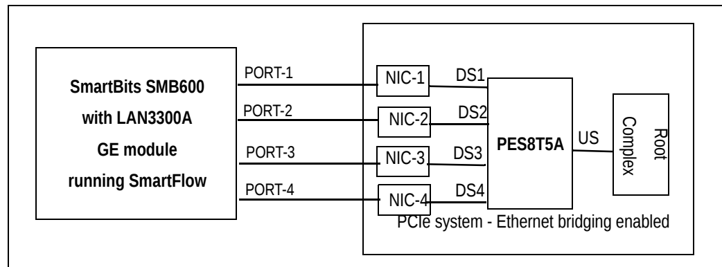
Figure 2 GE Throughput Measurement Setup with the PES8T5A
