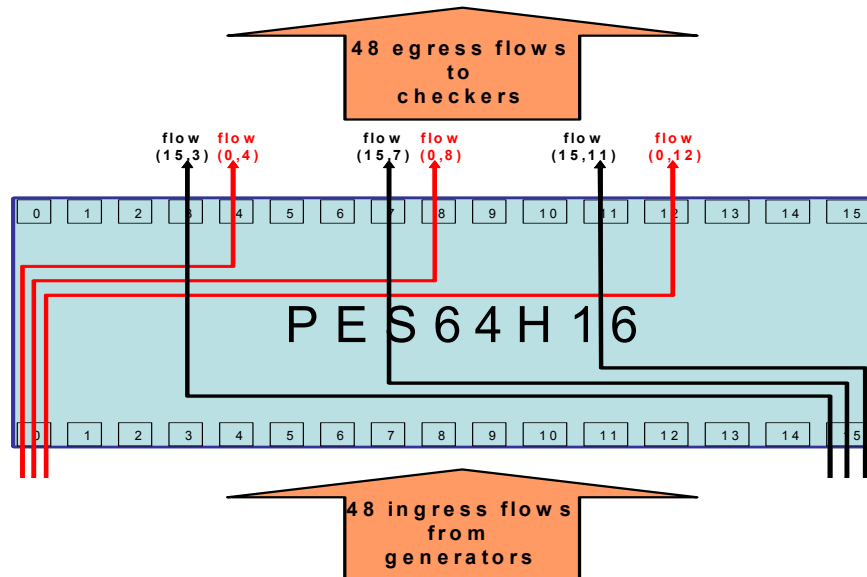
Figure 7 Traffic pattern through the DUT
