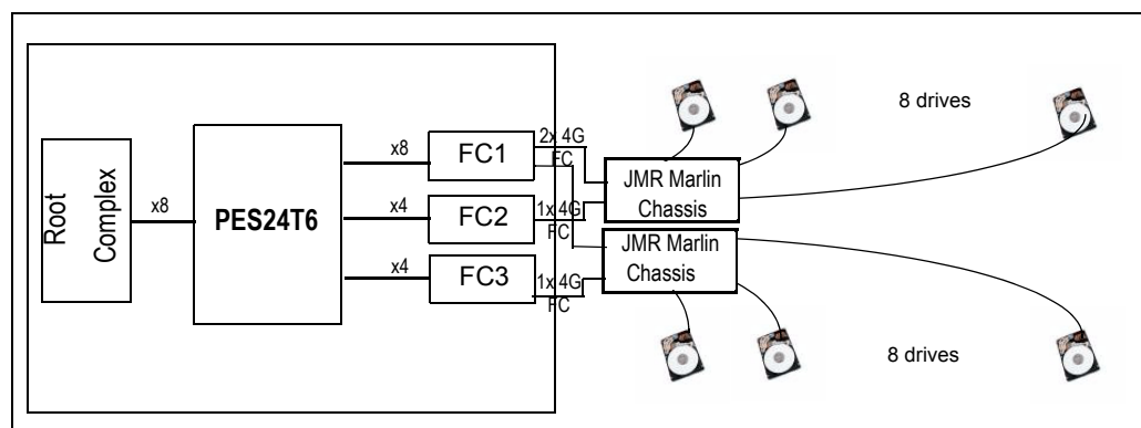
Figure 7 FC Throughput Measurement Setup with the PES24T6
