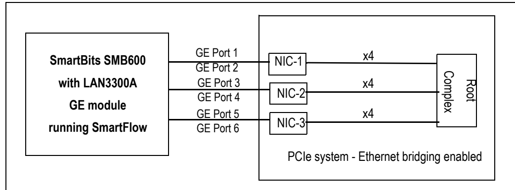
Figure 6 GE Throughput Measurement Setup without the PES24T6
