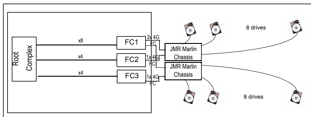
Figure 8 FC Throughput Measurement without the PES24T6
