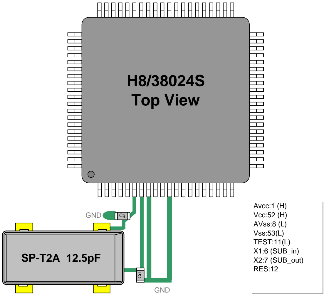
Figure 1 Referencial components layout
