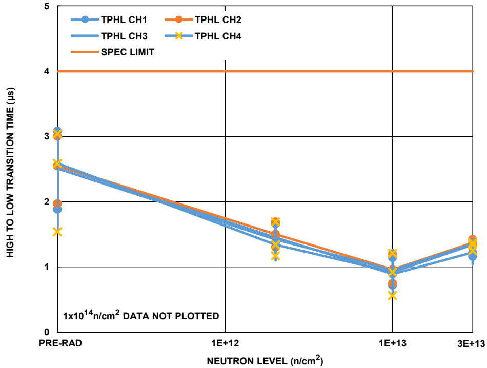
Figure 16. IS-139ASRH HIGH to LOW response time, V_{OD} = V_{IO} + 5mV , each of four channels, as a function of 1MeV equivalent neutron irradiation at 2 \times 10^{12} n/cm^2 , 1 \times 10^{13} n/cm^2 and 3 \times 10^{13} n/cm^2 . All samples were nonfunctional after 1 \times 10^{14} n/cm^2 and that data is not plotted. The plot shows the population median, minimum and maximum at each datapoint. Sample size for each cell was 5. The post-total dose irradiation SMD limit is 4\mu s maximum.
