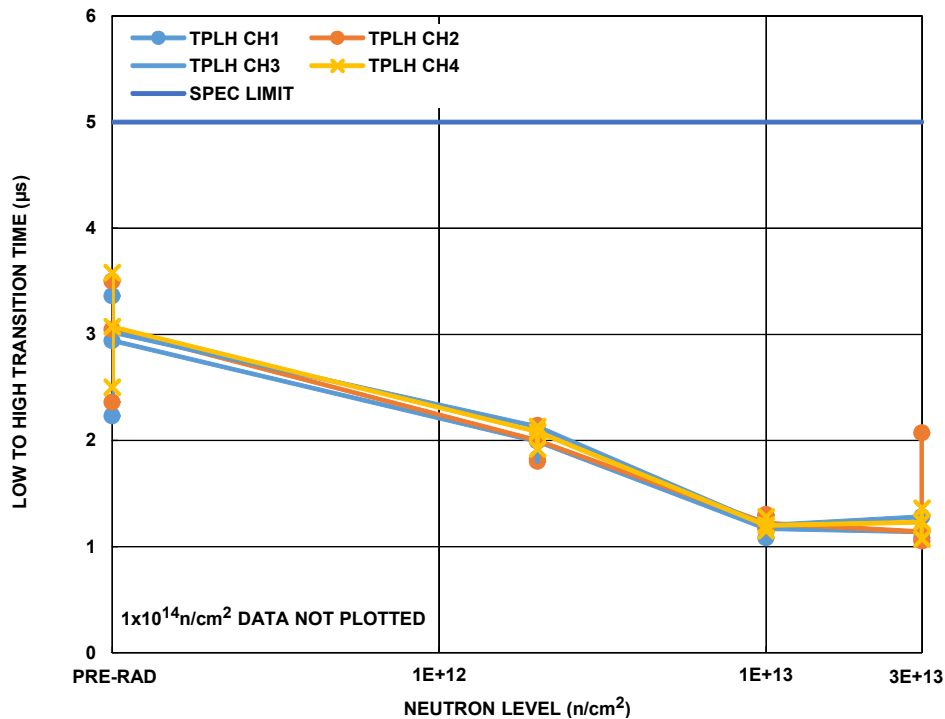
Figure 17. IS-139ASRH LOW to HIGH response time, V_{OD} = V_{IO} + 5mV , each of four channels, as a function of 1MeV equivalent neutron irradiation at 2 \times 10^{12} n/cm^2 , 1 \times 10^{13} n/cm^2 and 3 \times 10^{13} n/cm^2 . All samples were nonfunctional after 1 \times 10^{14} n/cm^2 and that data is not plotted. The plot shows the population median, minimum and maximum at each datapoint. Sample size for each cell was 5. The post-total dose irradiation SMD limit is 5\mu s maximum.
