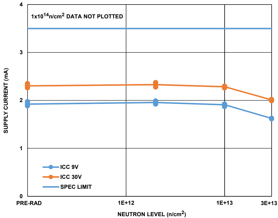
Figure 1. IS-139ASRH supply current for the 9V and 30V supply cases, as a function of 1MeV equivalent neutron irradiation at 2 \times 10^{12} \text{ n/cm}^2 , 1 \times 10^{13} \text{ n/cm}^2 and 3 \times 10^{13} \text{ n/cm}^2 . All samples were nonfunctional after 1 \times 10^{14} \text{ n/cm}^2 and that data is not plotted. The plot shows the population median, minimum and maximum at each downpoint. Sample size for each cell was 5. The post-total dose irradiation SMD limit is 3.5mA maximum.
