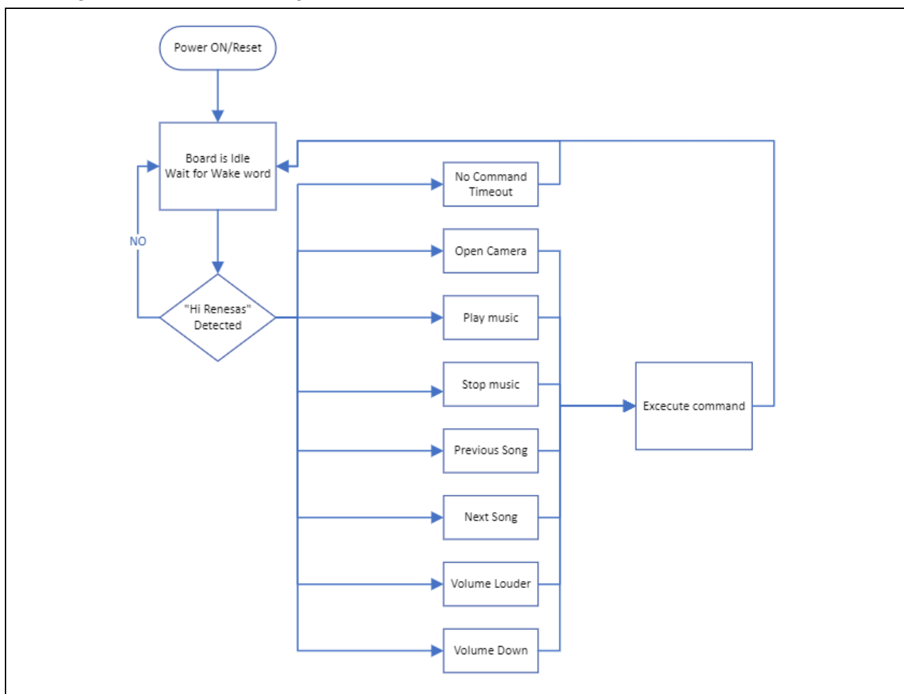
Figure 2. Quick Start Guide Project Flow
