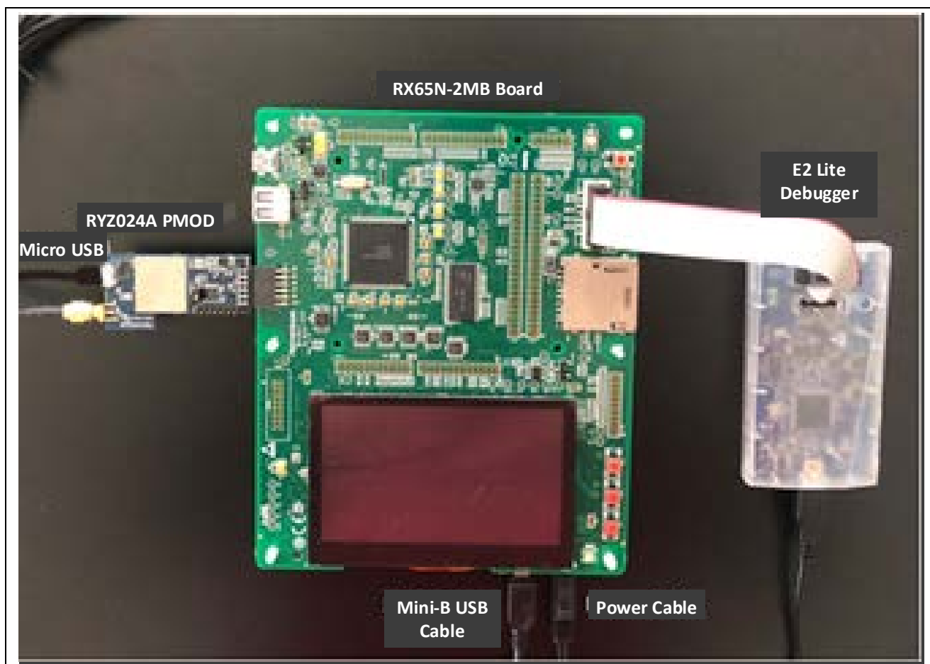
Figure 1. RSK-RX65N-2MB Setup with RYZ024A PMOD Board Connected
