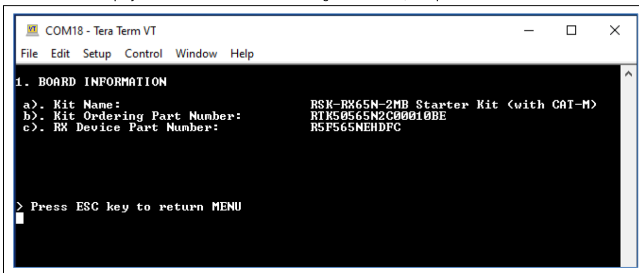
Figure 10. Board Information
