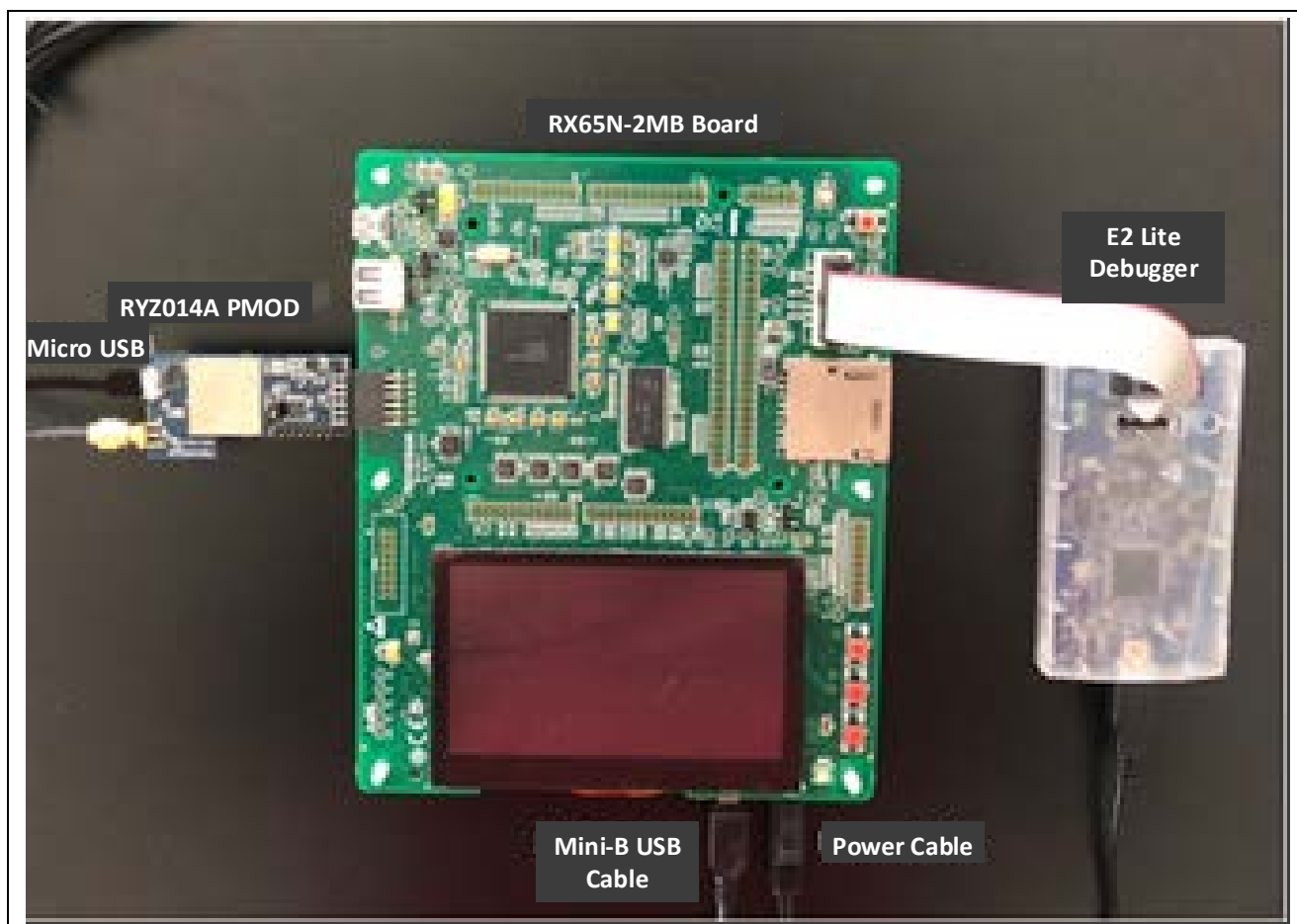
Figure 1. RSK-RX65N-2MB Setup with RYZ014A PMOD Board Connected
