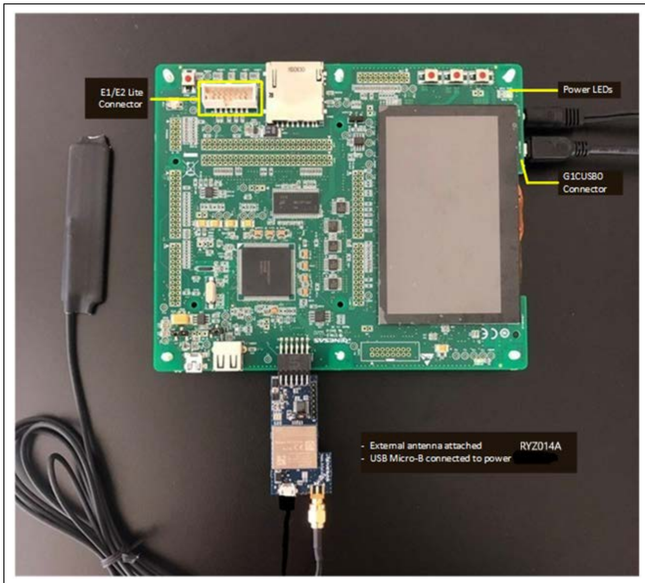
Figure 5. Connections to the RX65N-2MB Board After Flashing
